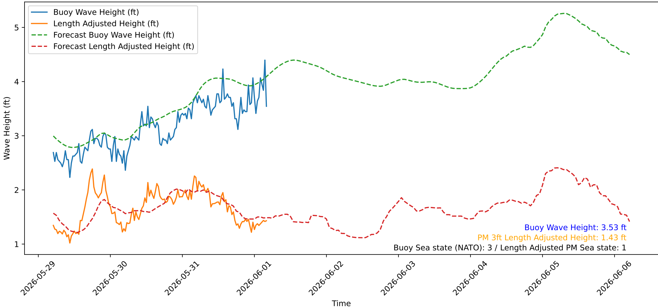
Wave Heights over Time for Oceanside Harbor at 2026-06-01 04:50:26
