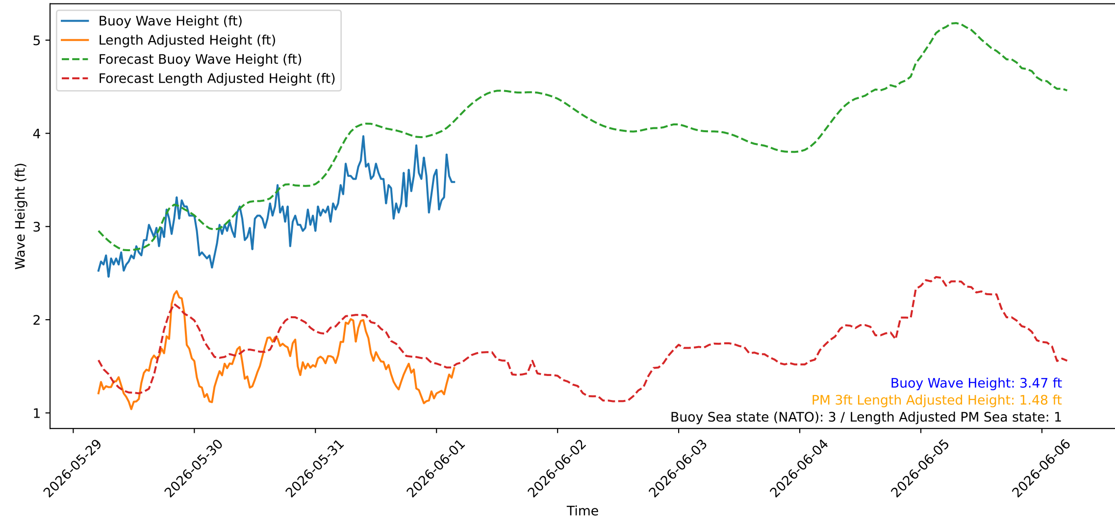
Wave Heights over Time for Green Beach at 2026-06-01 04:51:09
