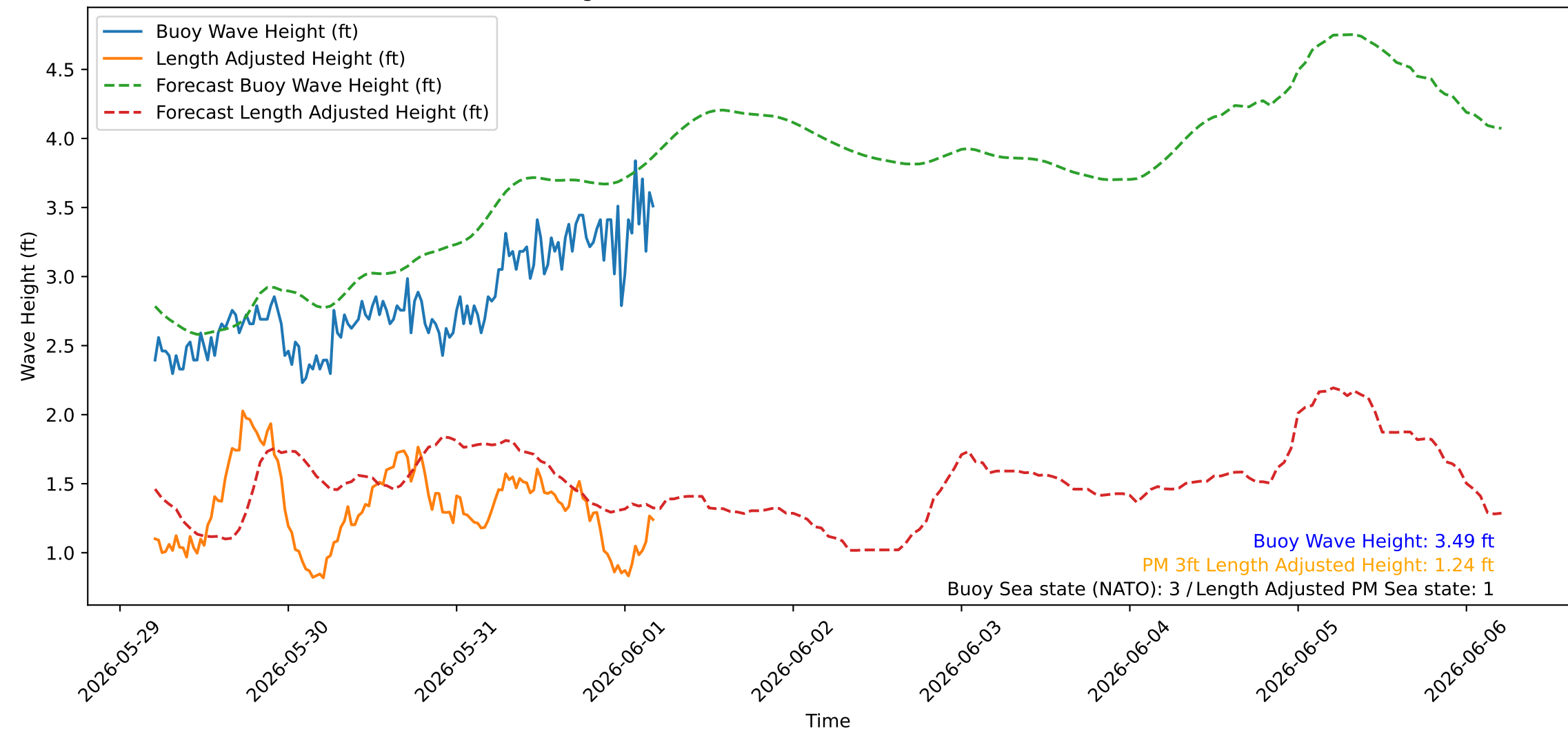
Wave Heights over Time for Red Beach at 2026-06-01 04:50:46
