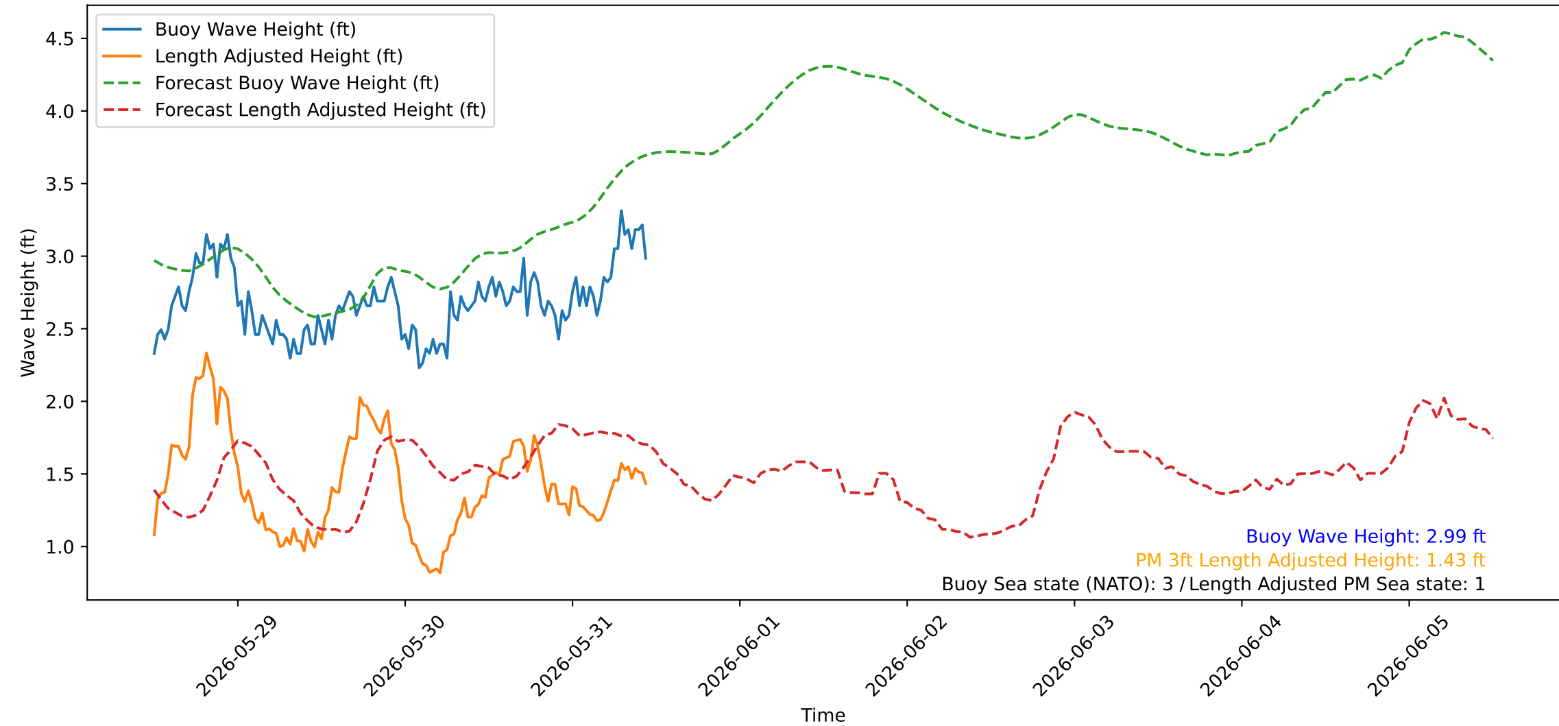
Wave Heights over Time for Red Beach at 2026-05-31 11:40:46
