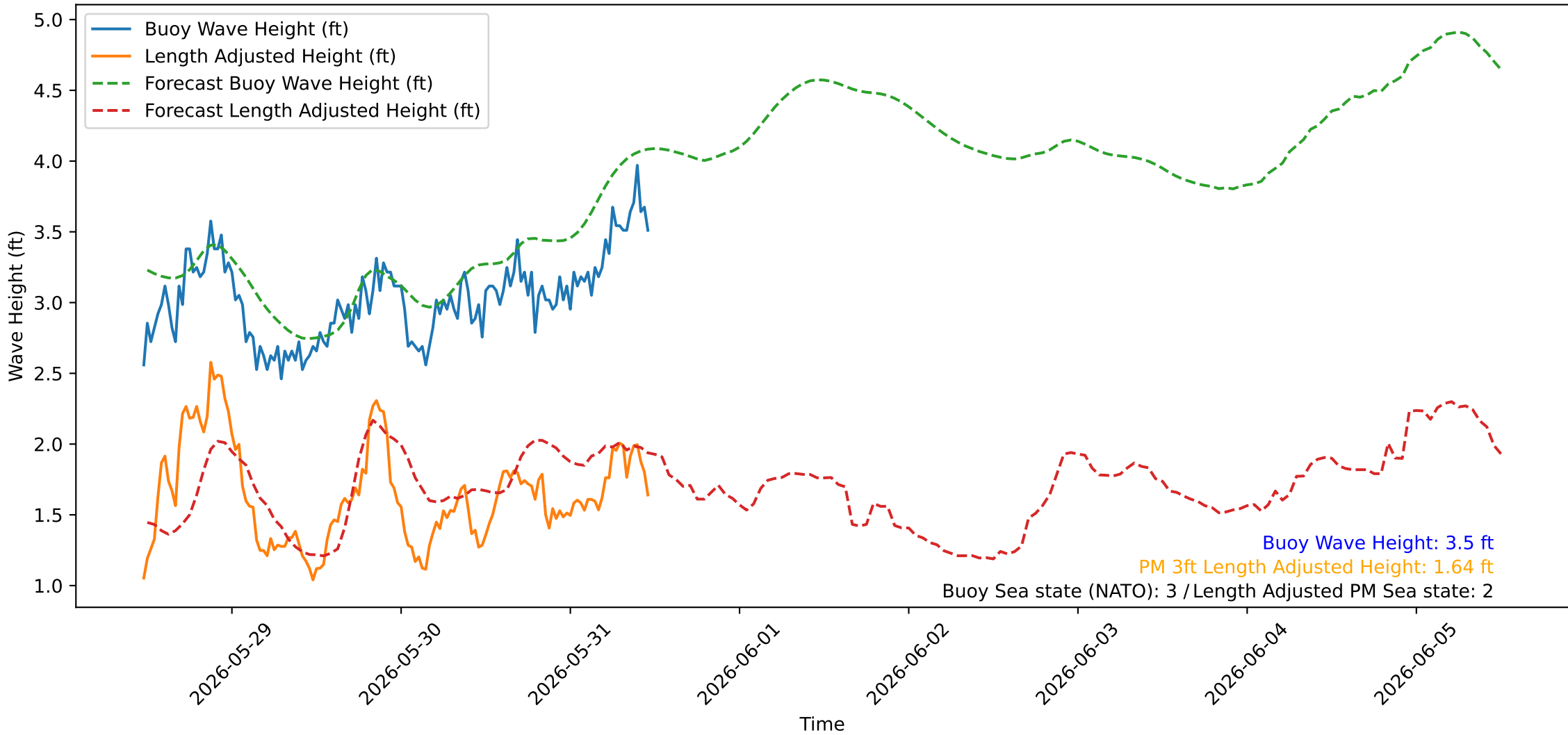
Wave Heights over Time for Green Beach at 2026-05-31 11:41:08
