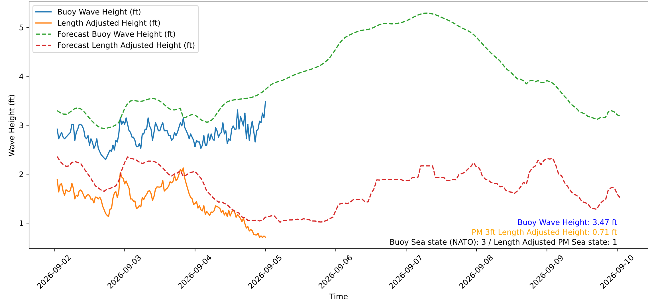
Wave Heights over Time for Red Beach at 2026-09-05 00:50:50
