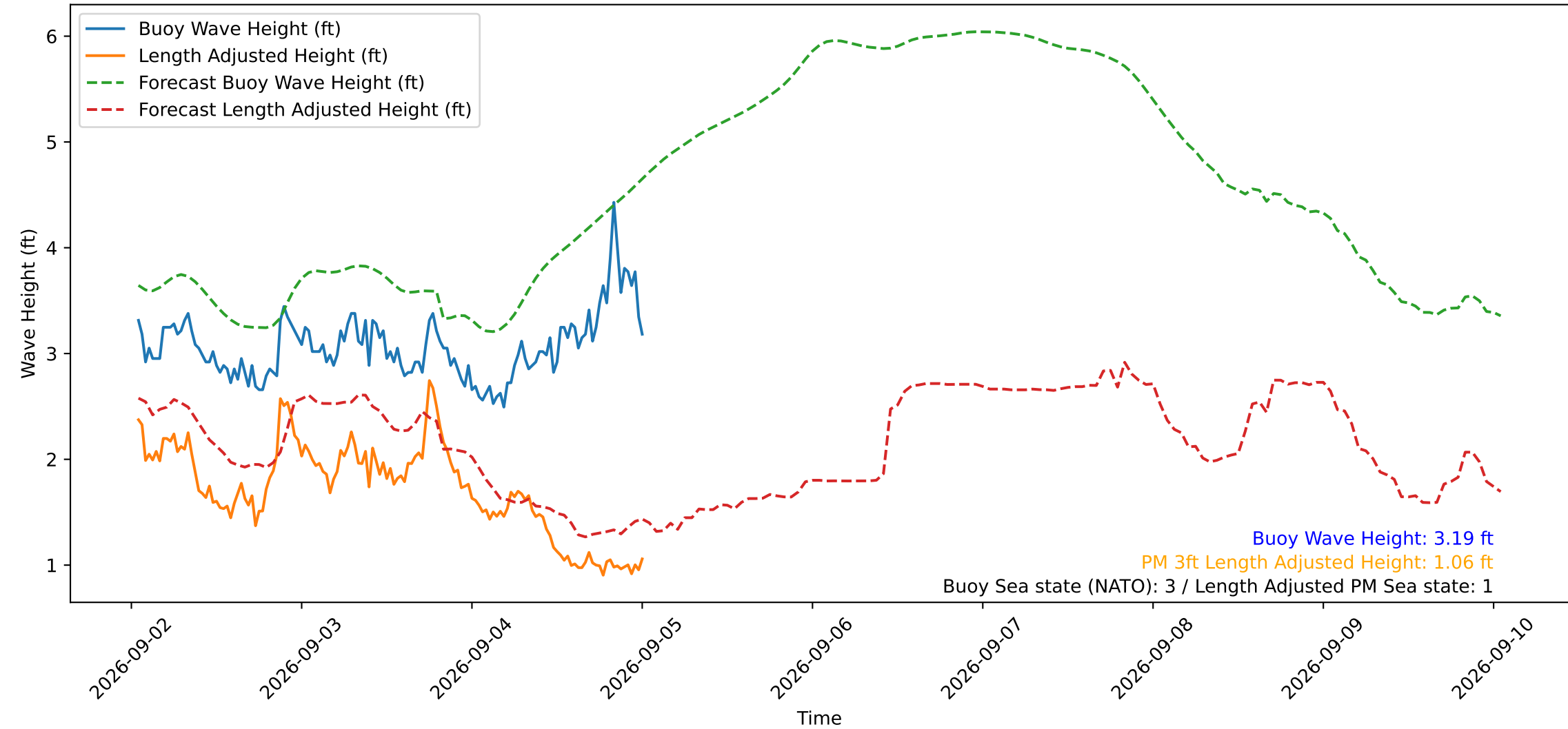
Wave Heights over Time for Green Beach at 2026-09-05 00:51:15
