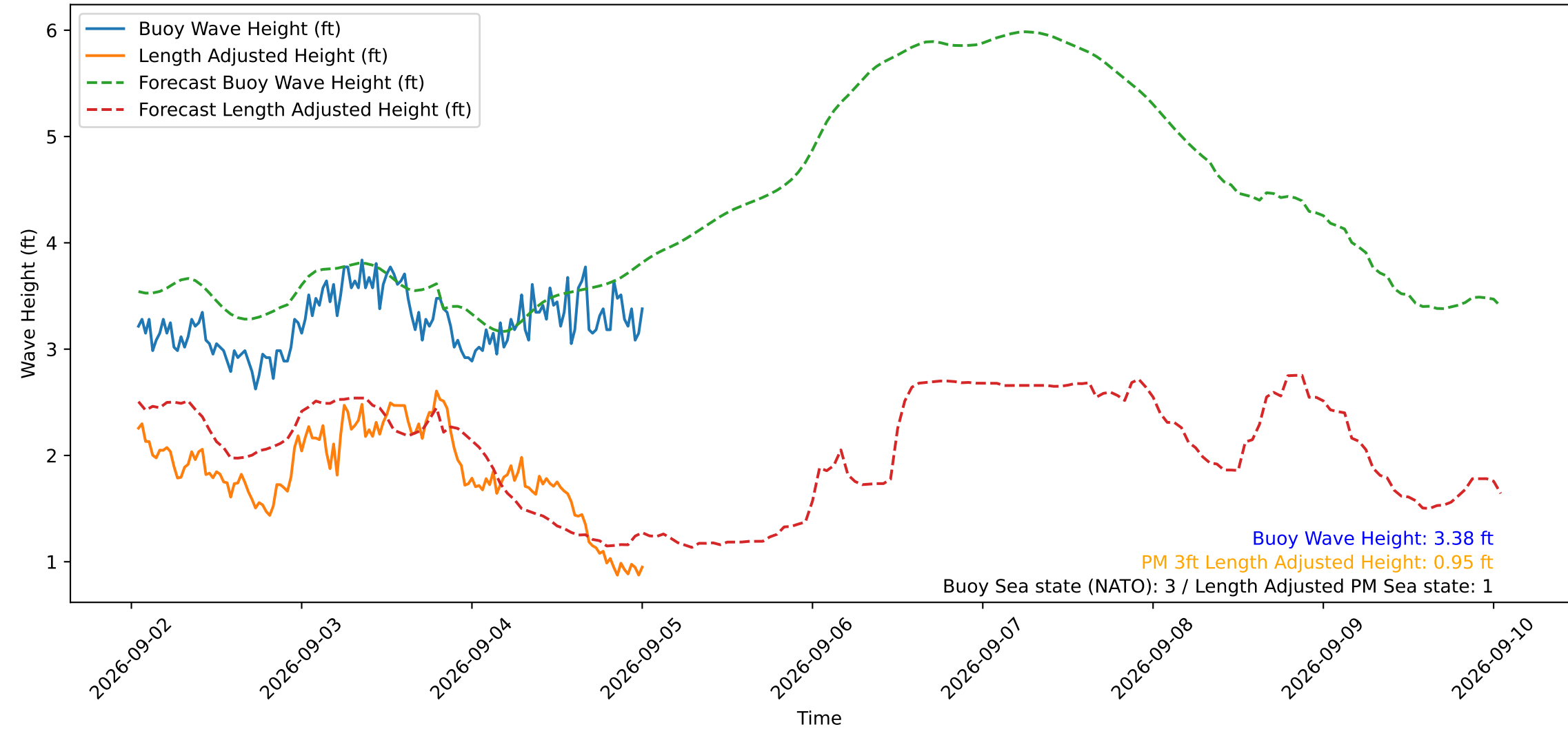
Wave Heights over Time for Oceanside Harbor at 2026-09-05 00:50:29
