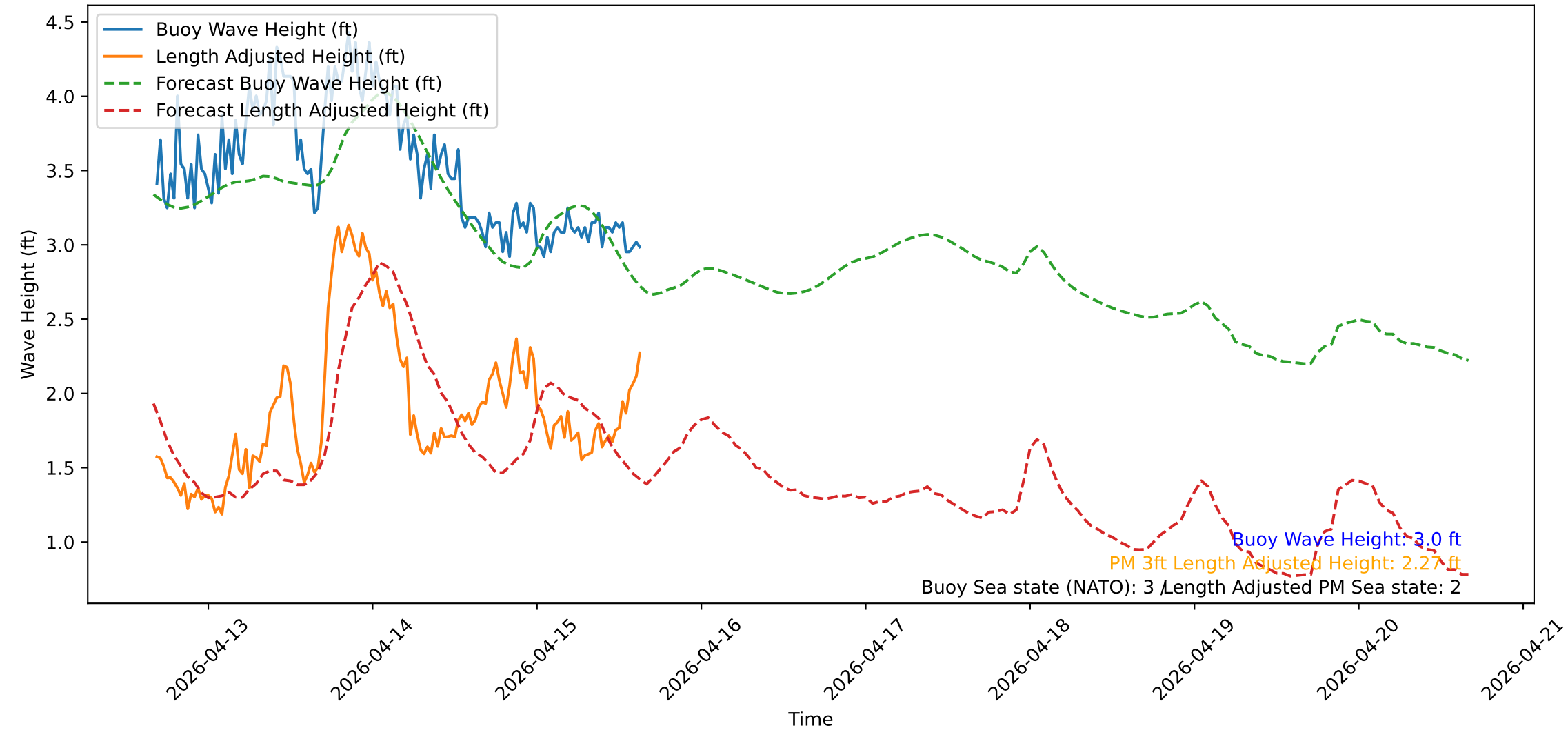
Wave Heights over Time for Red Beach at 2026-04-15 16:00:50
