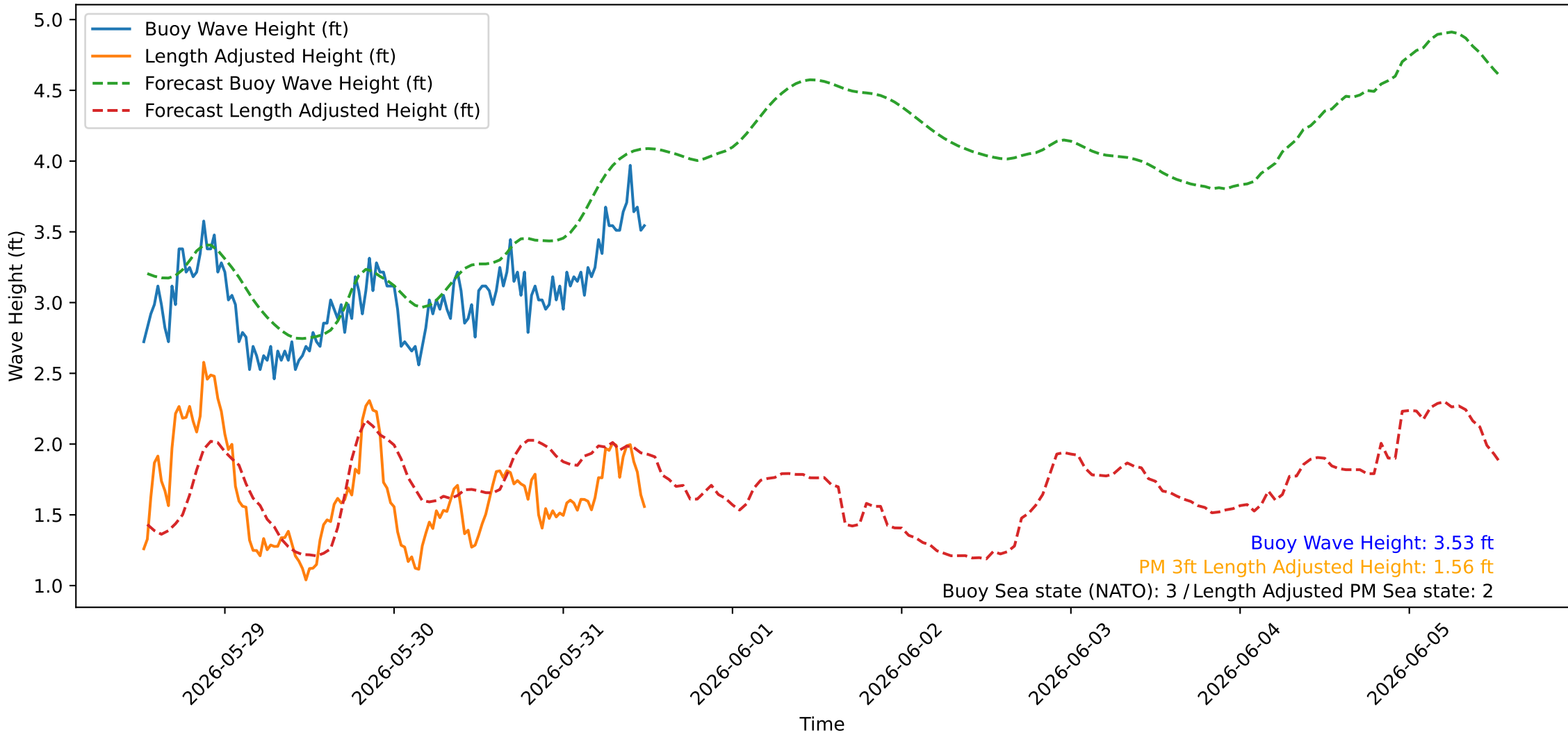
Wave Heights over Time for Green Beach at 2026-05-31 12:31:08
