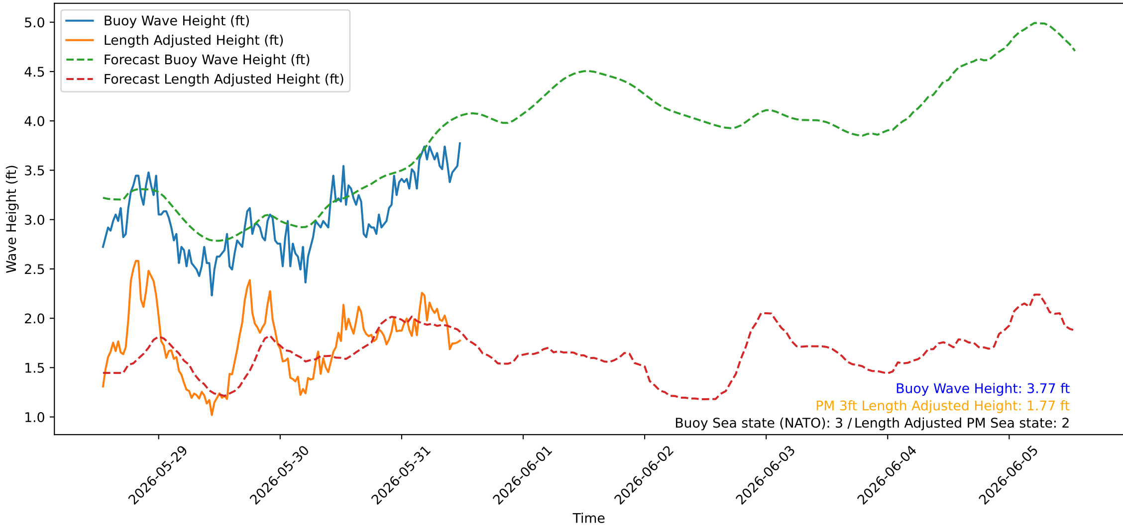
Wave Heights over Time for Oceanside Harbor at 2026-05-31 12:30:27
