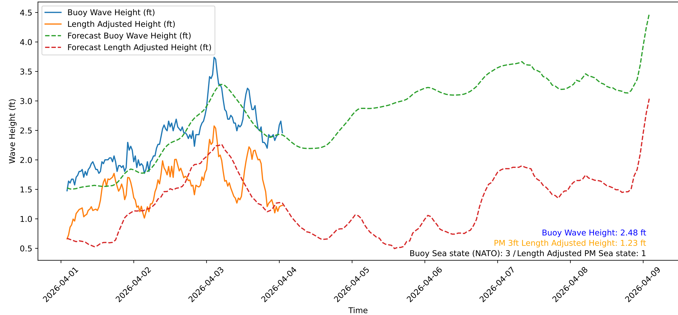
Wave Heights over Time for Red Beach at 2026-04-04 01:40:47
