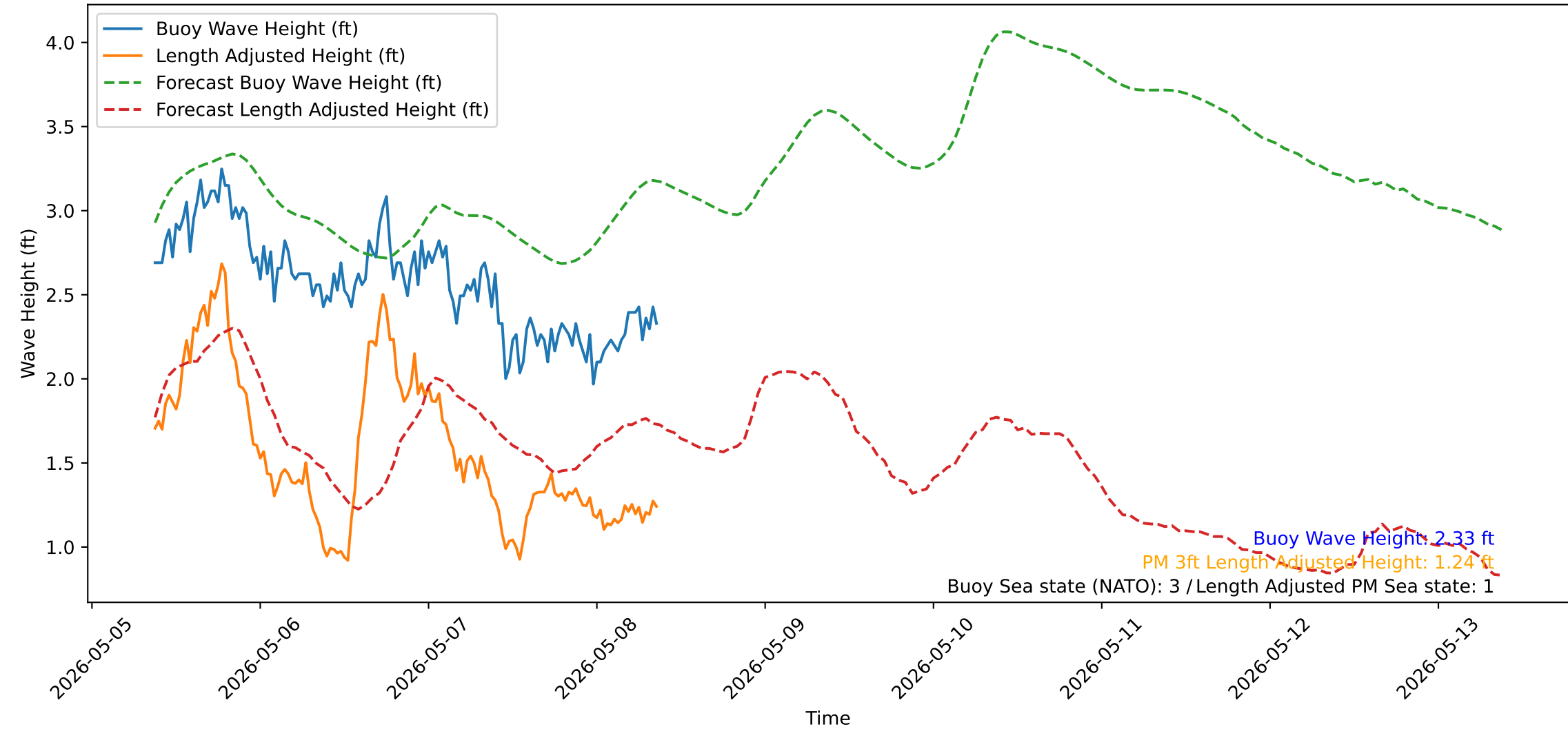
Wave Heights over Time for Oceanside Harbor at 2026-05-08 09:00:31
