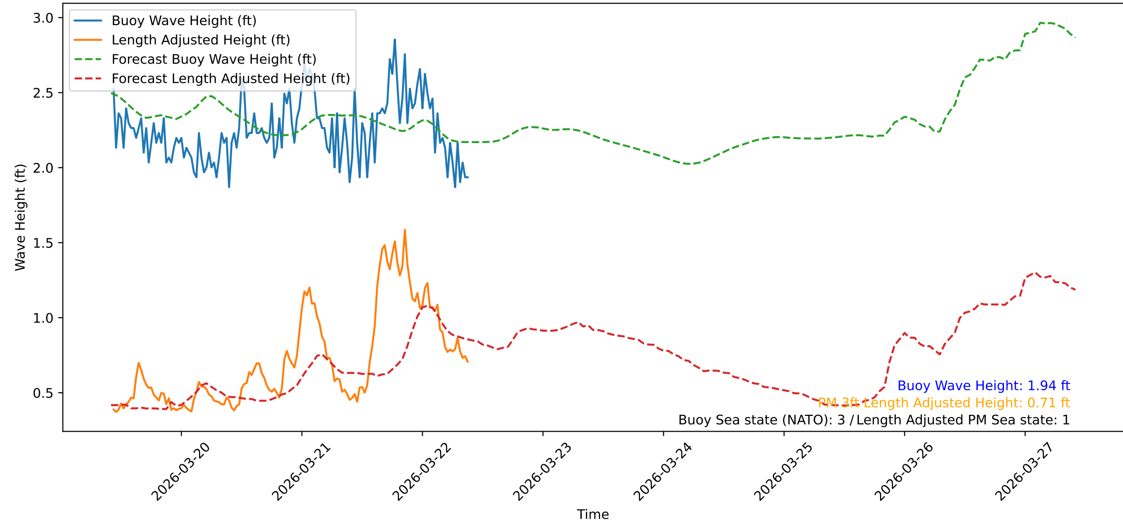
Wave Heights over Time for Red Beach at 2026-03-22 10:00:48
