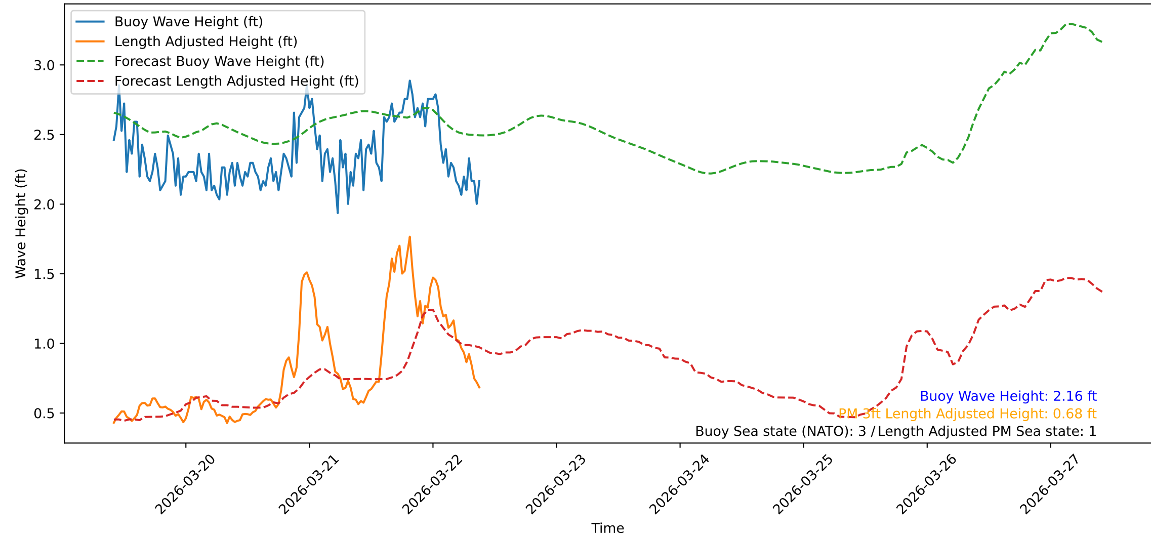
Wave Heights over Time for Green Beach at 2026-03-22 10:01:11
