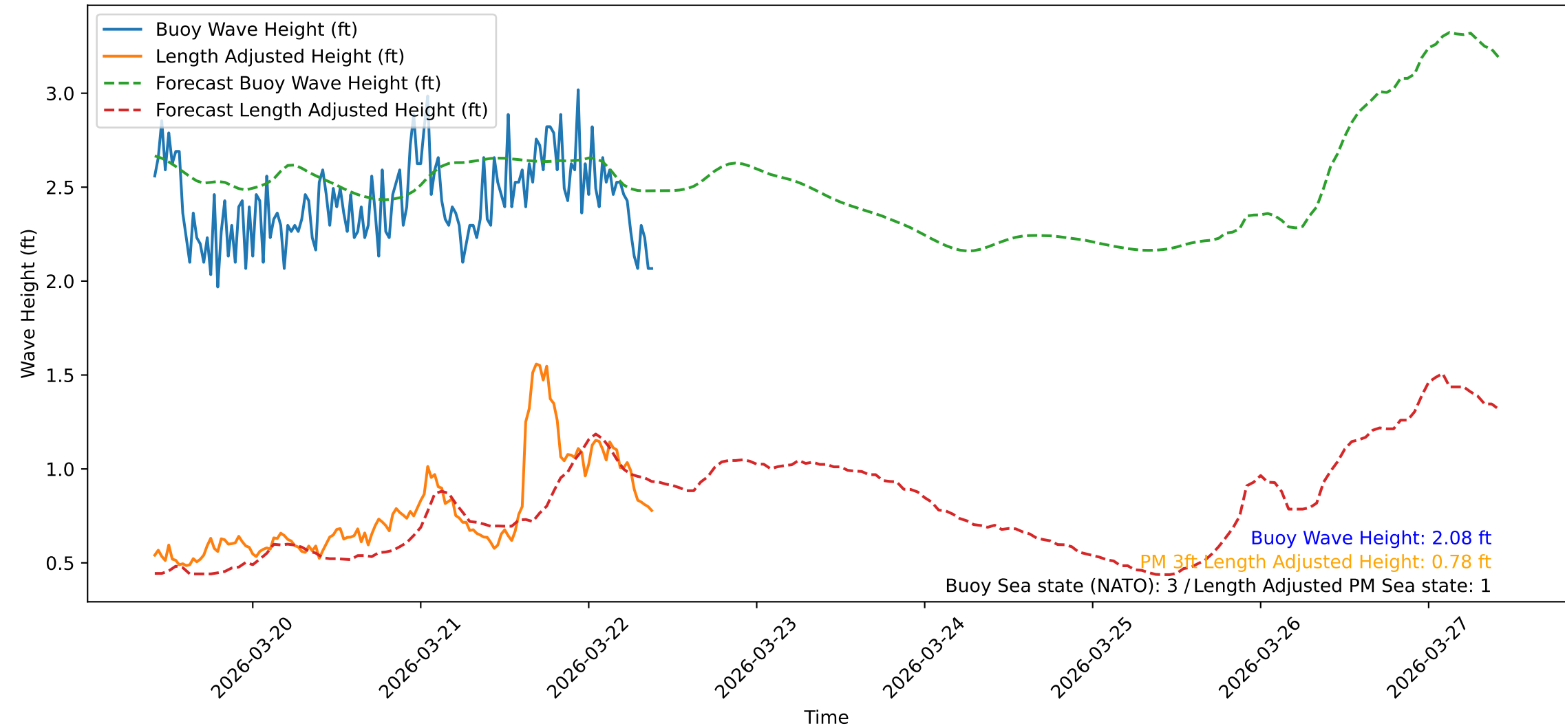
Wave Heights over Time for Oceanside Harbor at 2026-03-22 10:00:32
