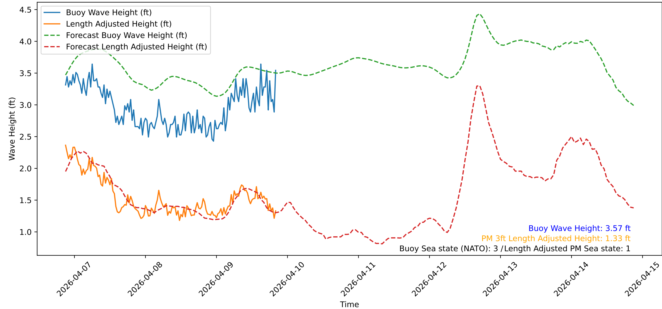
Wave Heights over Time for Oceanside Harbor at 2026-04-09 20:50:30
