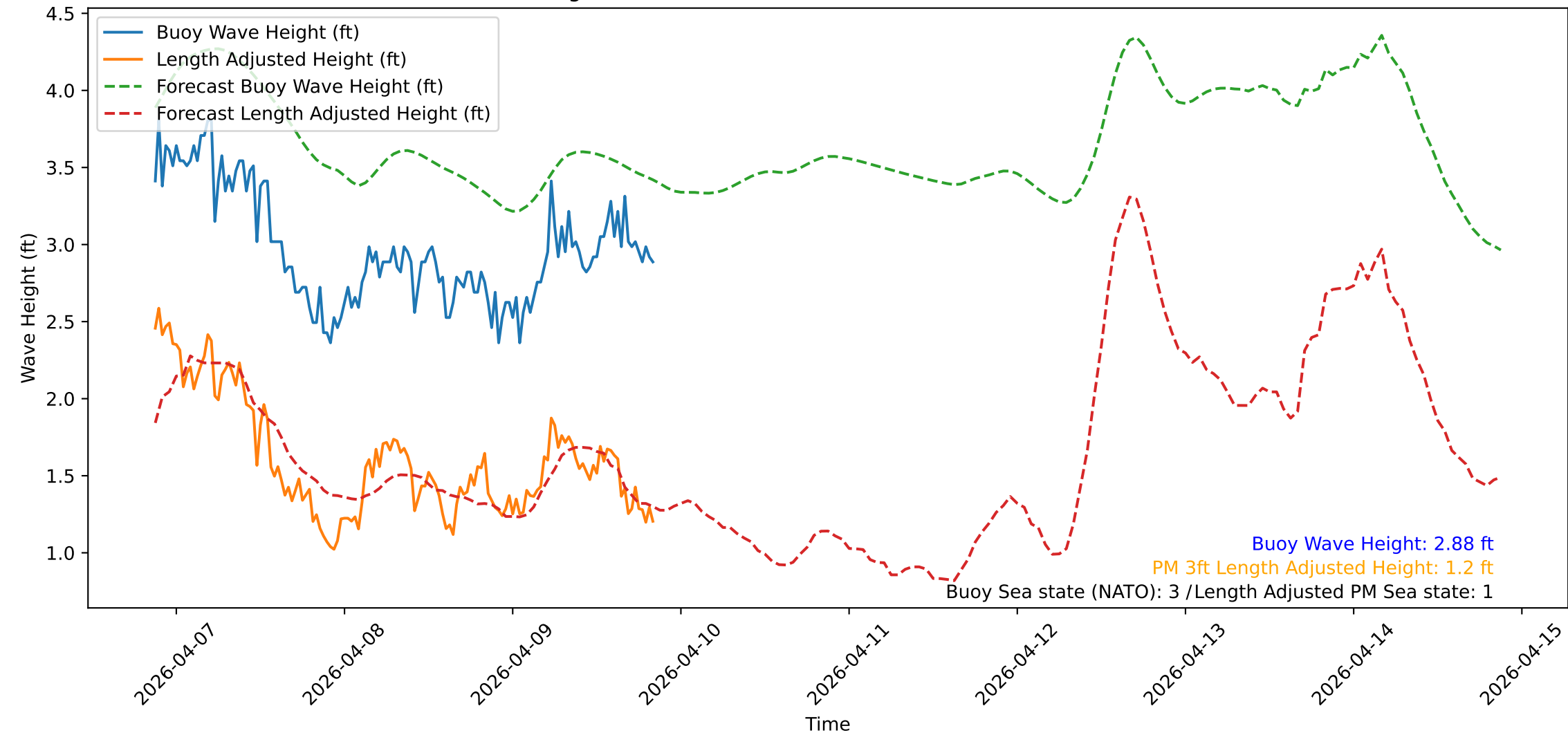
Wave Heights over Time for Green Beach at 2026-04-09 20:51:09
