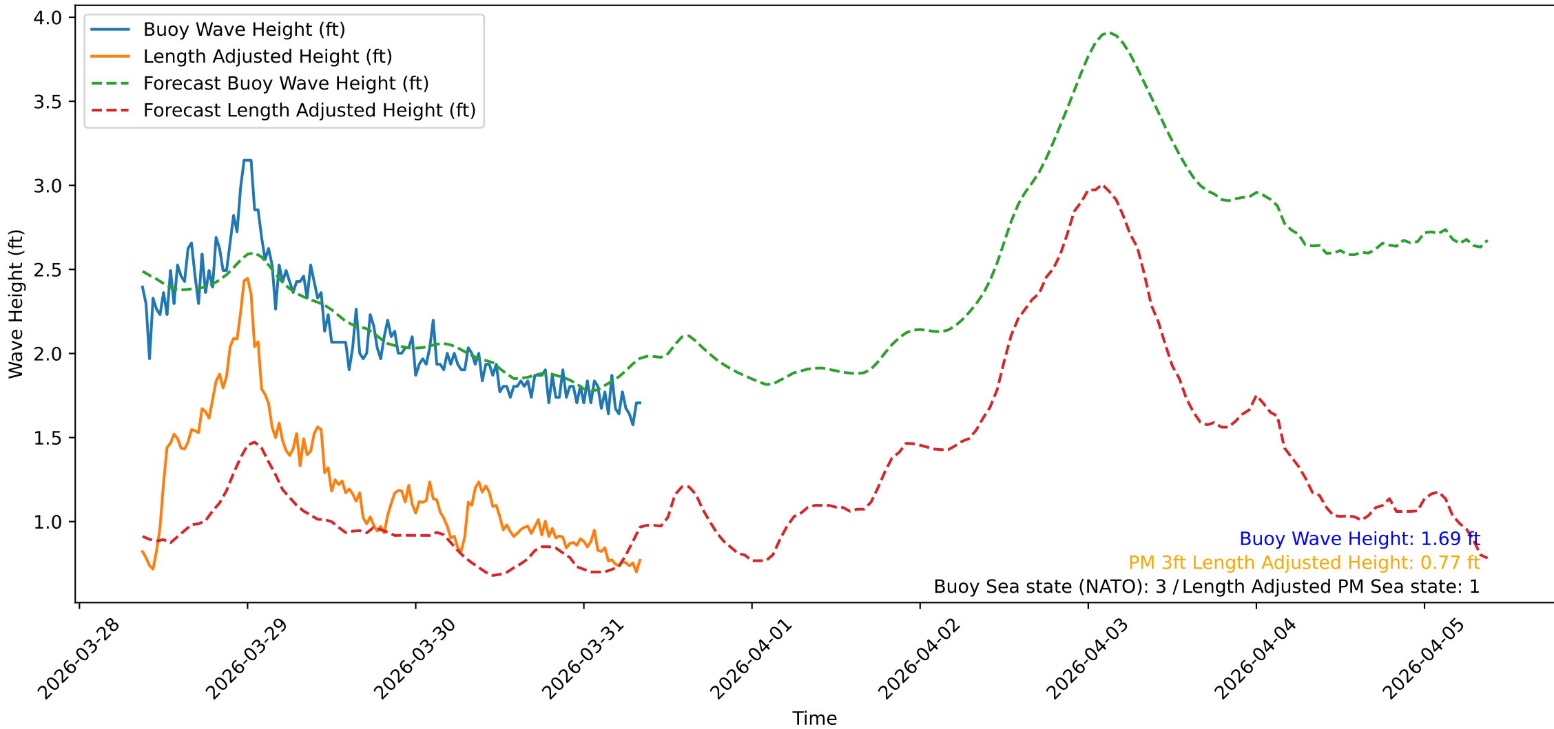
Wave Heights over Time for Oceanside Harbor at 2026-03-31 09:00:31
