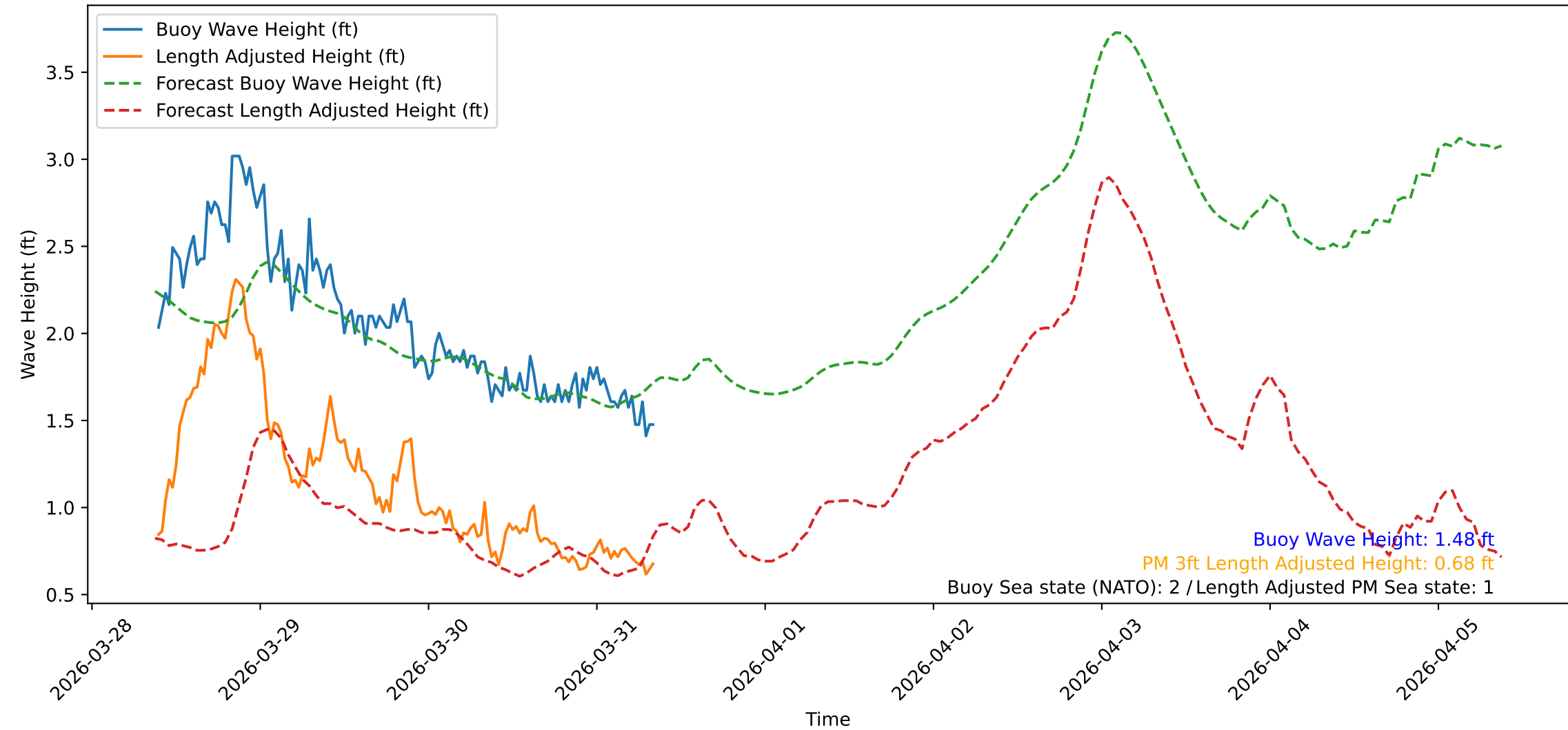
Wave Heights over Time for Red Beach at 2026-03-31 09:00:47
