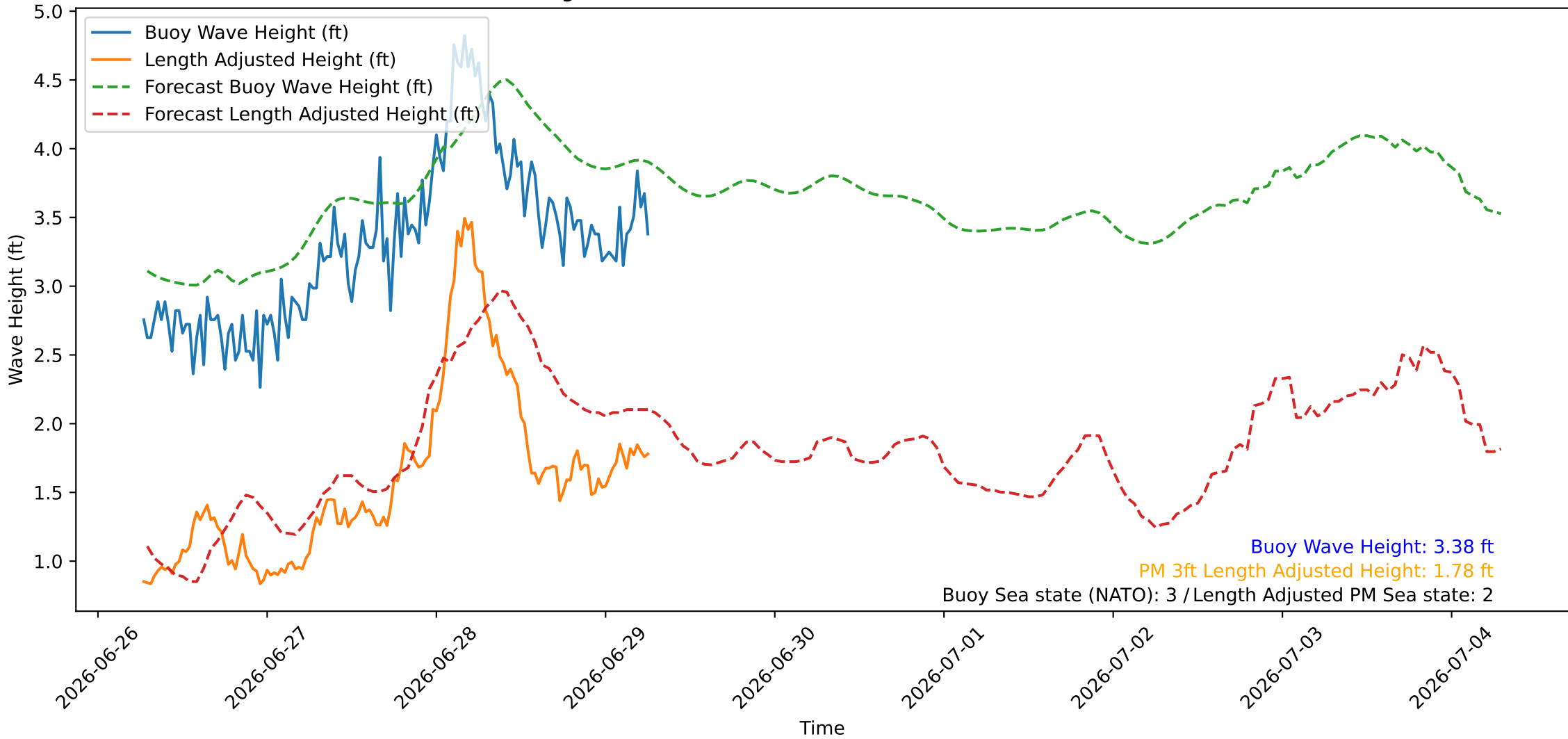
Wave Heights over Time for Green Beach at 2026-06-29 06:41:08
