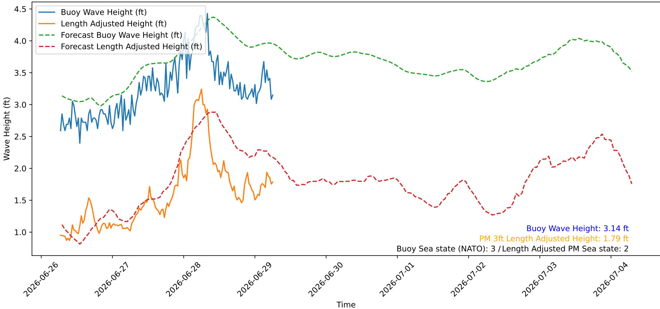
Wave Heights over Time for Oceanside Harbor at 2026-06-29 06:40:26
