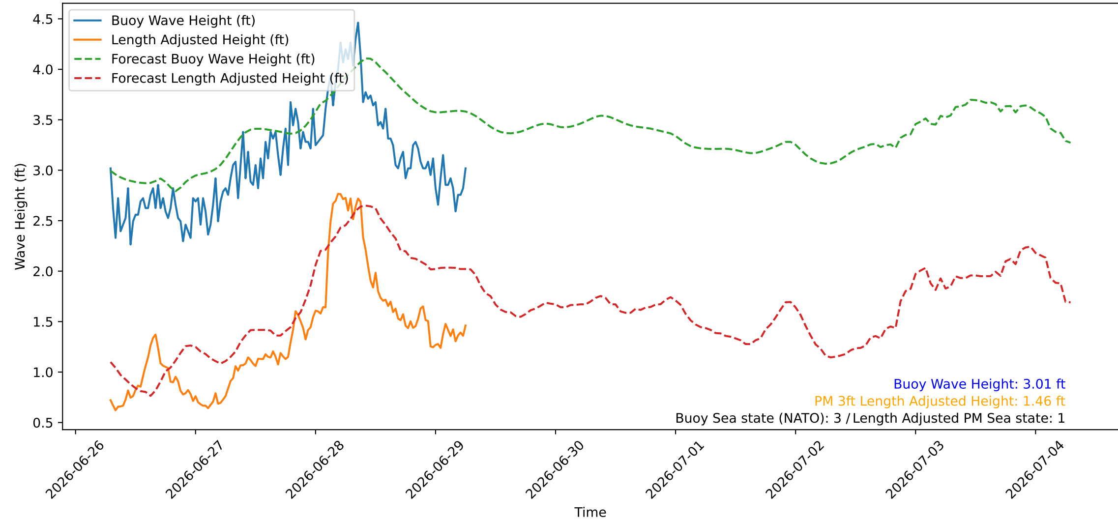
Wave Heights over Time for Red Beach at 2026-06-29 06:40:46
