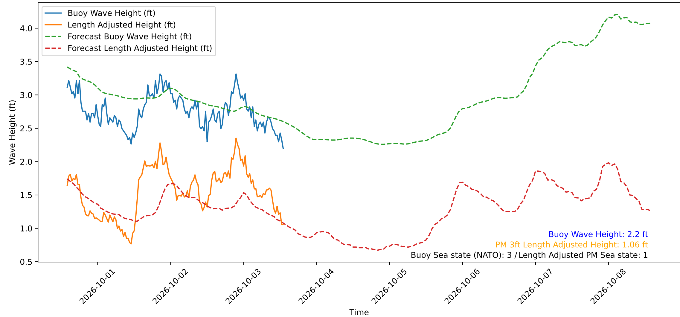
Wave Heights over Time for Oceanside Harbor at 2026-10-03 13:50:30
