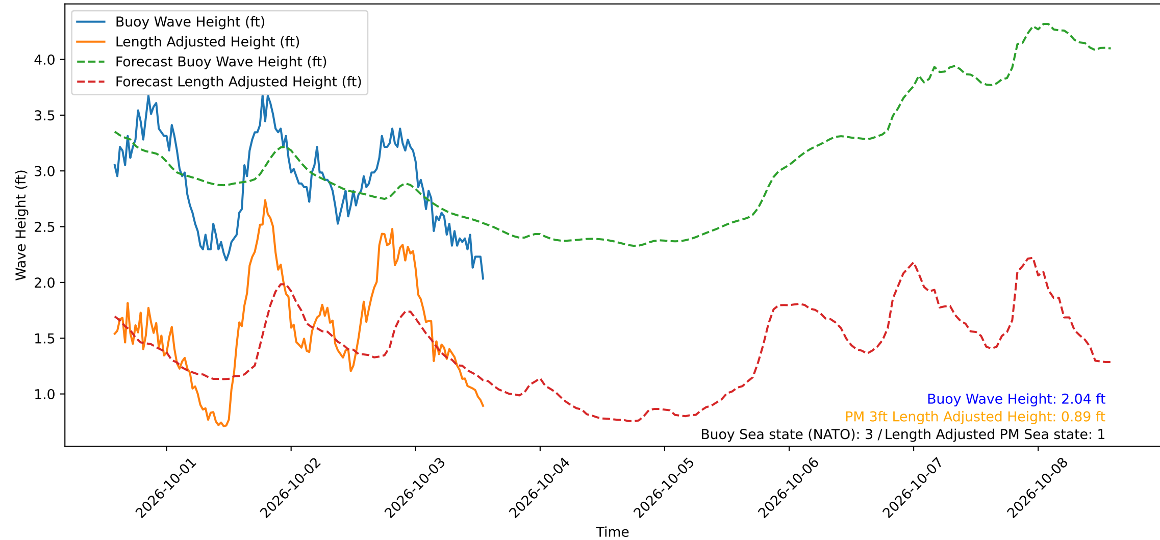
Wave Heights over Time for Green Beach at 2026-10-03 13:51:15
