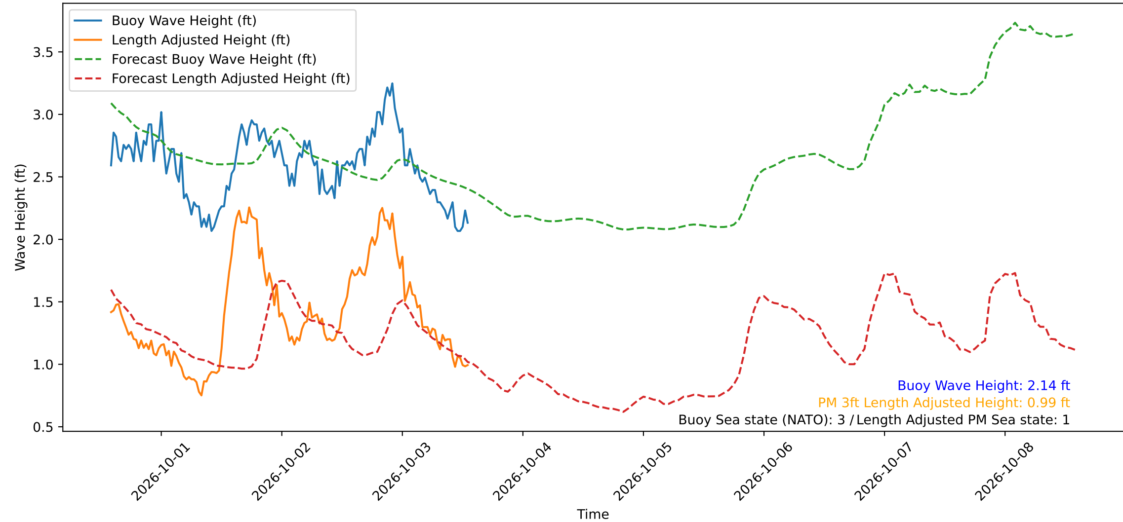
Wave Heights over Time for Red Beach at 2026-10-03 13:50:51
