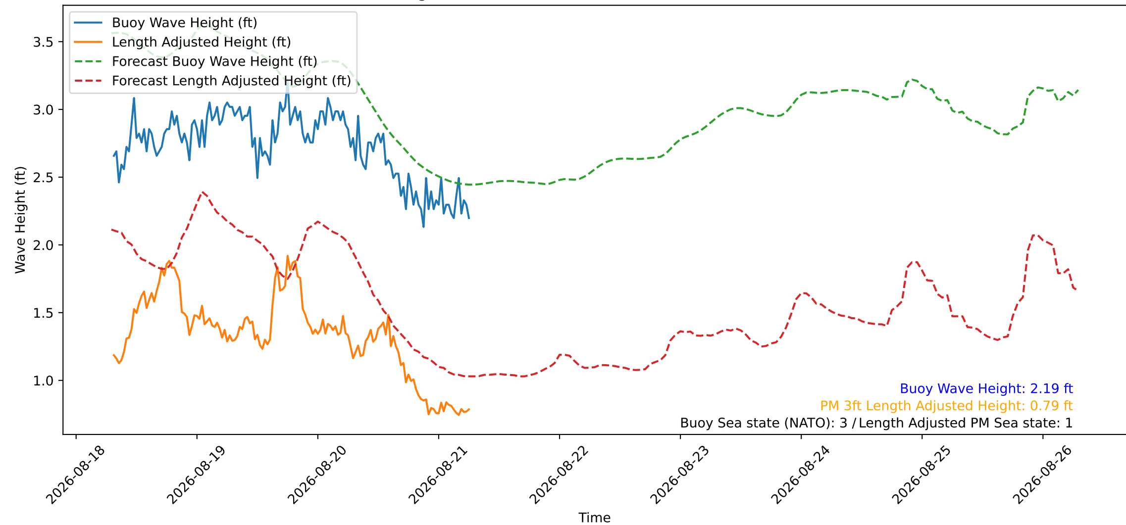
Wave Heights over Time for Red Beach at 2026-08-21 07:00:45
