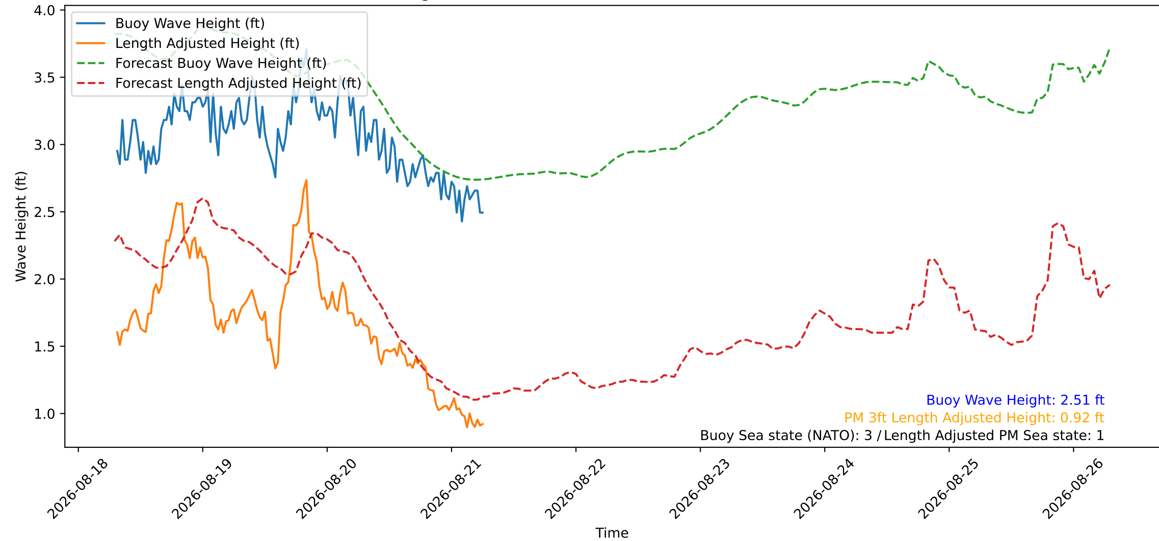
Wave Heights over Time for Green Beach at 2026-08-21 07:01:07
