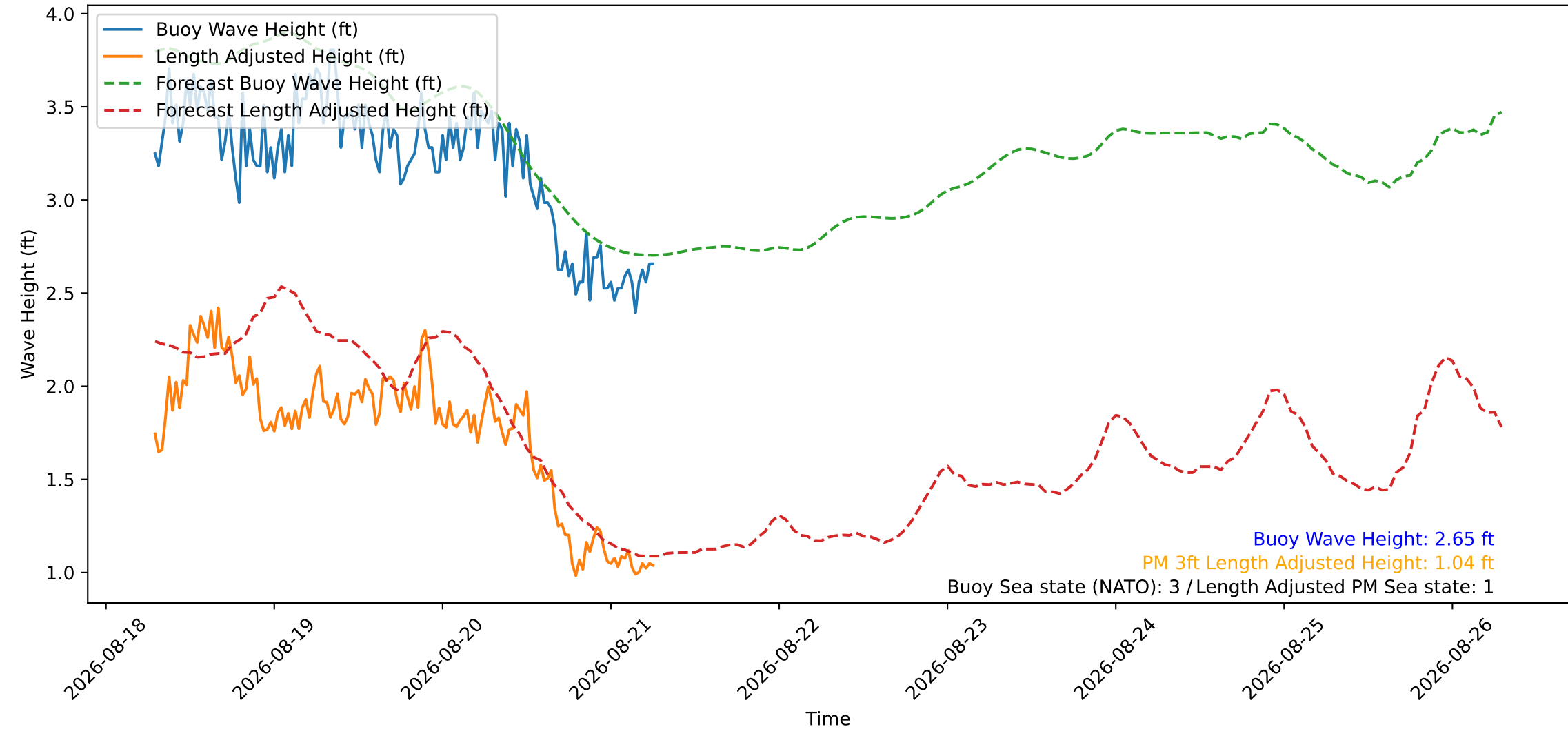
Wave Heights over Time for Oceanside Harbor at 2026-08-21 07:00:26
