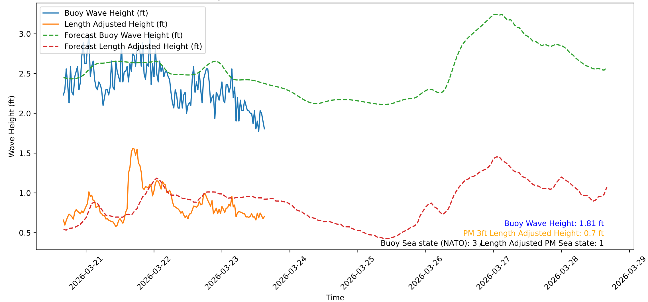
Wave Heights over Time for Oceanside Harbor at 2026-03-23 16:00:31
