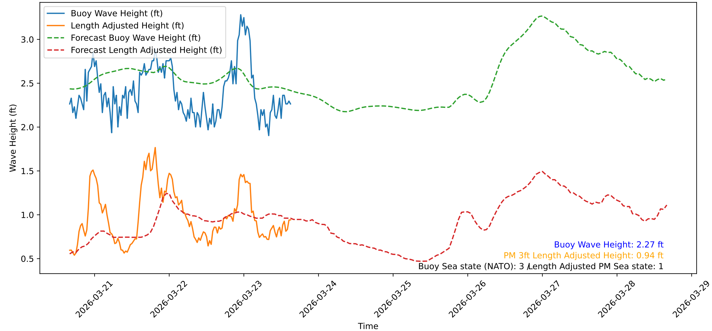
Wave Heights over Time for Green Beach at 2026-03-23 16:01:10
