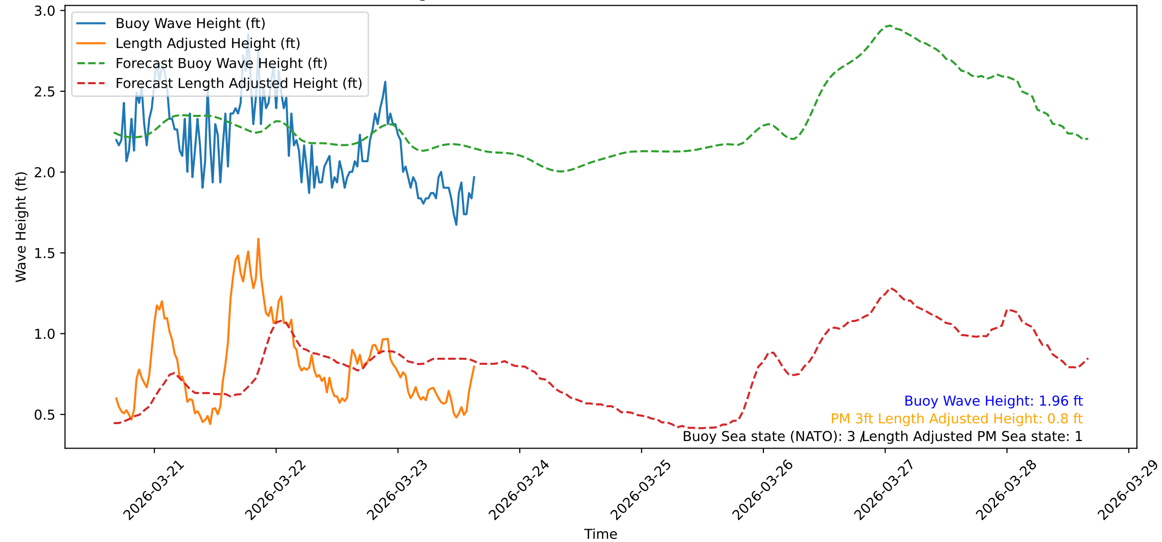
Wave Heights over Time for Red Beach at 2026-03-23 16:00:48
