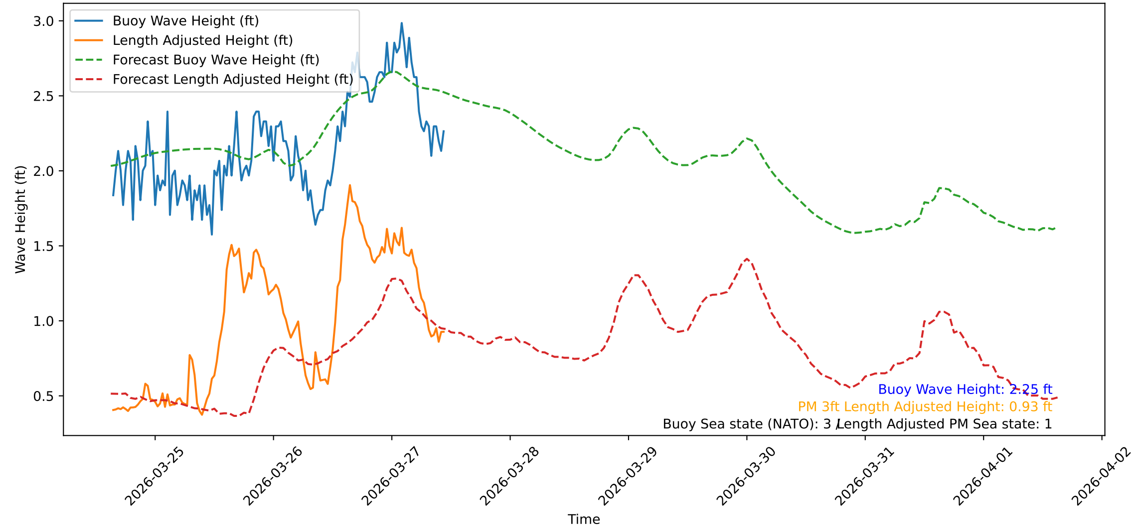
Wave Heights over Time for Red Beach at 2026-03-27 15:00:46
