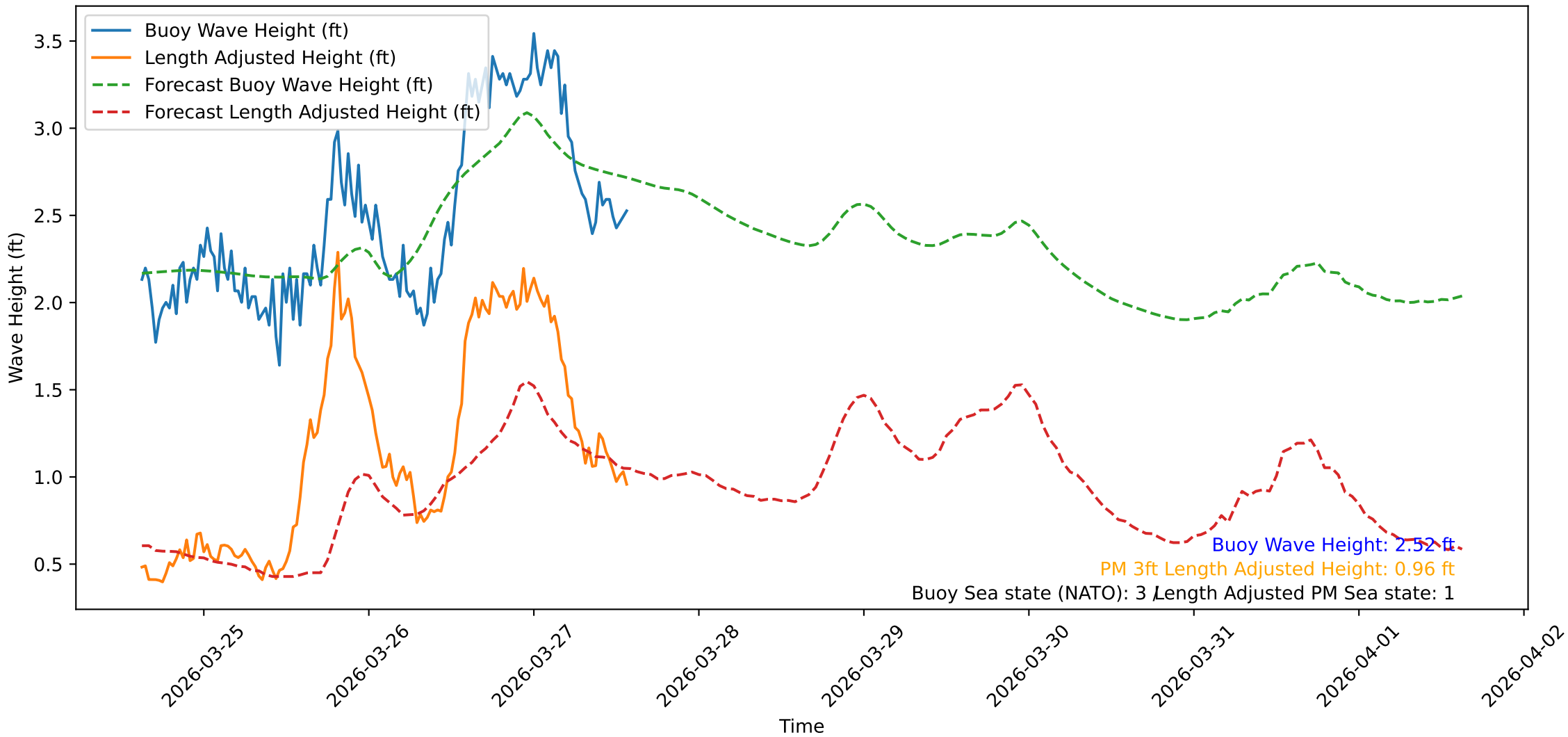
Wave Heights over Time for Green Beach at 2026-03-27 15:01:08
