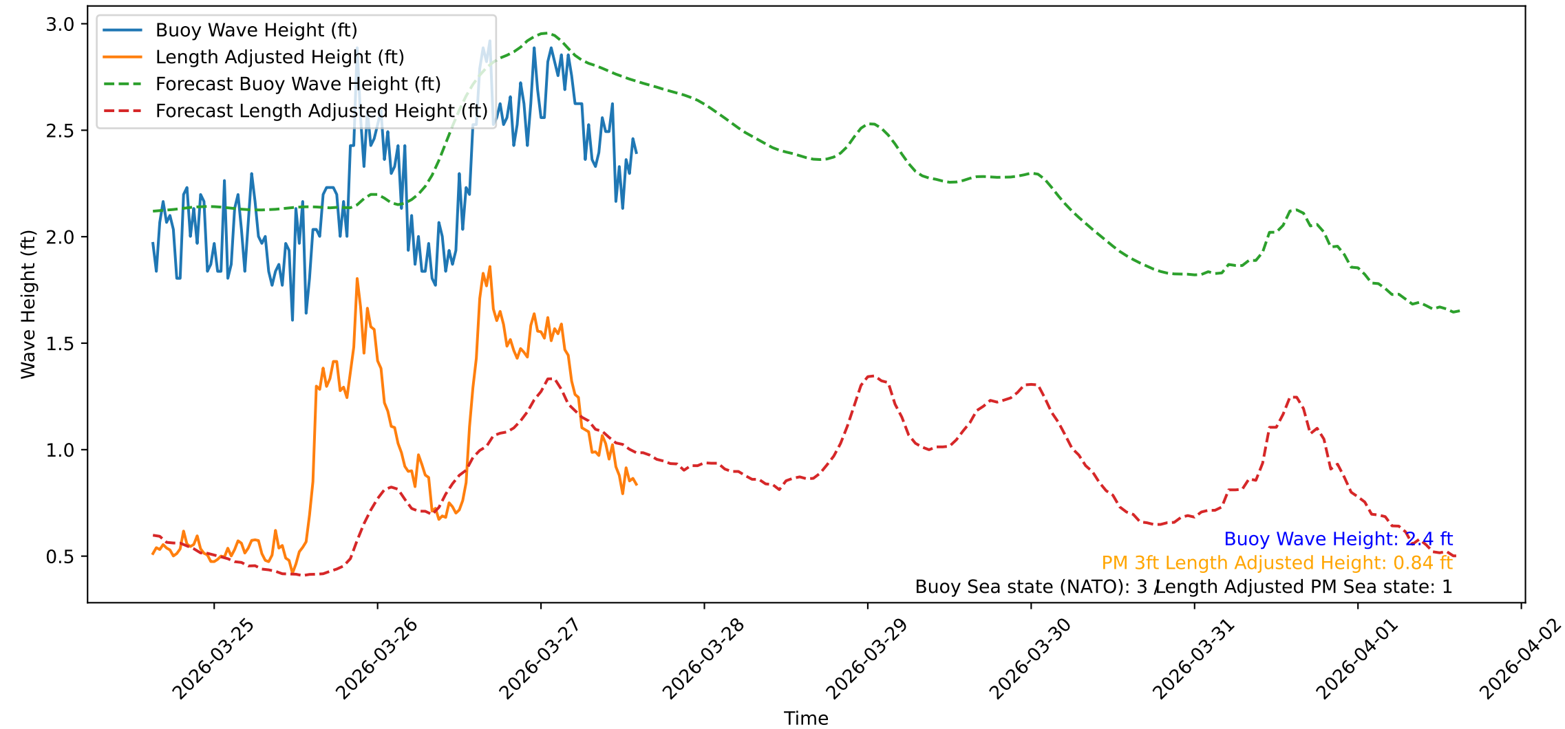
Wave Heights over Time for Oceanside Harbor at 2026-03-27 15:00:31
