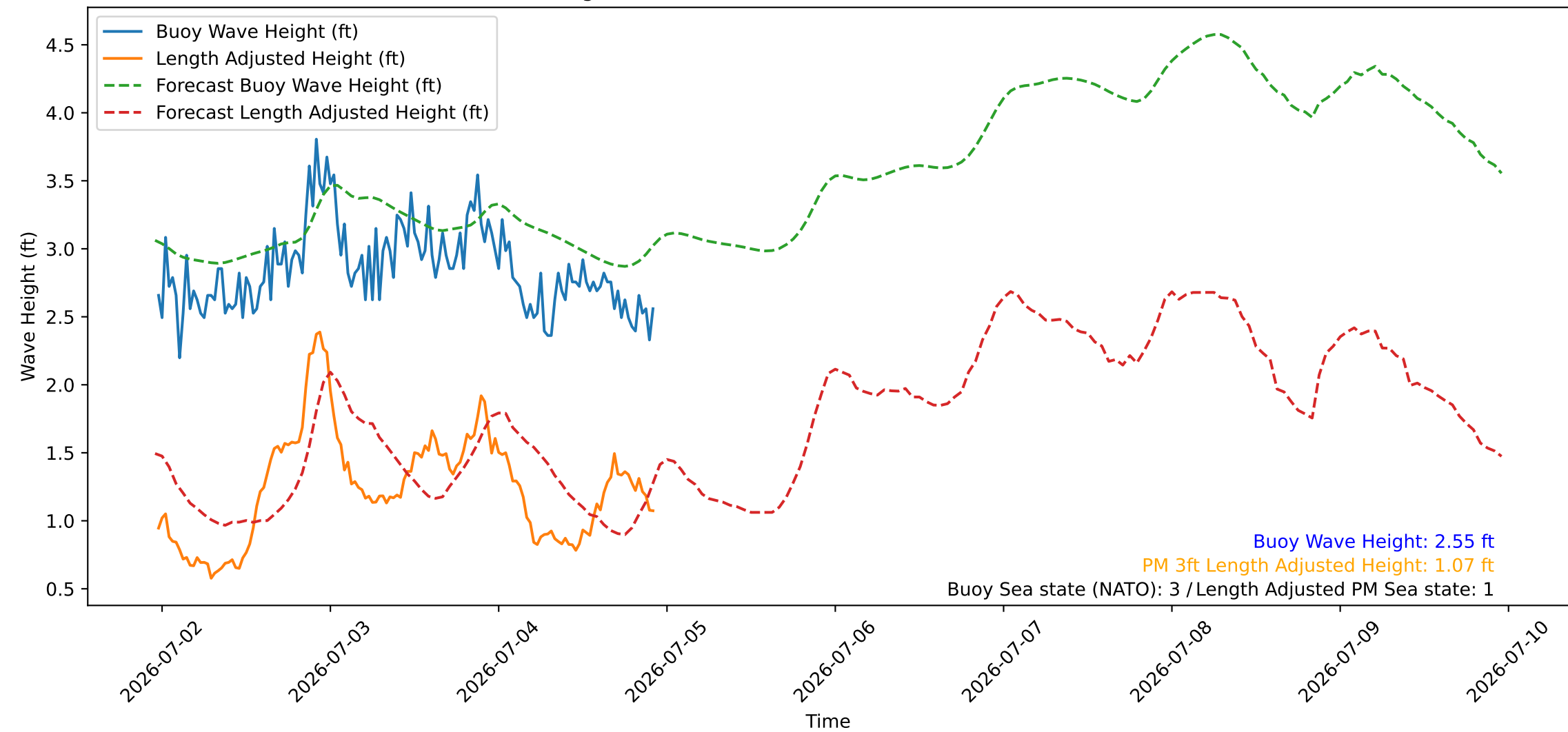
Wave Heights over Time for Red Beach at 2026-07-04 23:00:45
