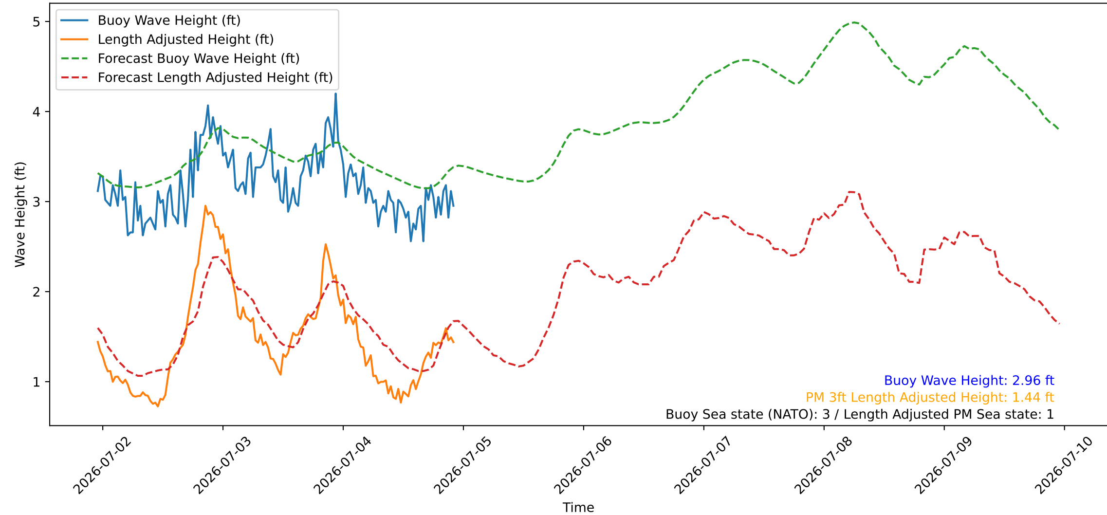
Wave Heights over Time for Green Beach at 2026-07-04 23:01:08
