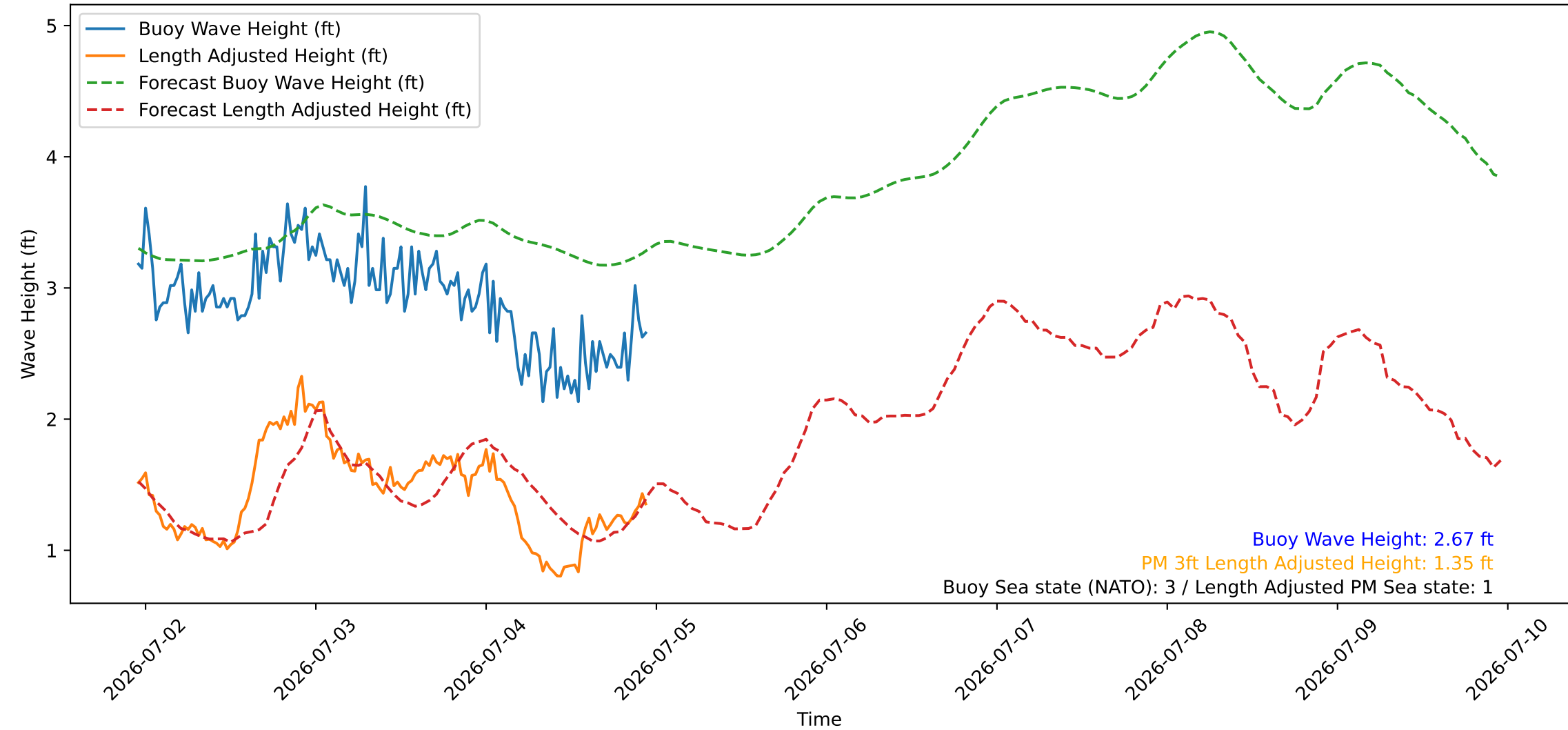
Wave Heights over Time for Oceanside Harbor at 2026-07-04 23:00:26
