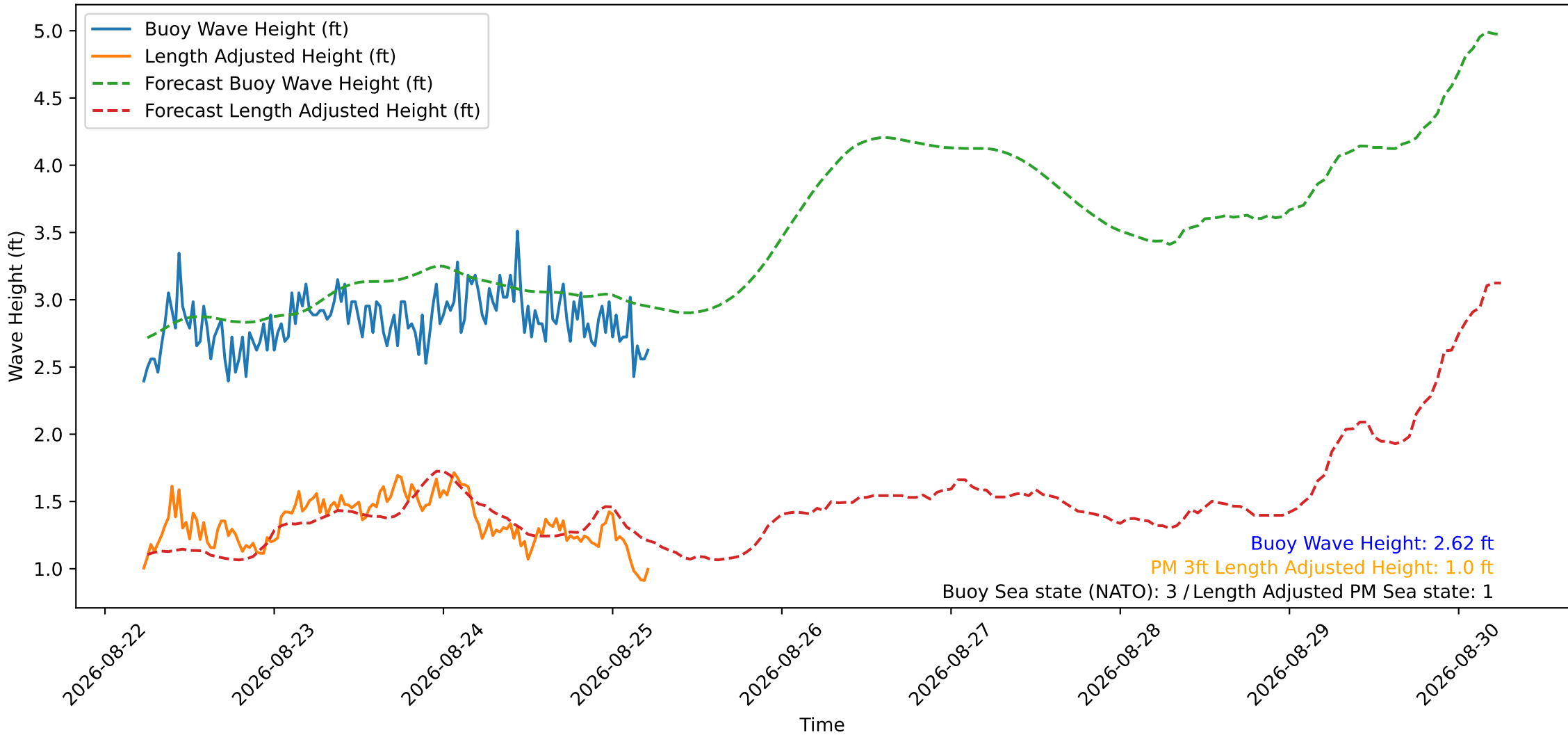
Wave Heights over Time for Oceanside Harbor at 2026-08-25 05:40:29
