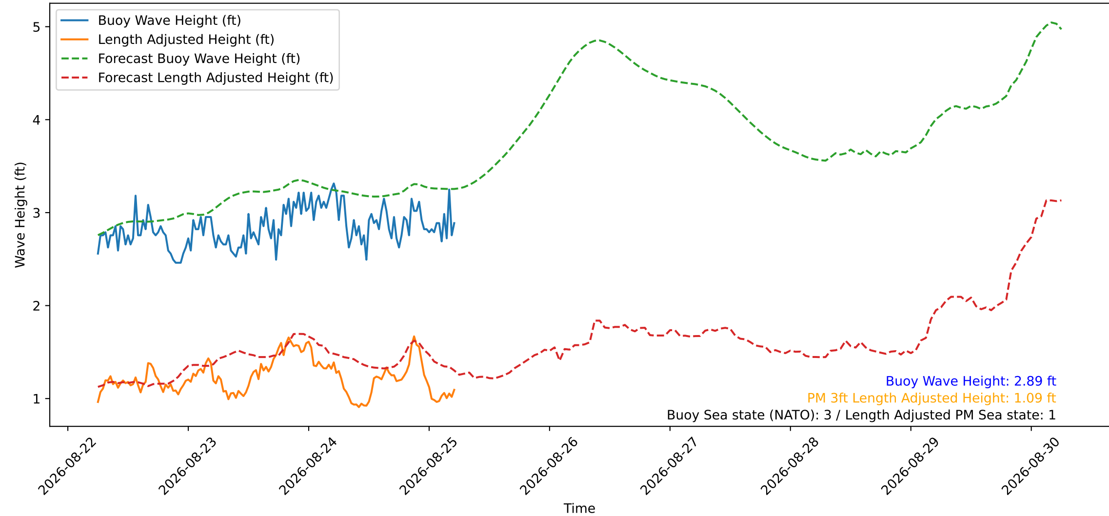
Wave Heights over Time for Green Beach at 2026-08-25 05:41:11
