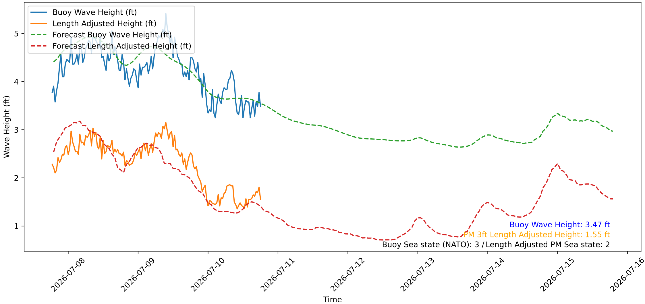
Wave Heights over Time for Oceanside Harbor at 2026-07-10 18:40:26
