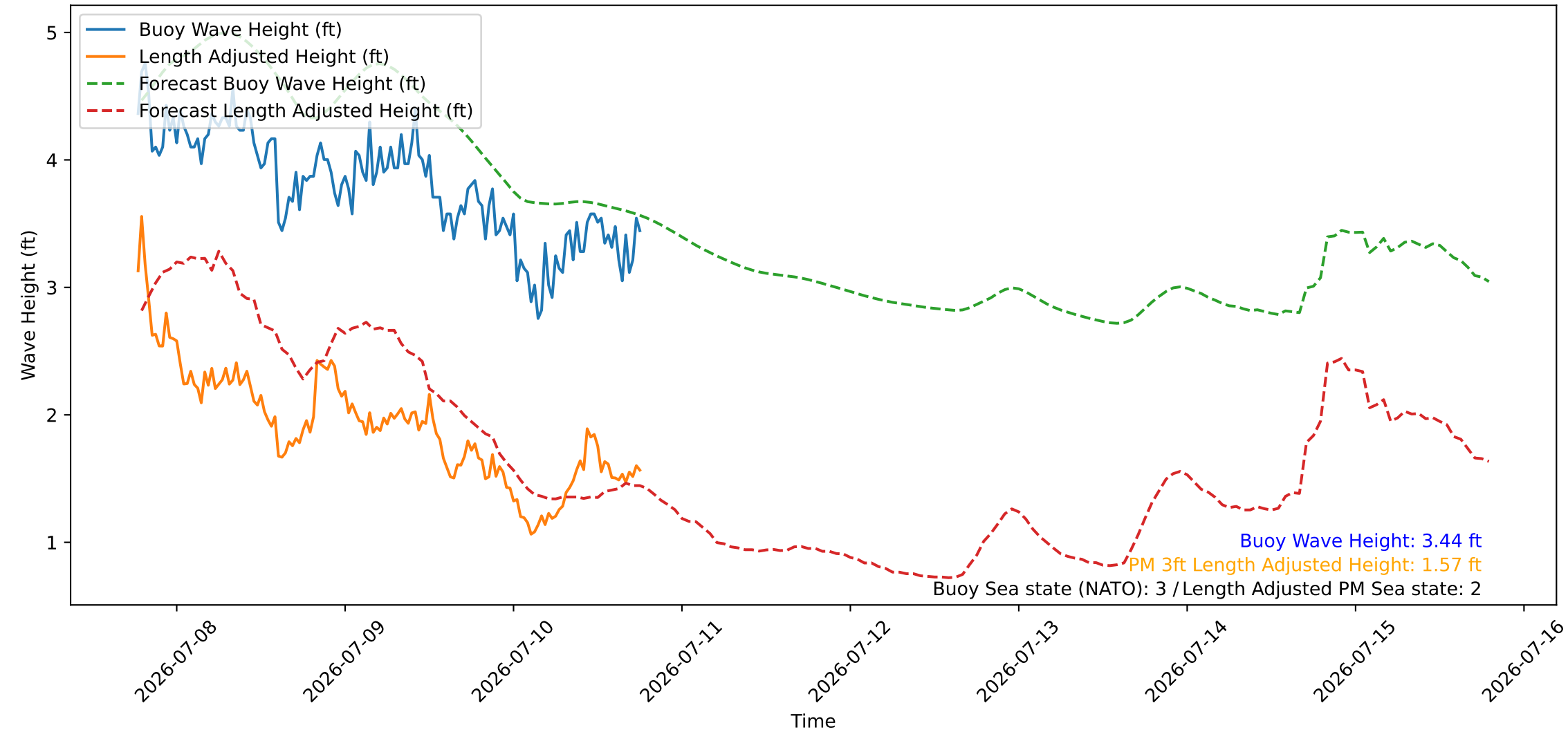
Wave Heights over Time for Green Beach at 2026-07-10 18:41:08
