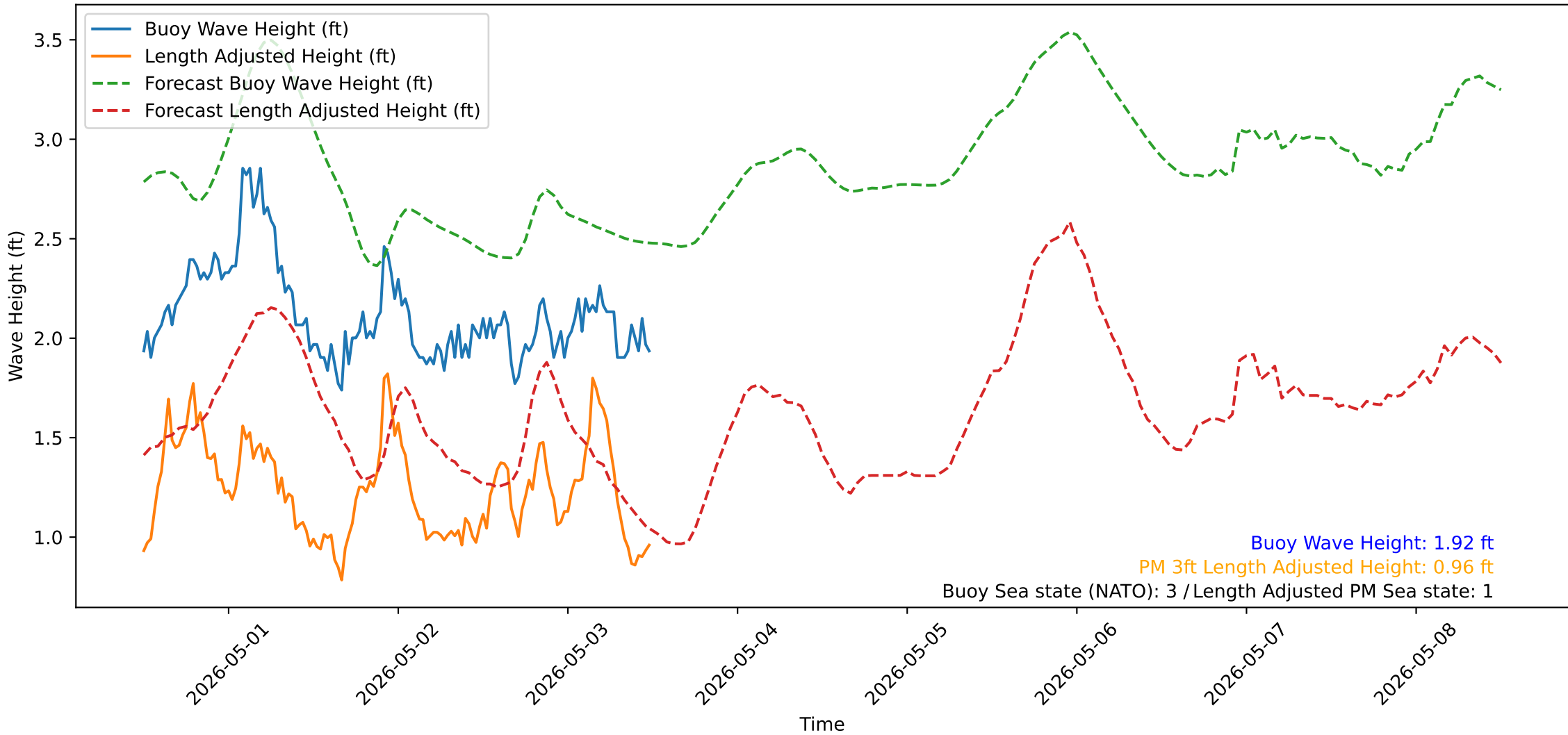
Wave Heights over Time for Green Beach at 2026-05-03 12:11:13
