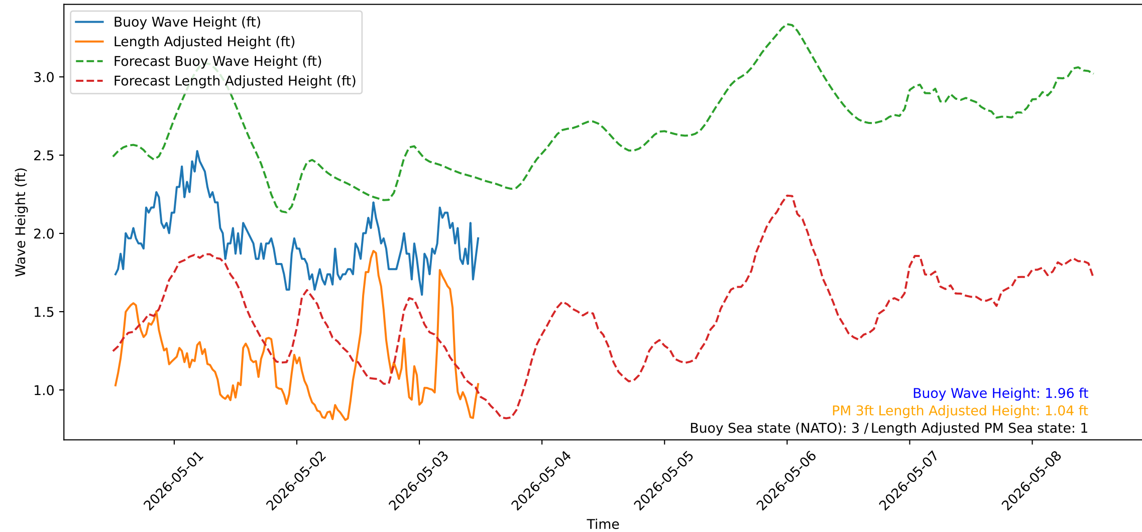
Wave Heights over Time for Red Beach at 2026-05-03 12:10:51
