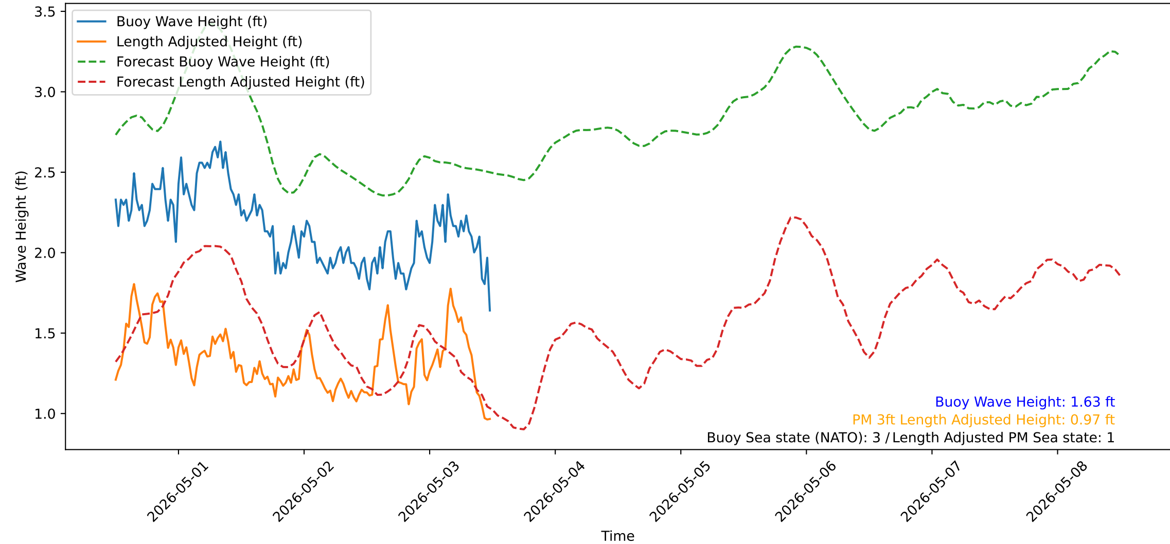
Wave Heights over Time for Oceanside Harbor at 2026-05-03 12:10:32
