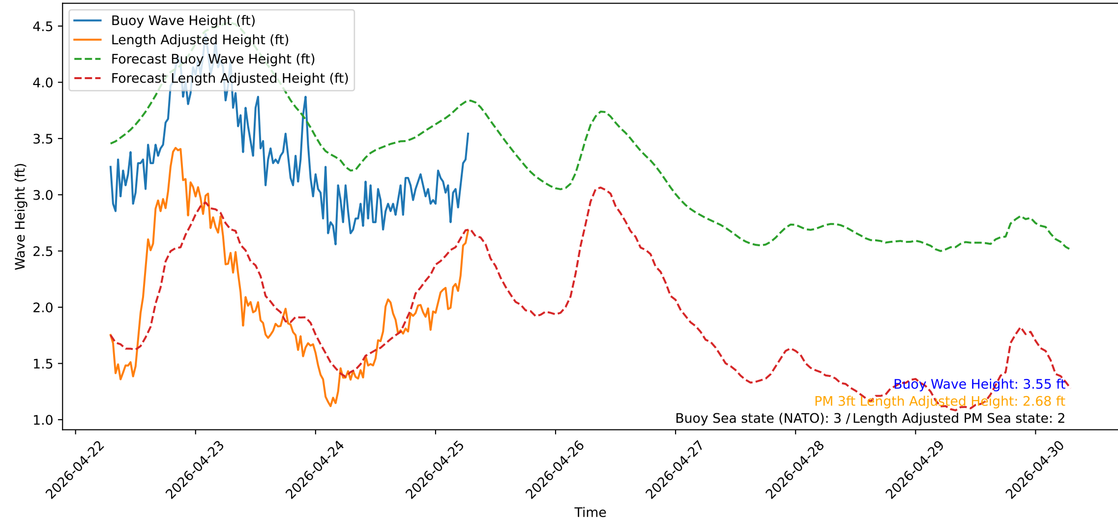
Wave Heights over Time for Oceanside Harbor at 2026-04-25 07:10:31
