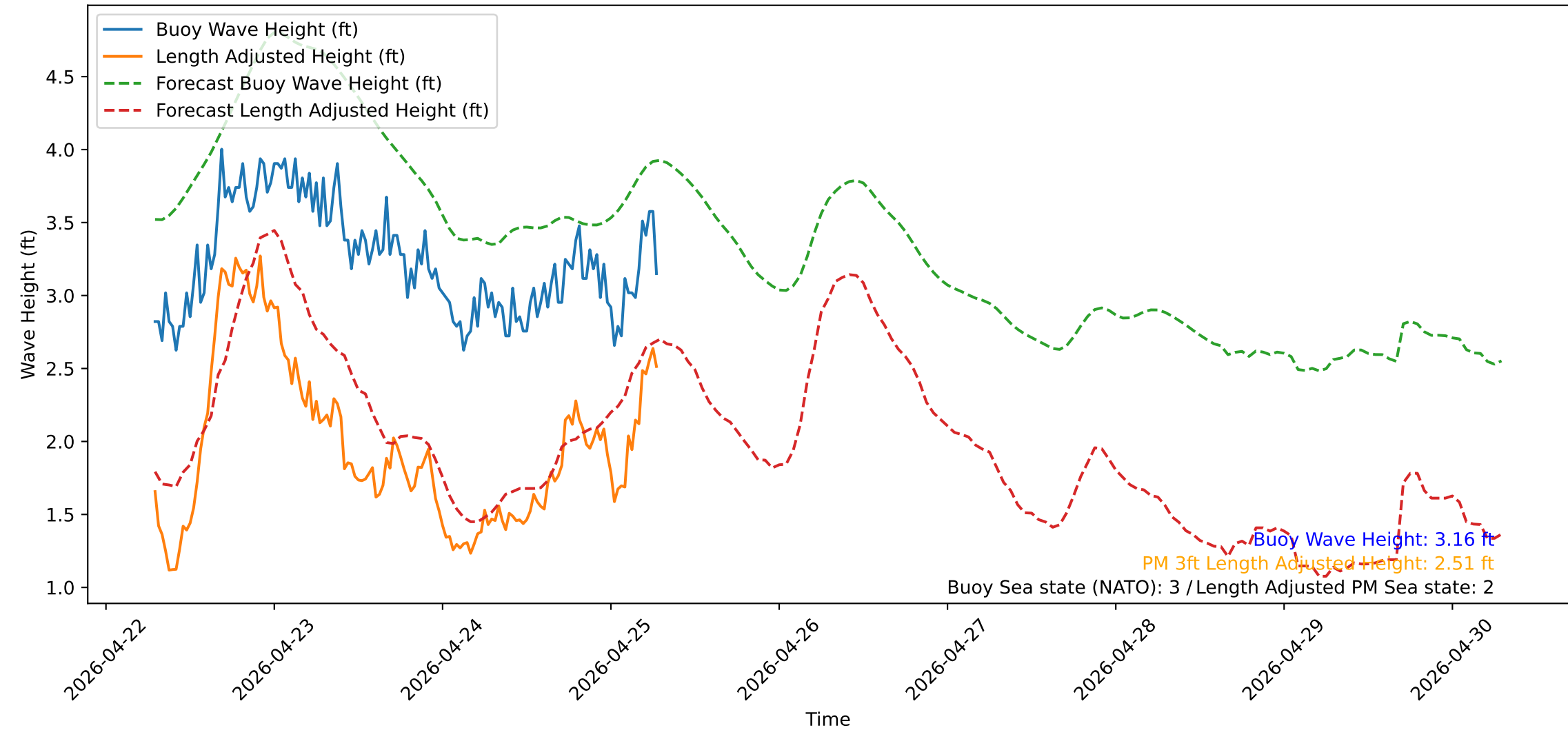
Wave Heights over Time for Green Beach at 2026-04-25 07:11:13
