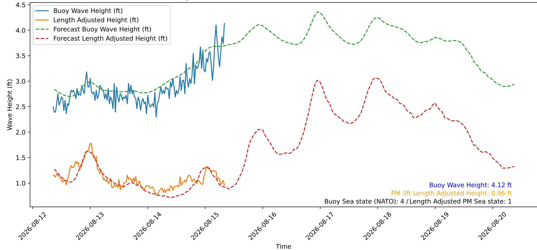
Wave Heights over Time for Oceanside Harbor at 2026-08-15 08:40:27
