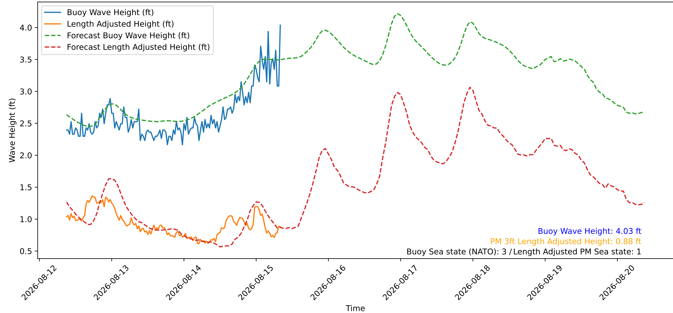
Wave Heights over Time for Red Beach at 2026-08-15 08:40:47
