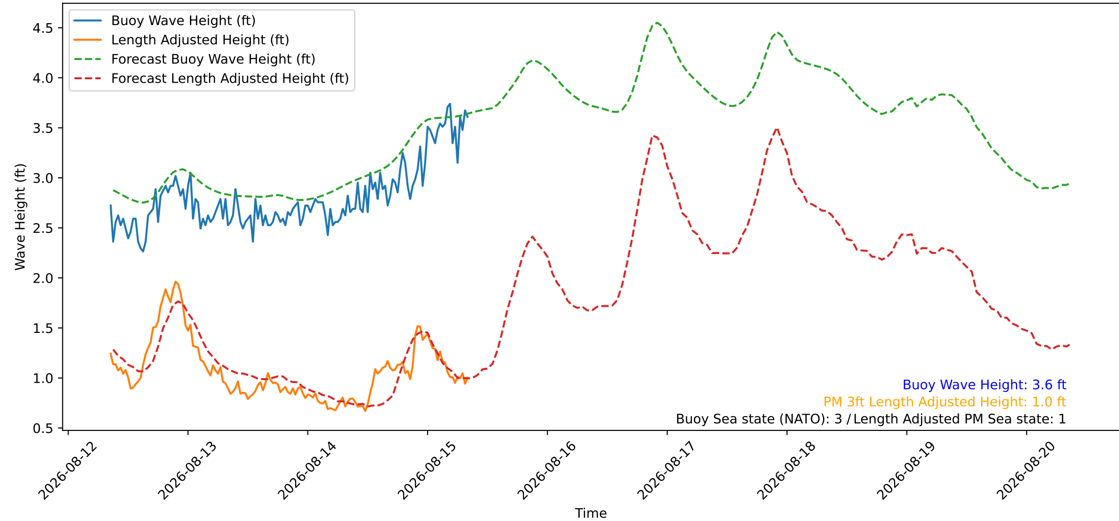
Wave Heights over Time for Green Beach at 2026-08-15 08:41:09
