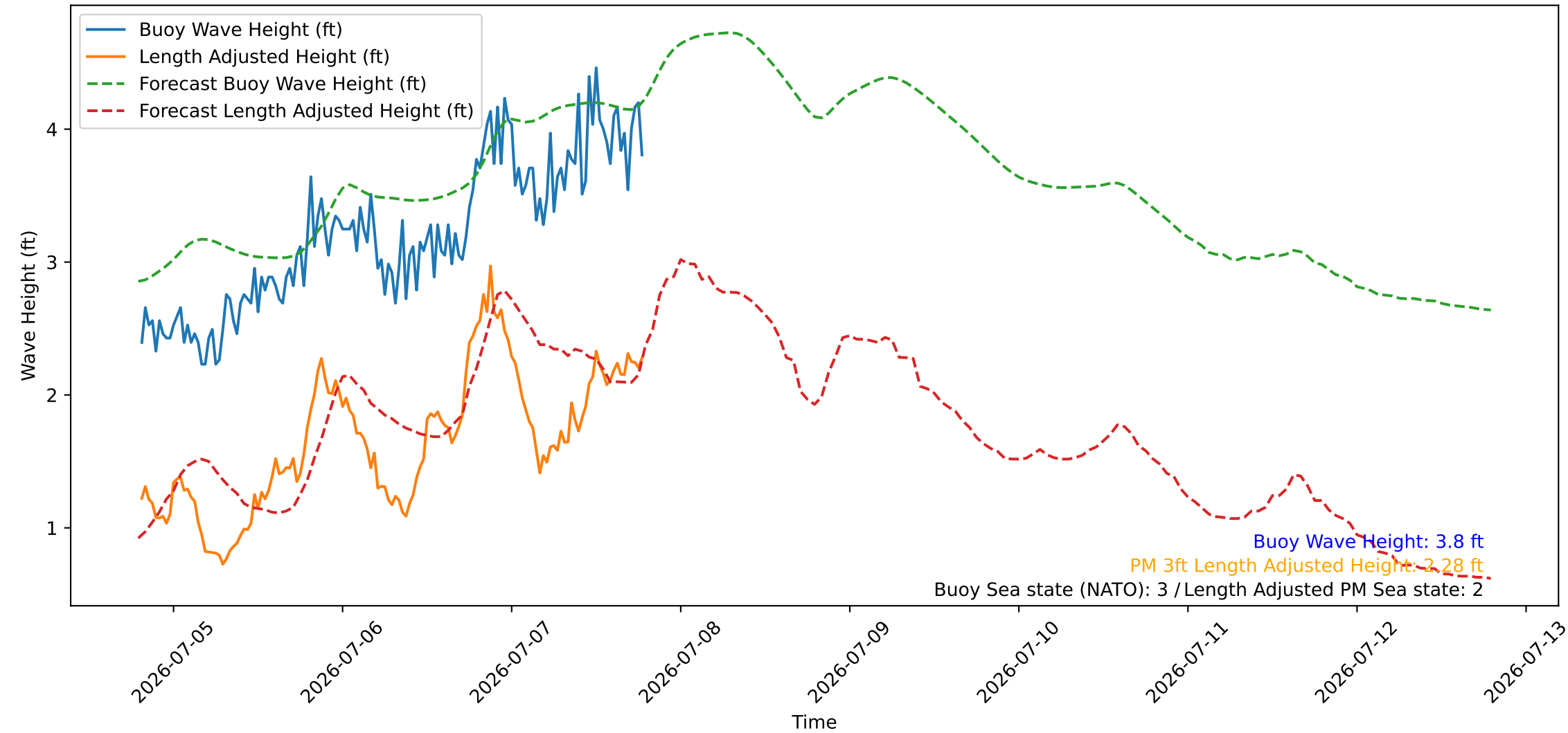
Wave Heights over Time for Red Beach at 2026-07-07 19:20:47
