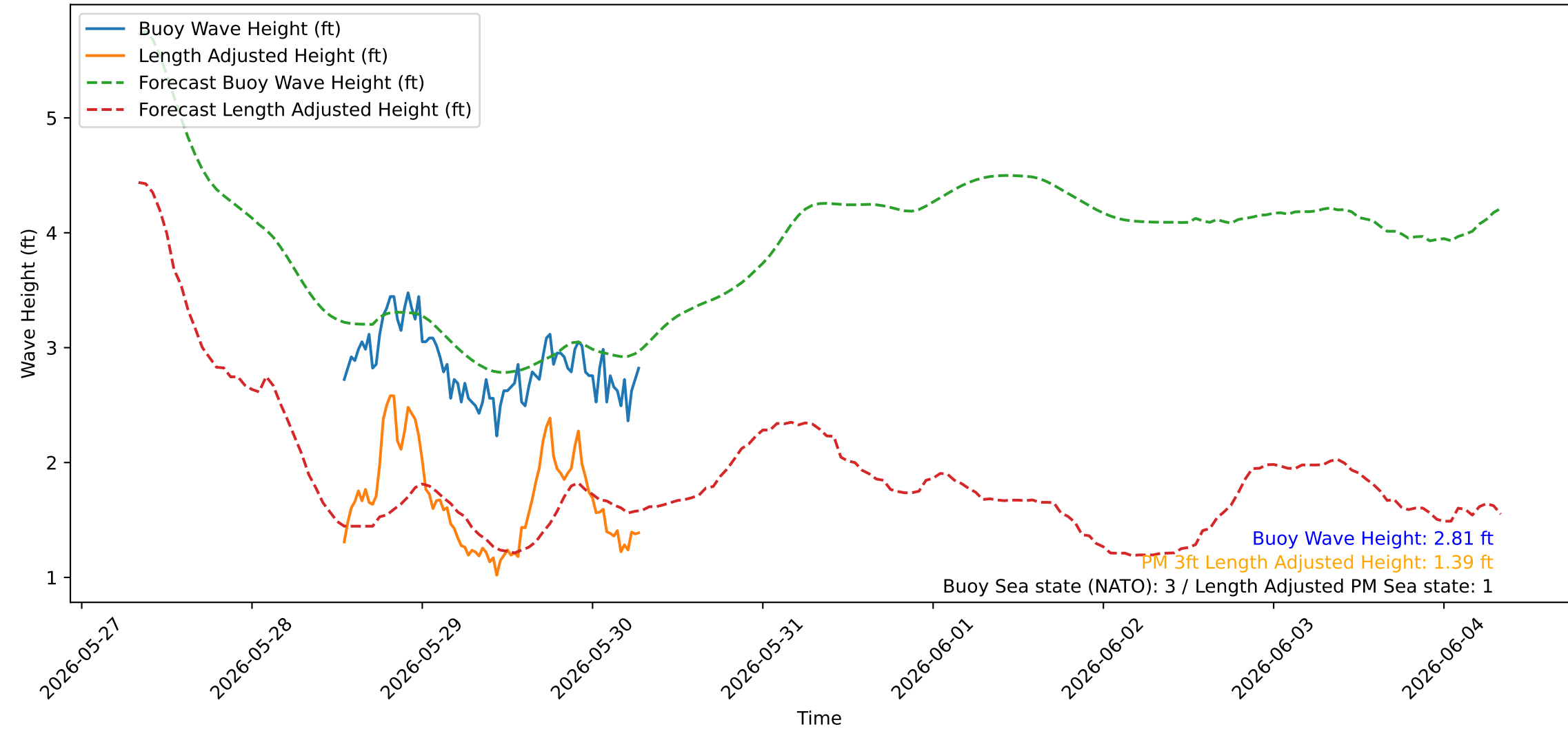
Wave Heights over Time for Oceanside Harbor at 2026-05-30 07:30:23
