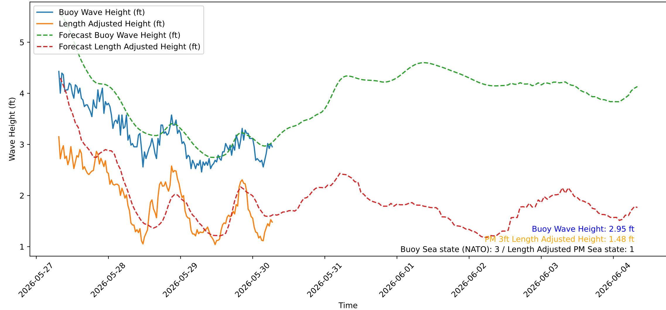
Wave Heights over Time for Green Beach at 2026-05-30 07:31:04
