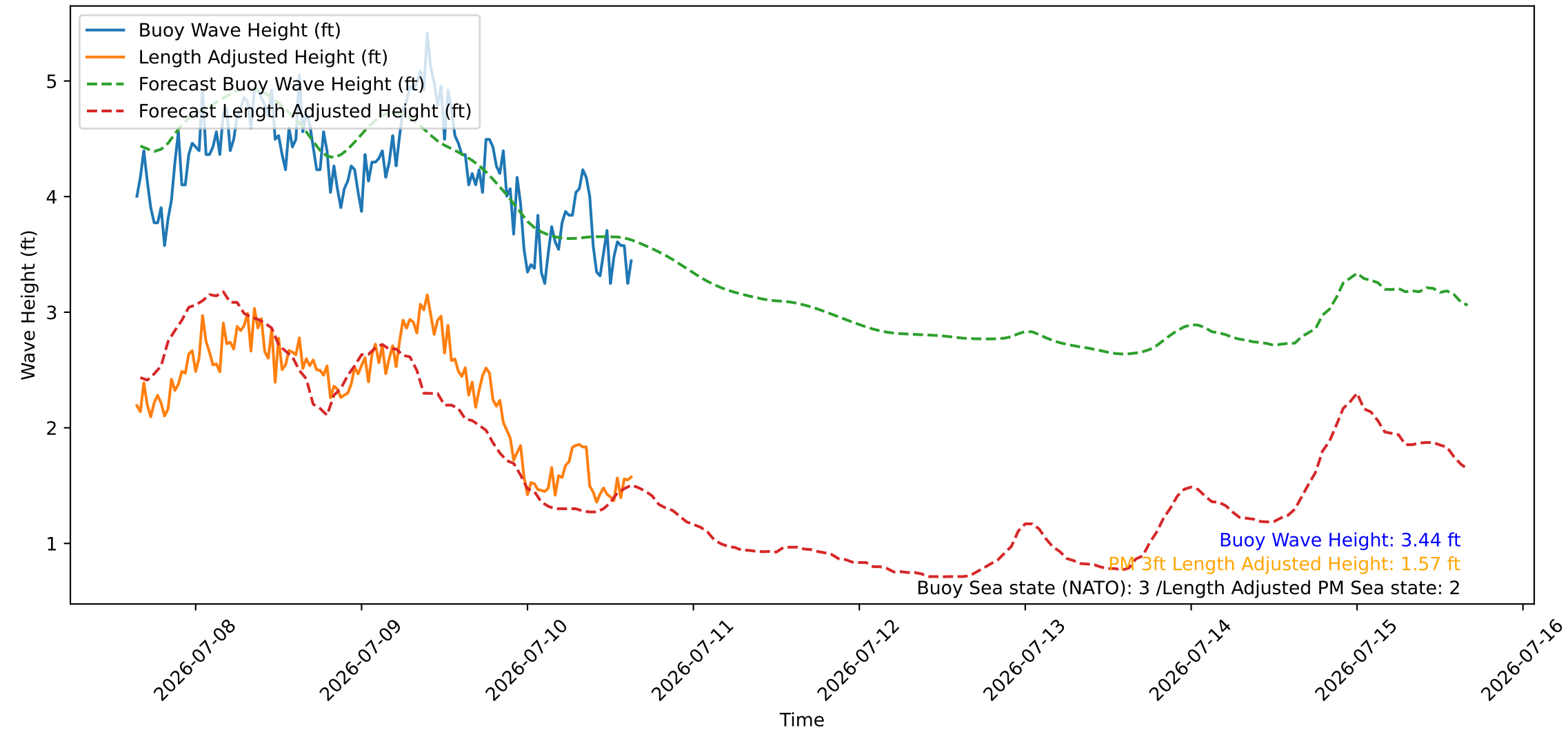
Wave Heights over Time for Oceanside Harbor at 2026-07-10 15:30:27
