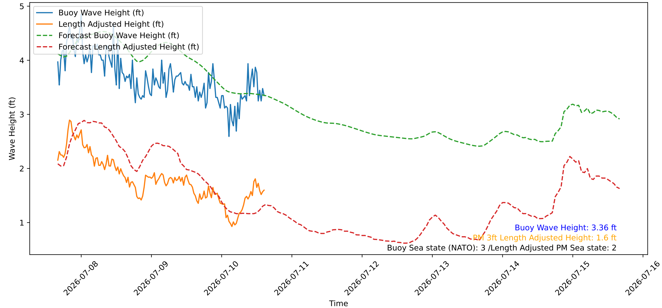
Wave Heights over Time for Red Beach at 2026-07-10 15:30:47
