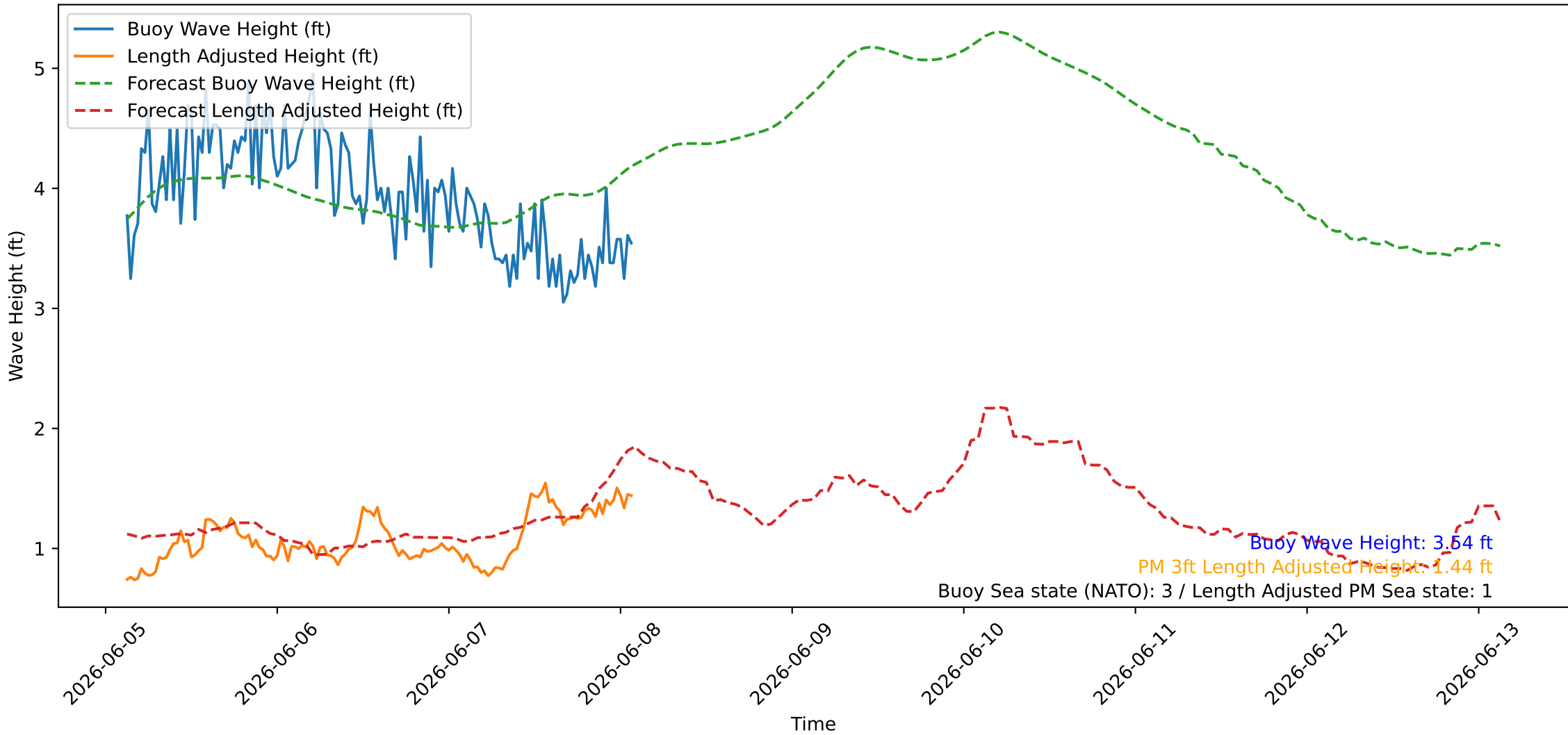
Wave Heights over Time for Red Beach at 2026-06-08 02:30:46
