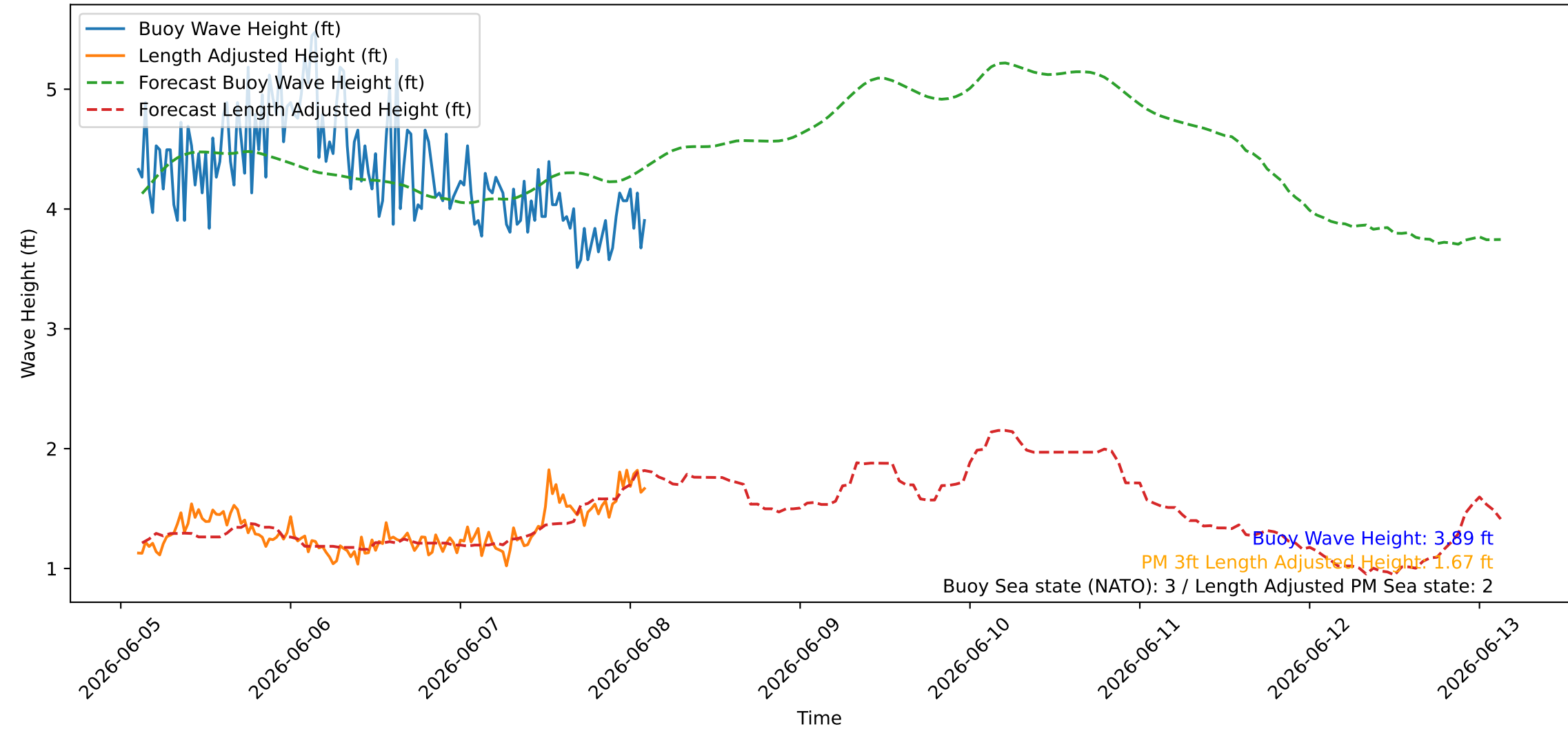
Wave Heights over Time for Oceanside Harbor at 2026-06-08 02:30:26
