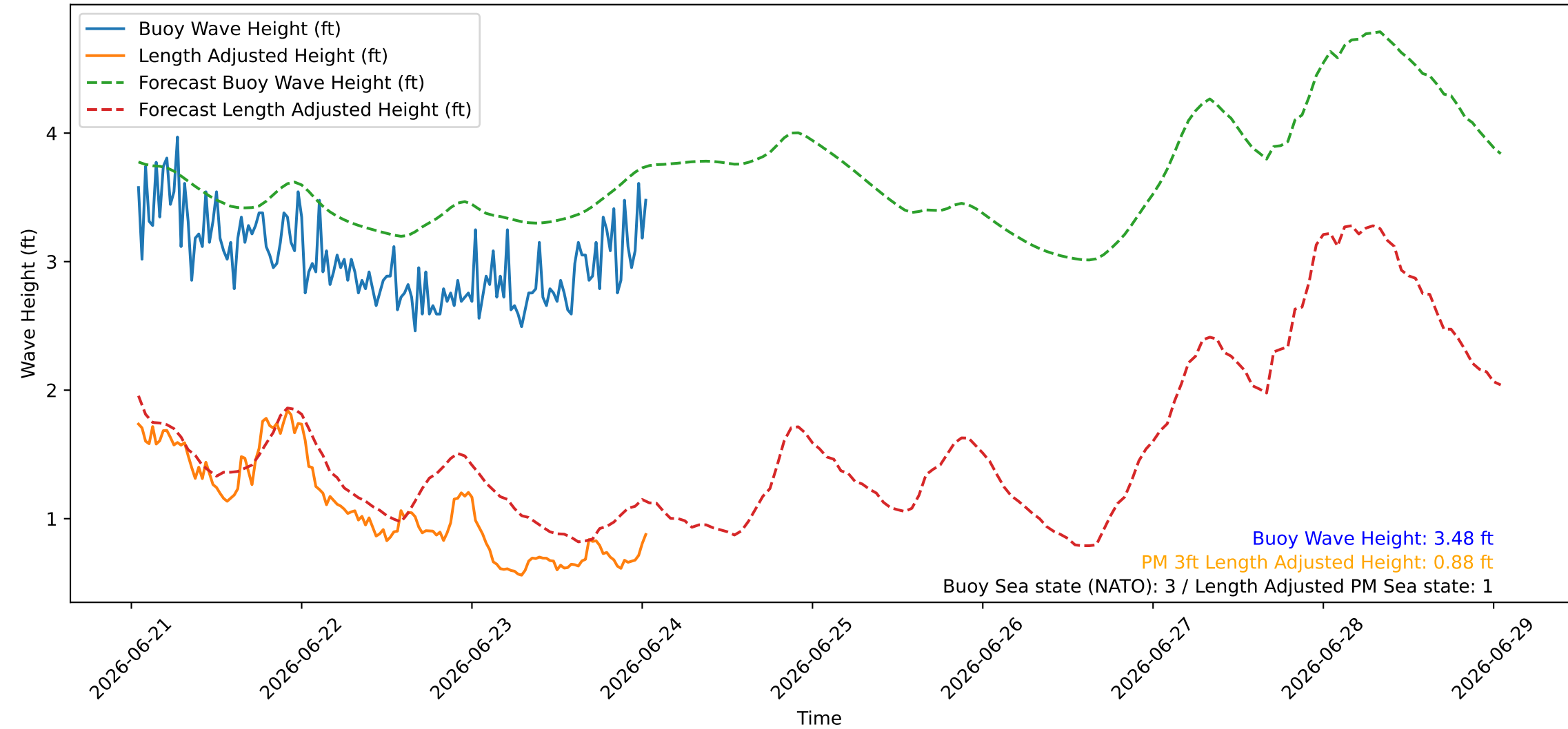
Wave Heights over Time for Green Beach at 2026-06-24 01:11:07
