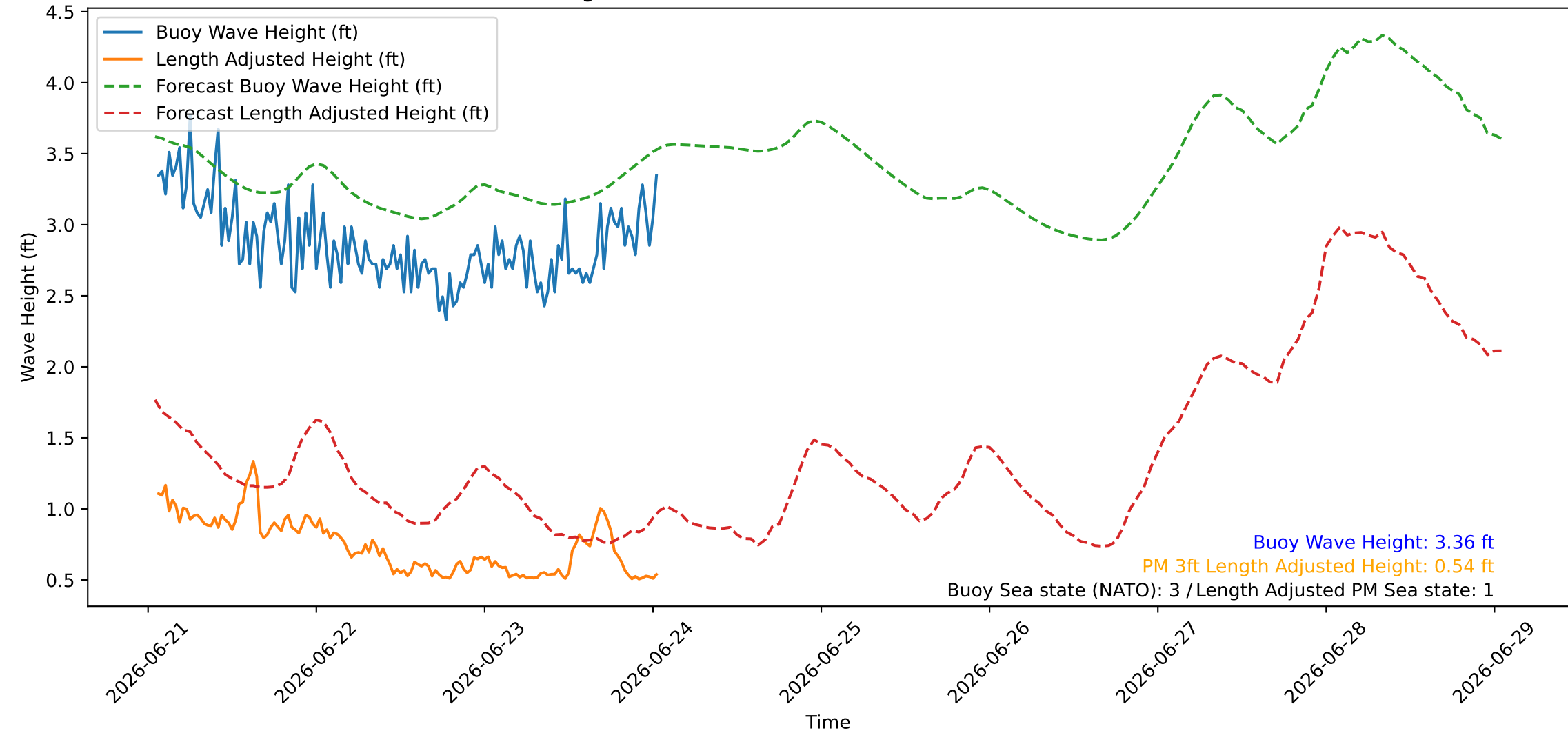
Wave Heights over Time for Red Beach at 2026-06-24 01:10:45
