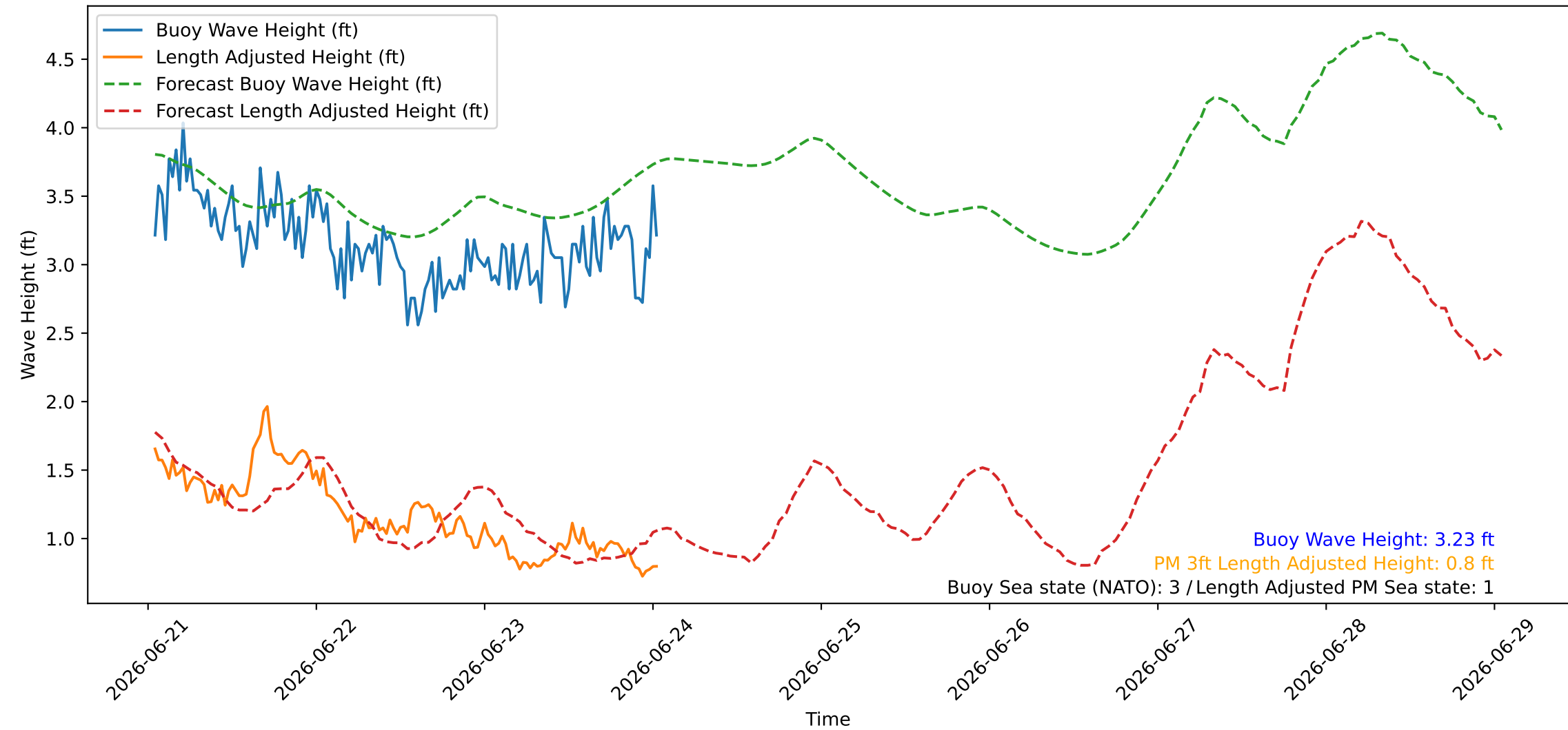
Wave Heights over Time for Oceanside Harbor at 2026-06-24 01:10:26
