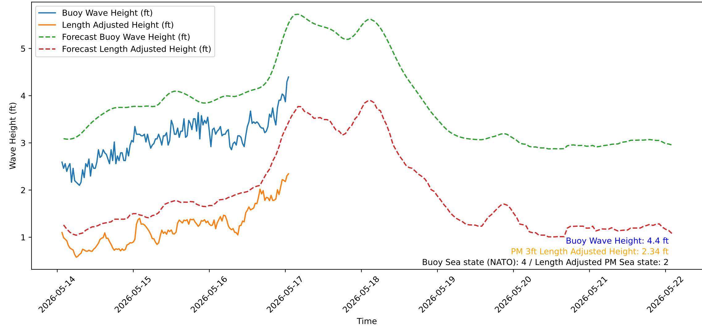
Wave Heights over Time for Green Beach at 2026-05-17 01:41:14
