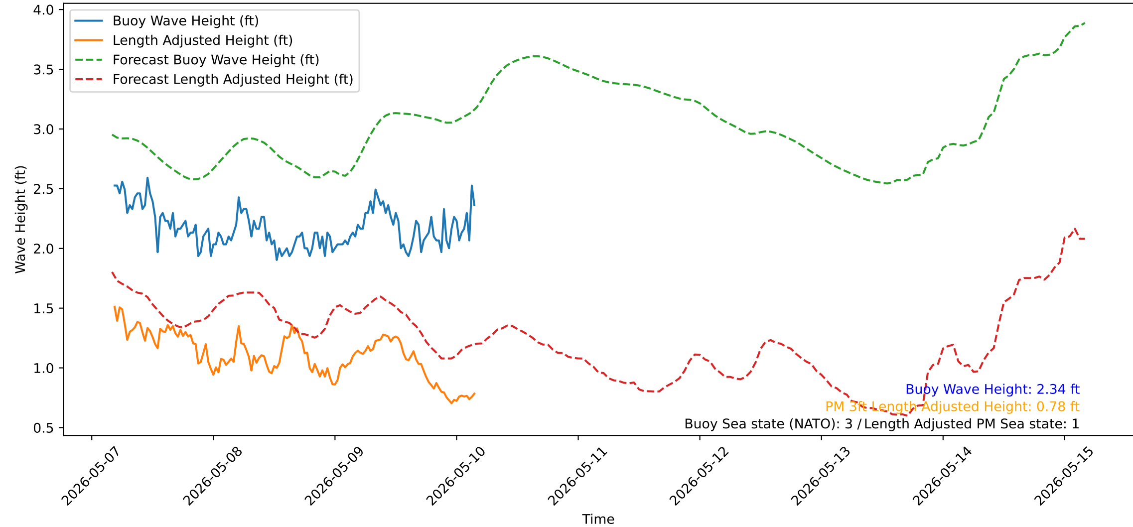
Wave Heights over Time for Red Beach at 2026-05-10 04:20:52
