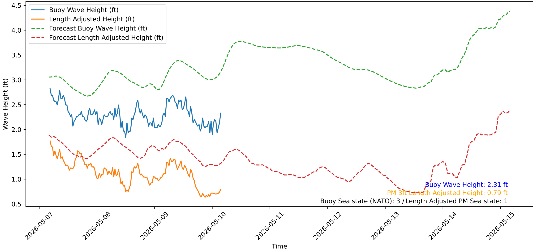
Wave Heights over Time for Green Beach at 2026-05-10 04:21:15
