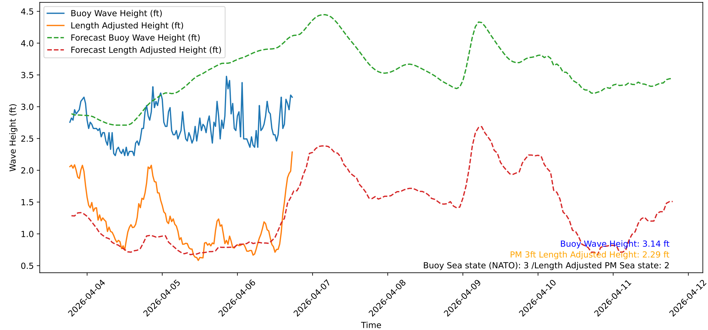
Wave Heights over Time for Green Beach at 2026-04-06 18:31:10
