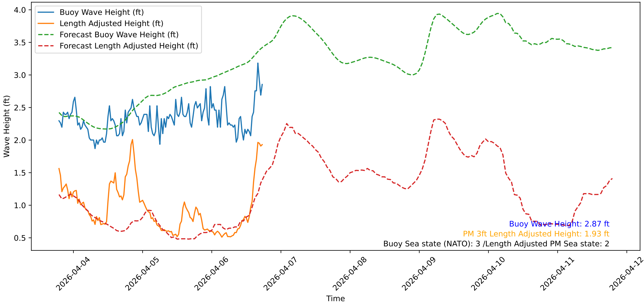
Wave Heights over Time for Red Beach at 2026-04-06 18:30:48
