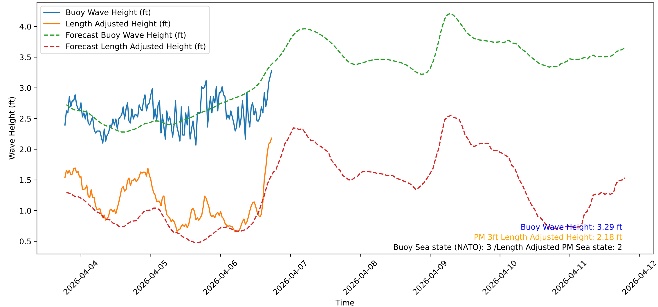
Wave Heights over Time for Oceanside Harbor at 2026-04-06 18:30:32
