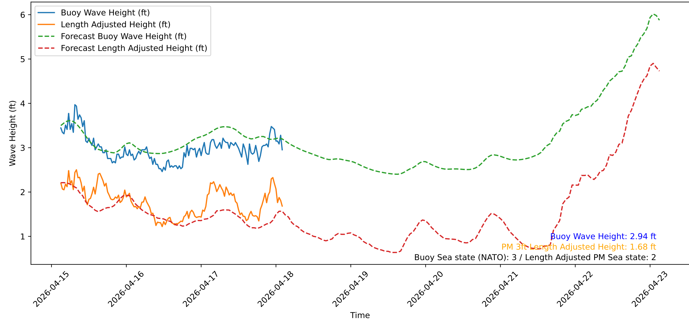
Wave Heights over Time for Green Beach at 2026-04-18 02:51:13
