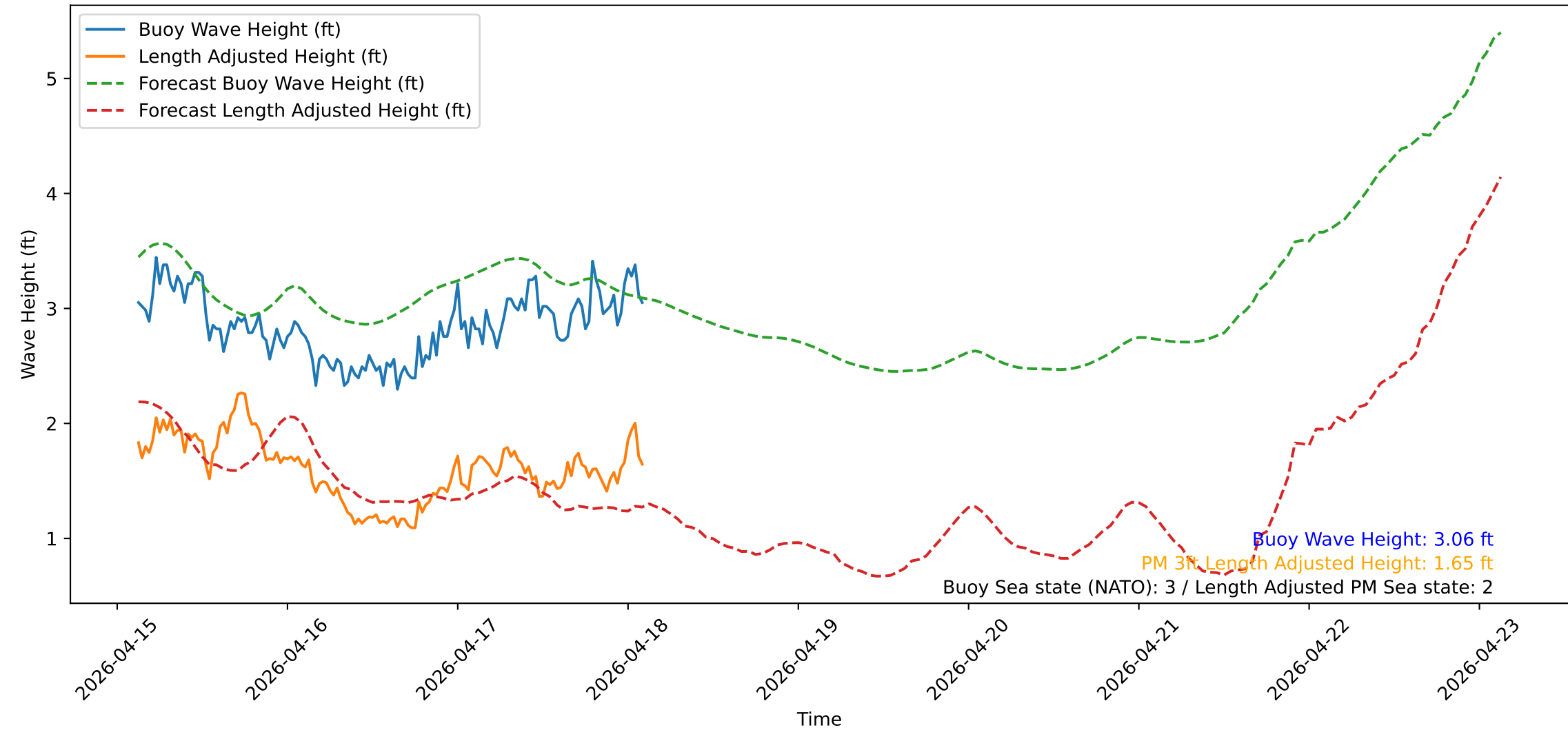
Wave Heights over Time for Oceanside Harbor at 2026-04-18 02:50:31
