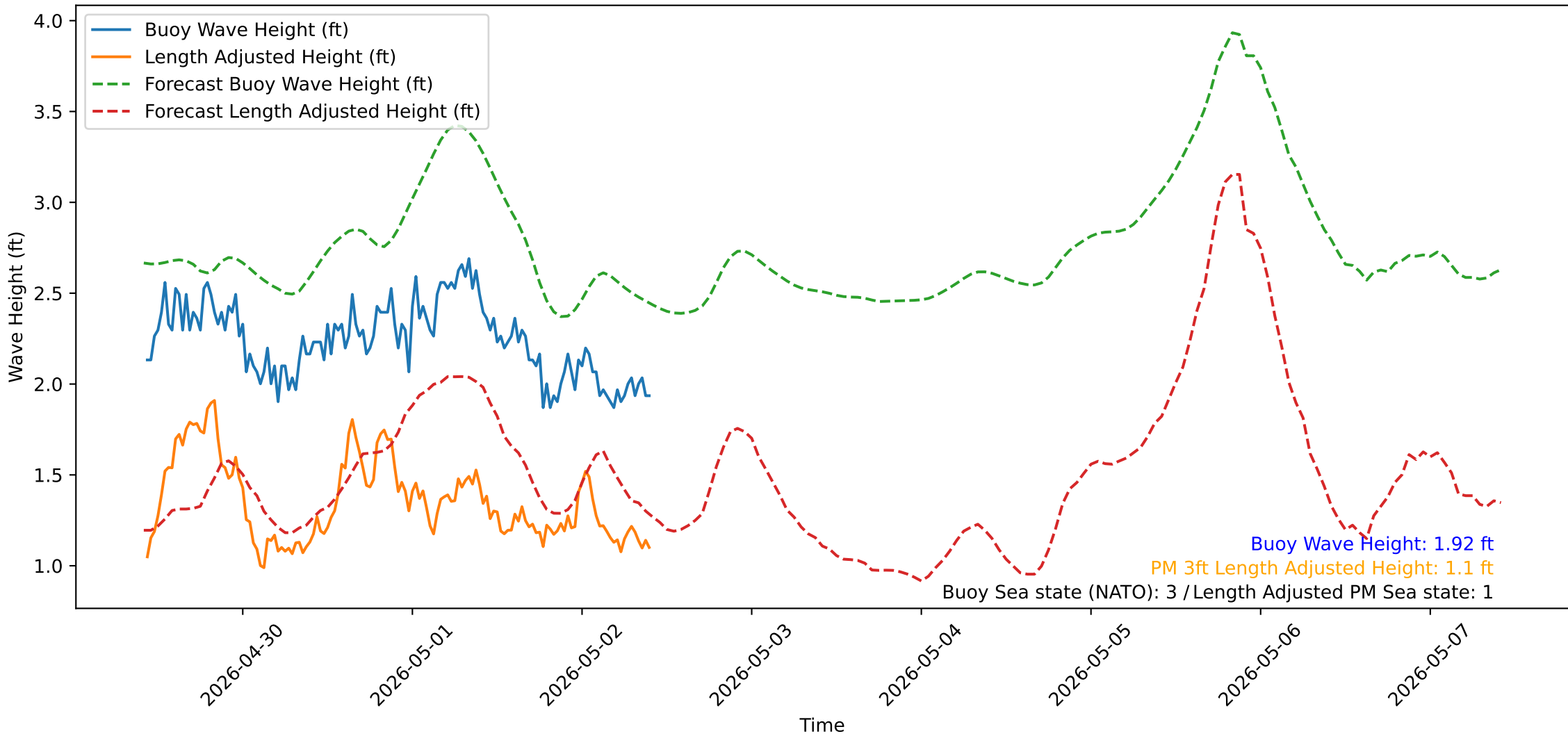
Wave Heights over Time for Oceanside Harbor at 2026-05-02 10:20:31
