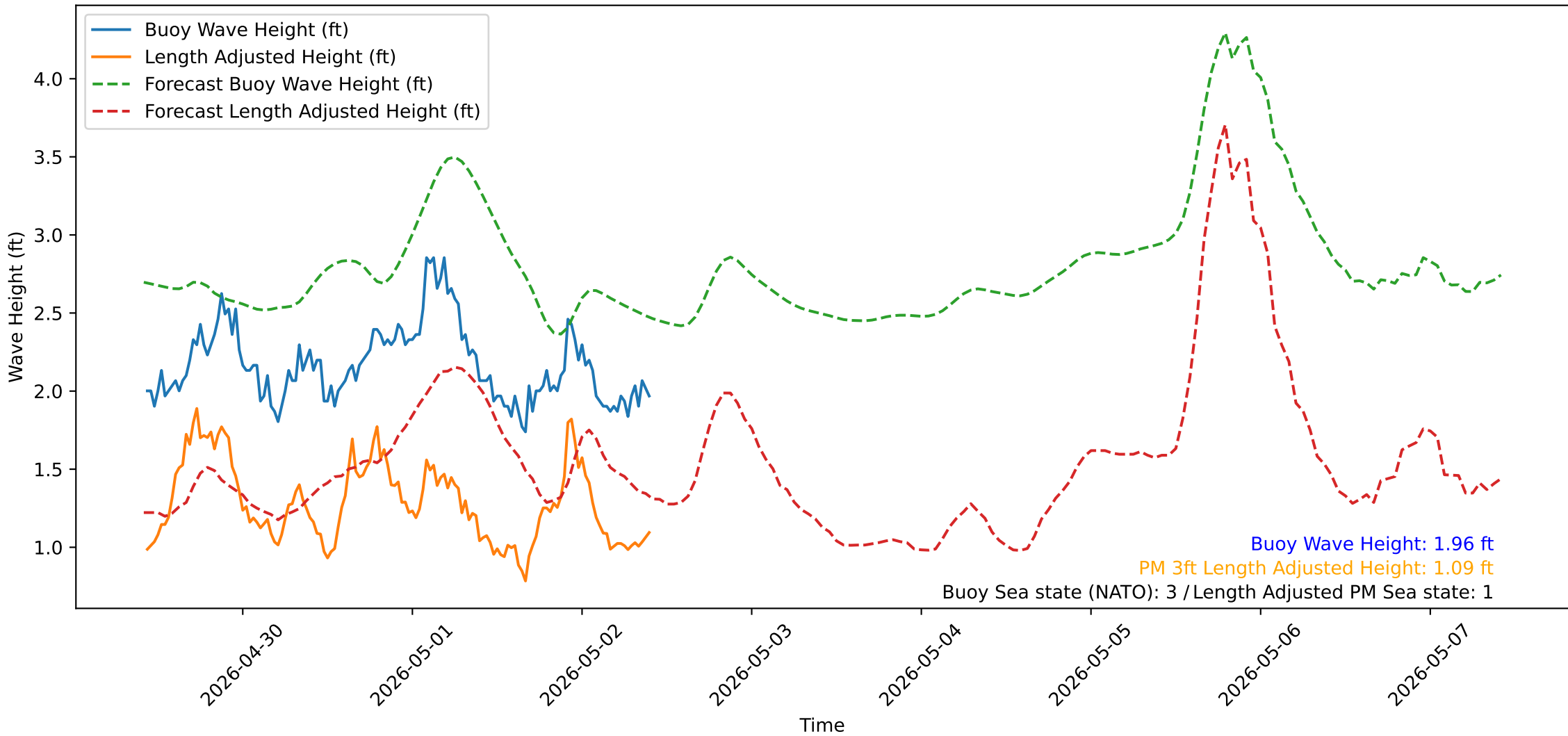
Wave Heights over Time for Green Beach at 2026-05-02 10:21:14
