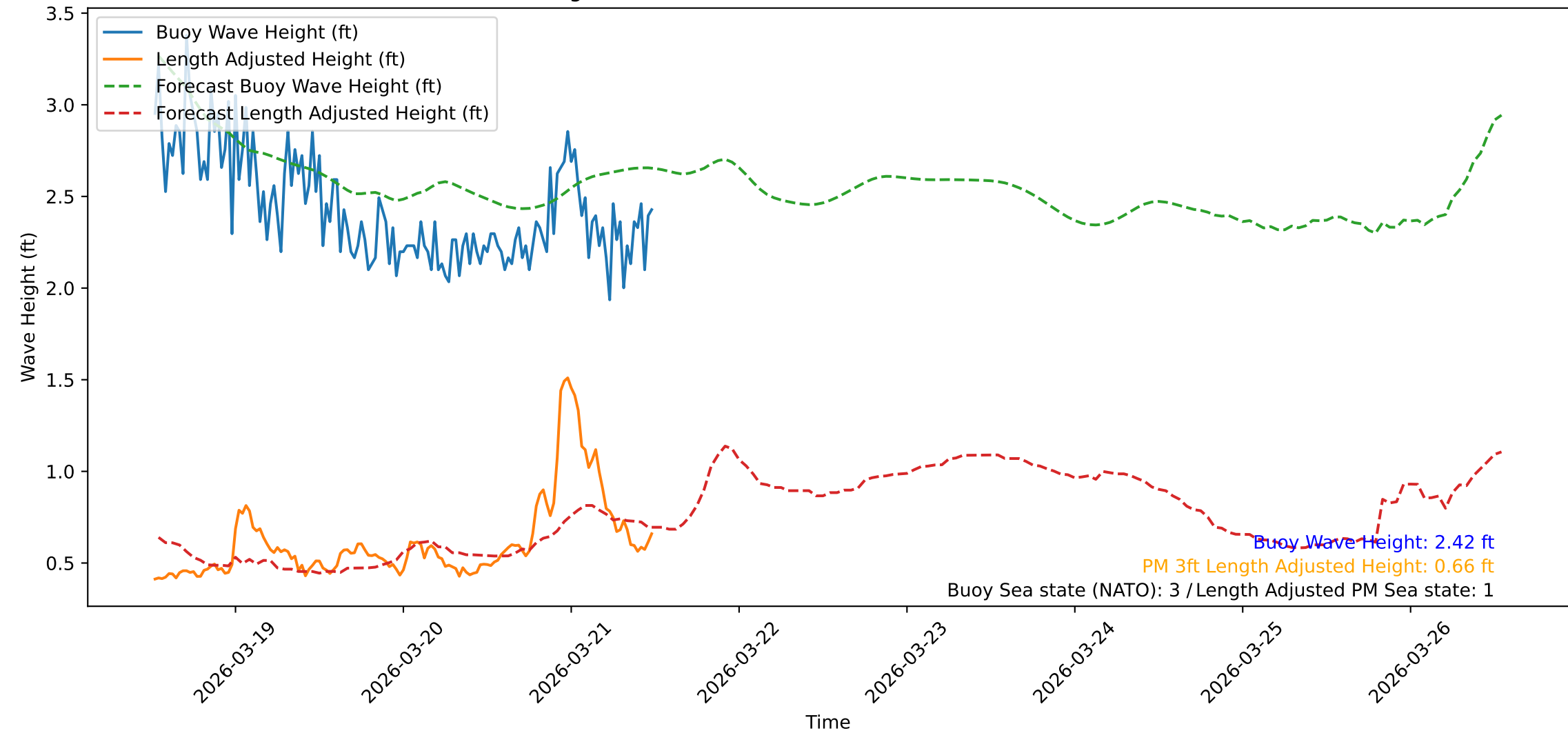
Wave Heights over Time for Green Beach at 2026-03-21 12:31:10
