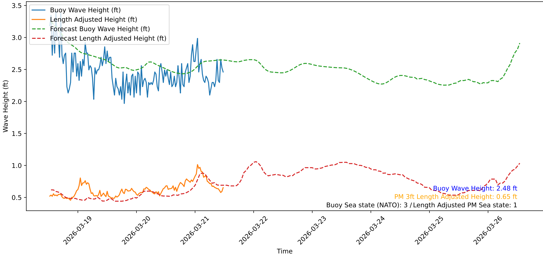
Wave Heights over Time for Oceanside Harbor at 2026-03-21 12:30:31
