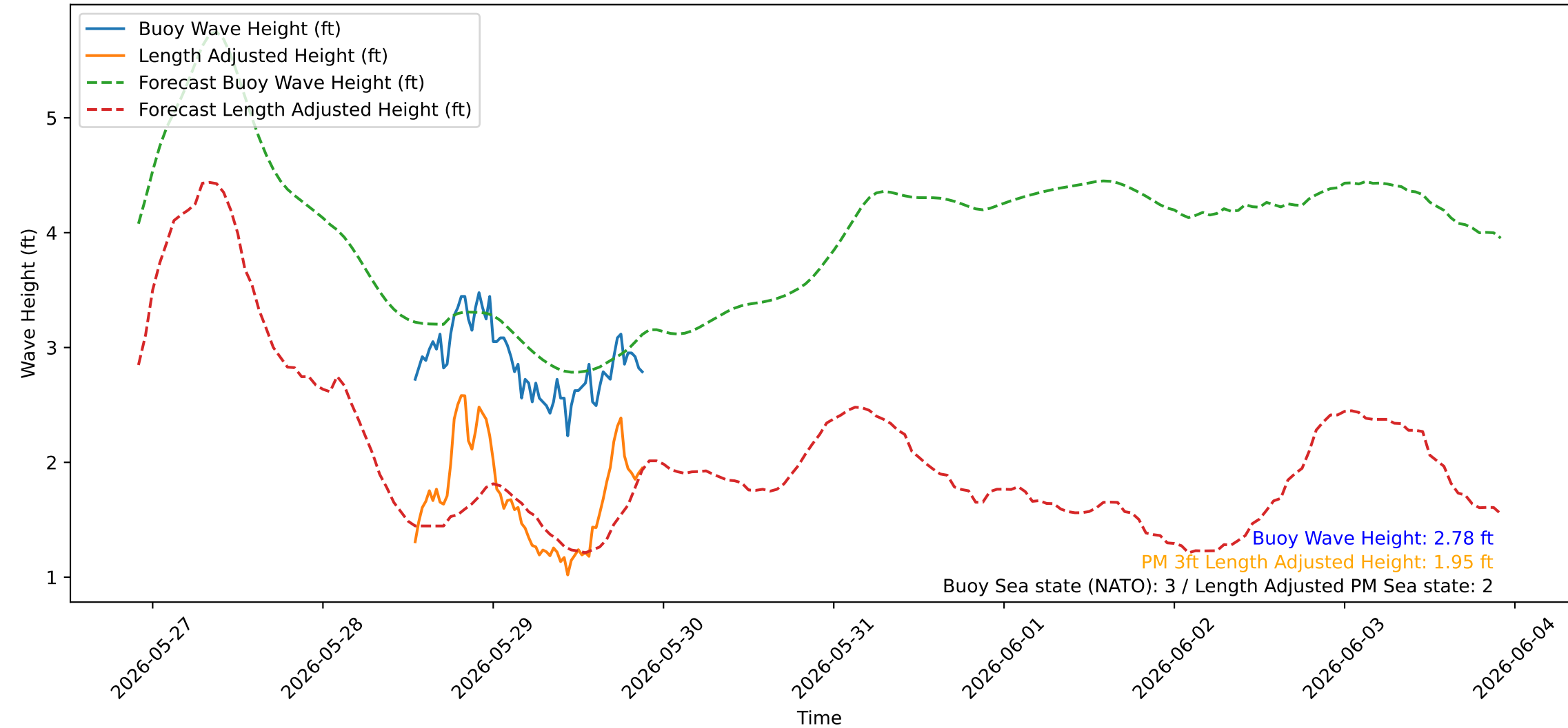
Wave Heights over Time for Oceanside Harbor at 2026-05-29 21:40:22
