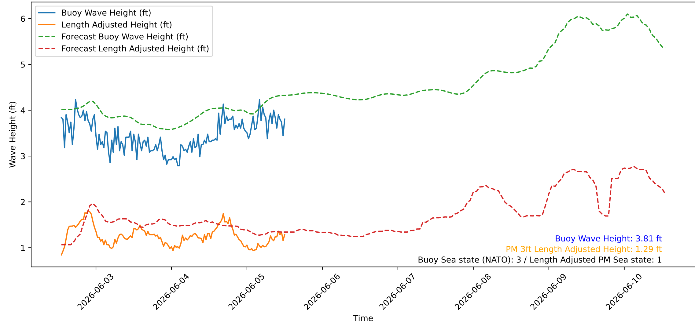
Wave Heights over Time for Green Beach at 2026-06-05 12:51:09
