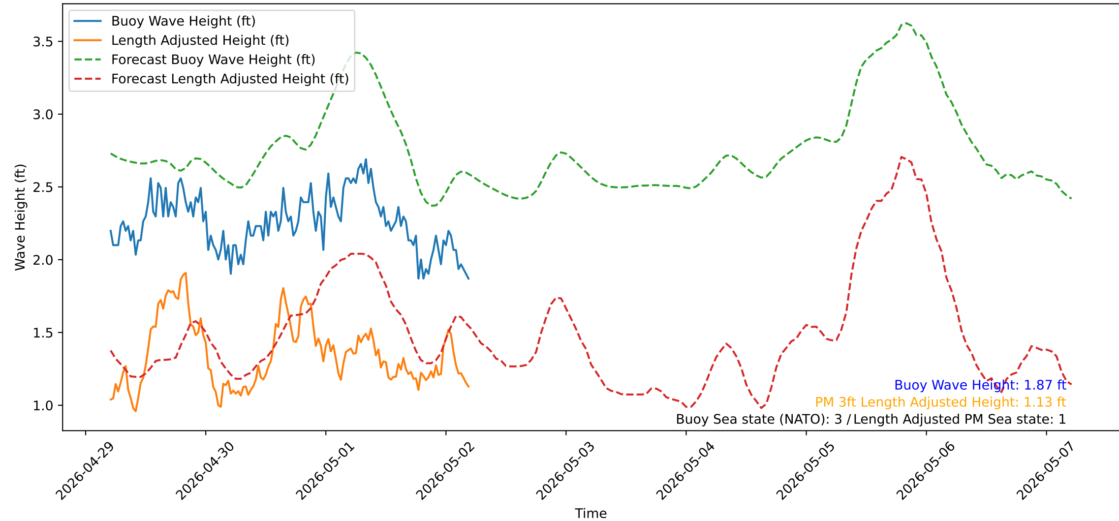
Wave Heights over Time for Oceanside Harbor at 2026-05-02 05:10:31
