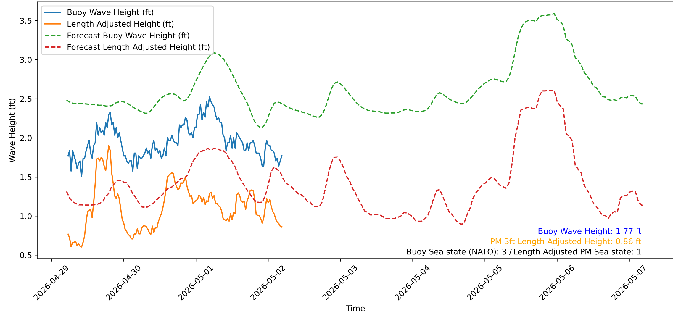
Wave Heights over Time for Red Beach at 2026-05-02 05:10:50
