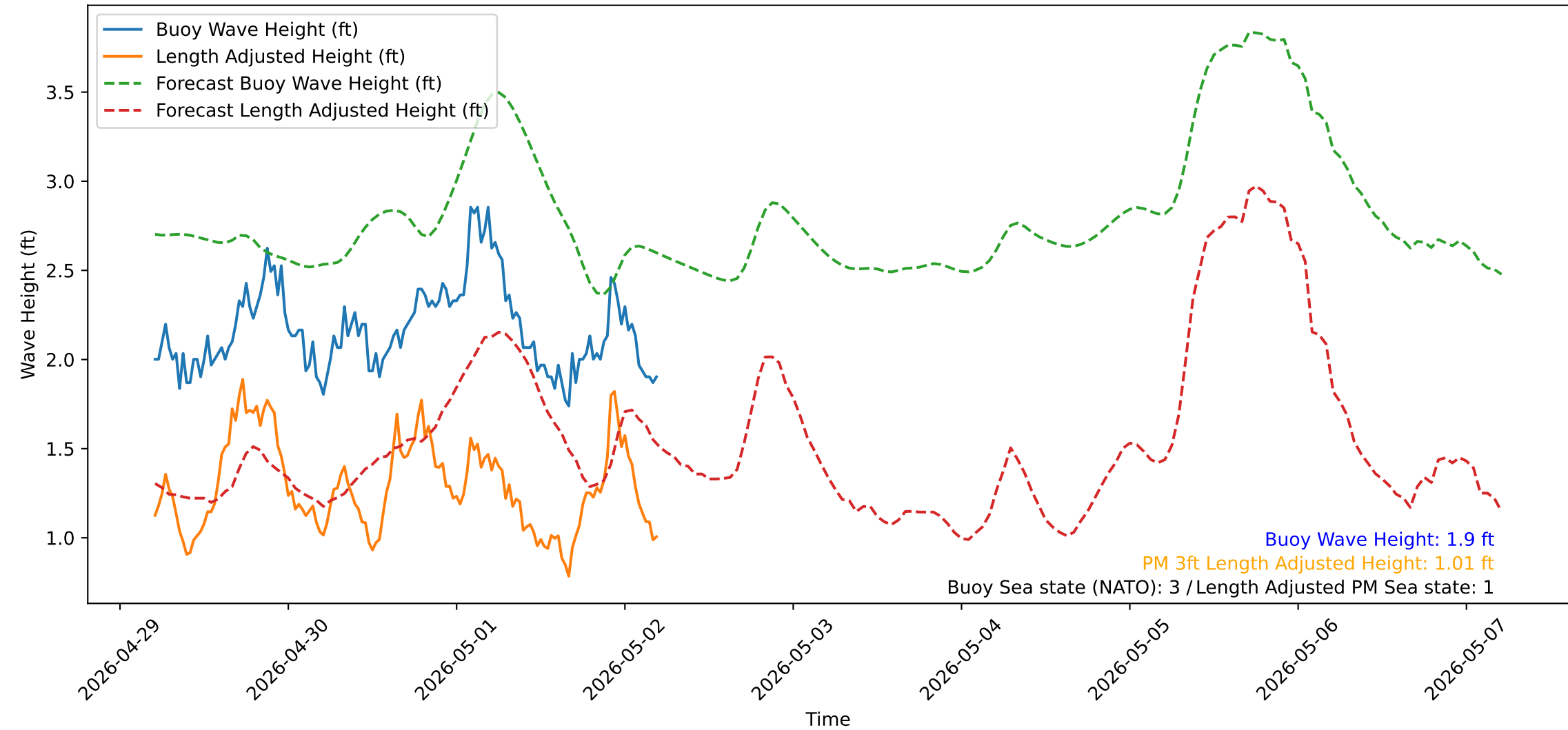
Wave Heights over Time for Green Beach at 2026-05-02 05:11:13
