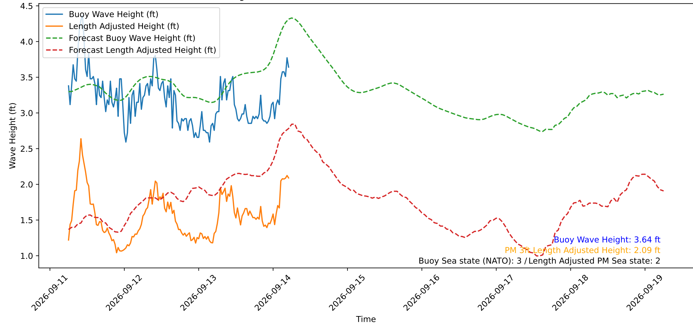
Wave Heights over Time for Oceanside Harbor at 2026-09-14 06:00:29
