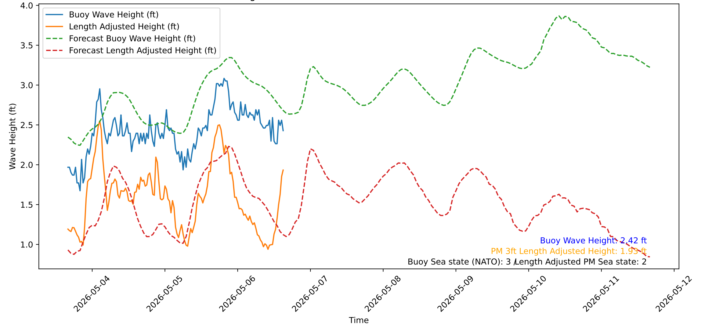
Wave Heights over Time for Red Beach at 2026-05-06 15:40:50
