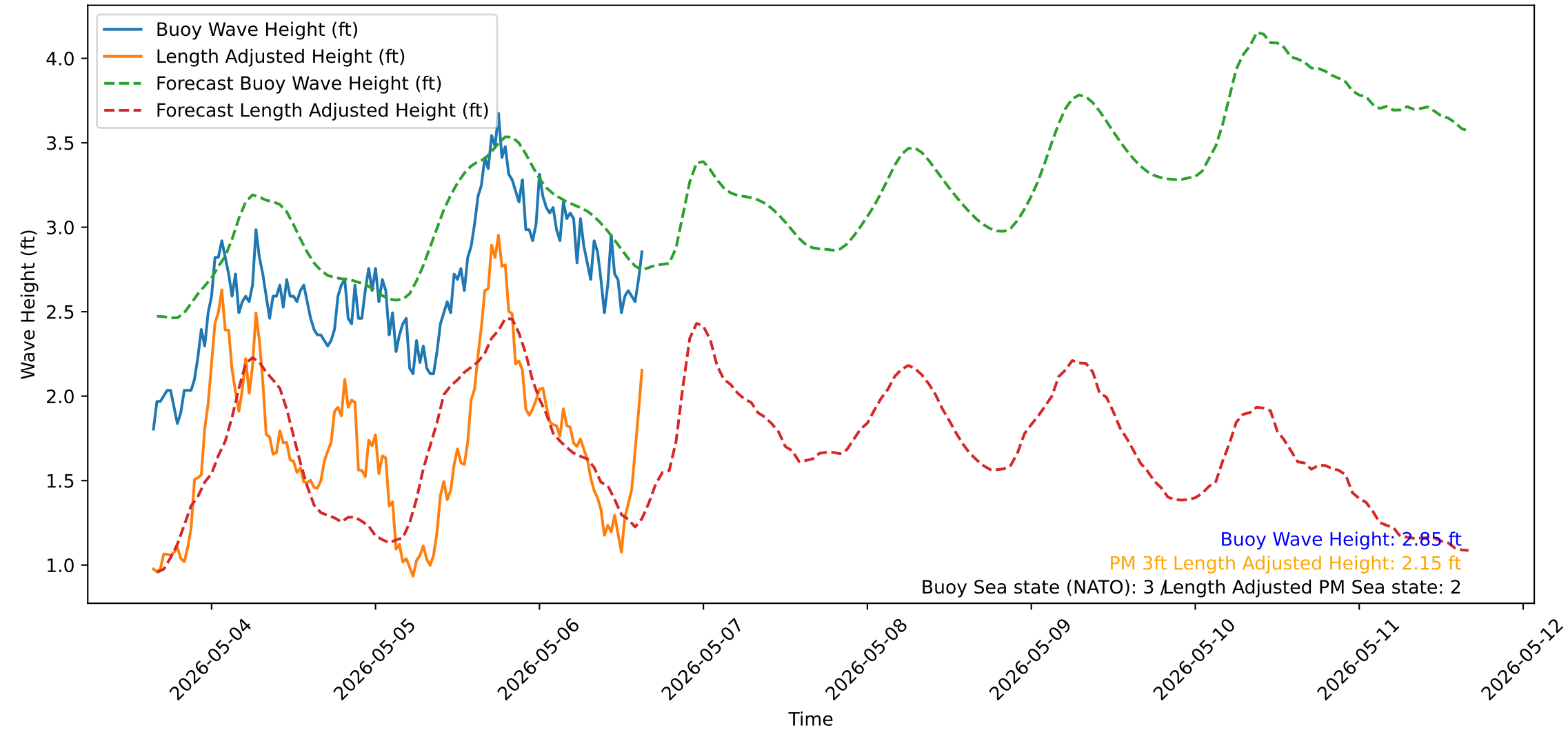
Wave Heights over Time for Green Beach at 2026-05-06 15:41:13
