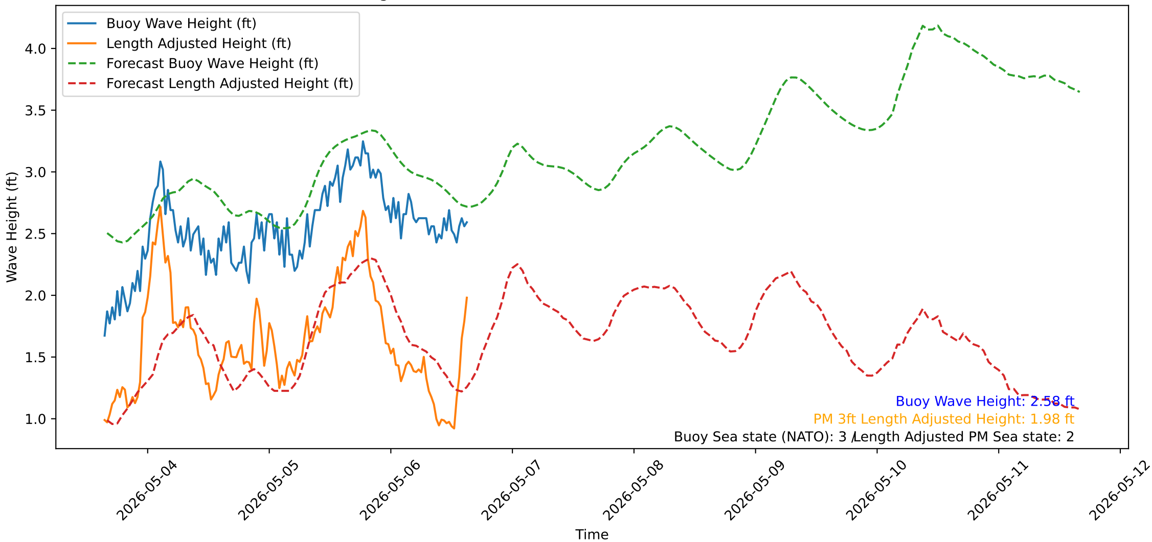
Wave Heights over Time for Oceanside Harbor at 2026-05-06 15:40:31
