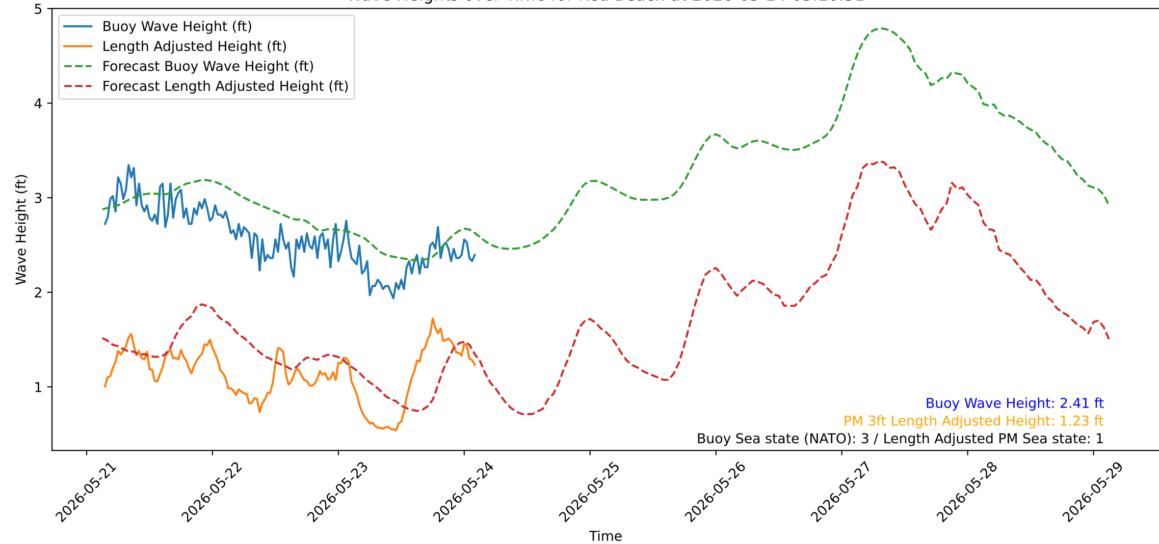
Wave Heights over Time for Red Beach at 2026-05-24 03:10:51
