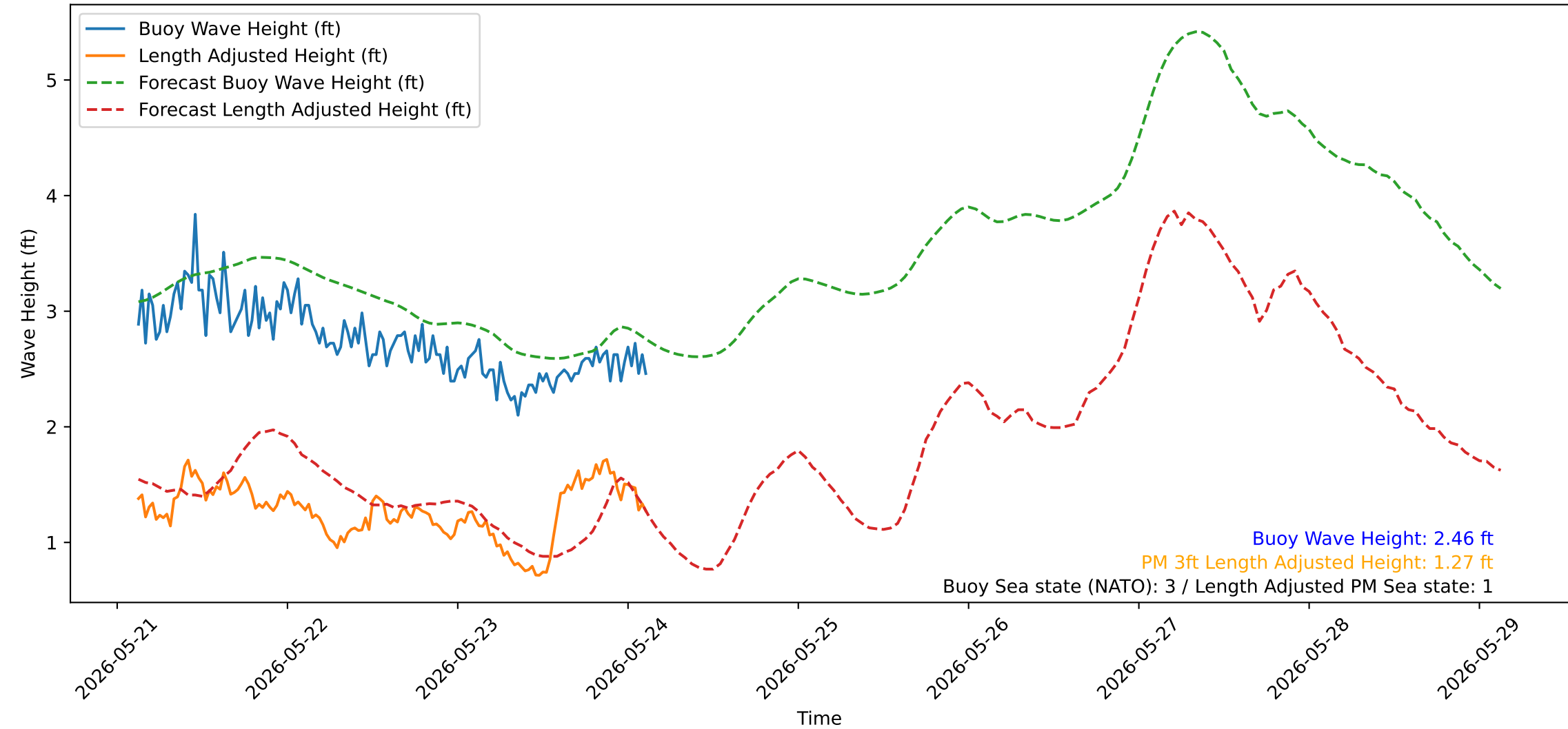
Wave Heights over Time for Oceanside Harbor at 2026-05-24 03:10:32
