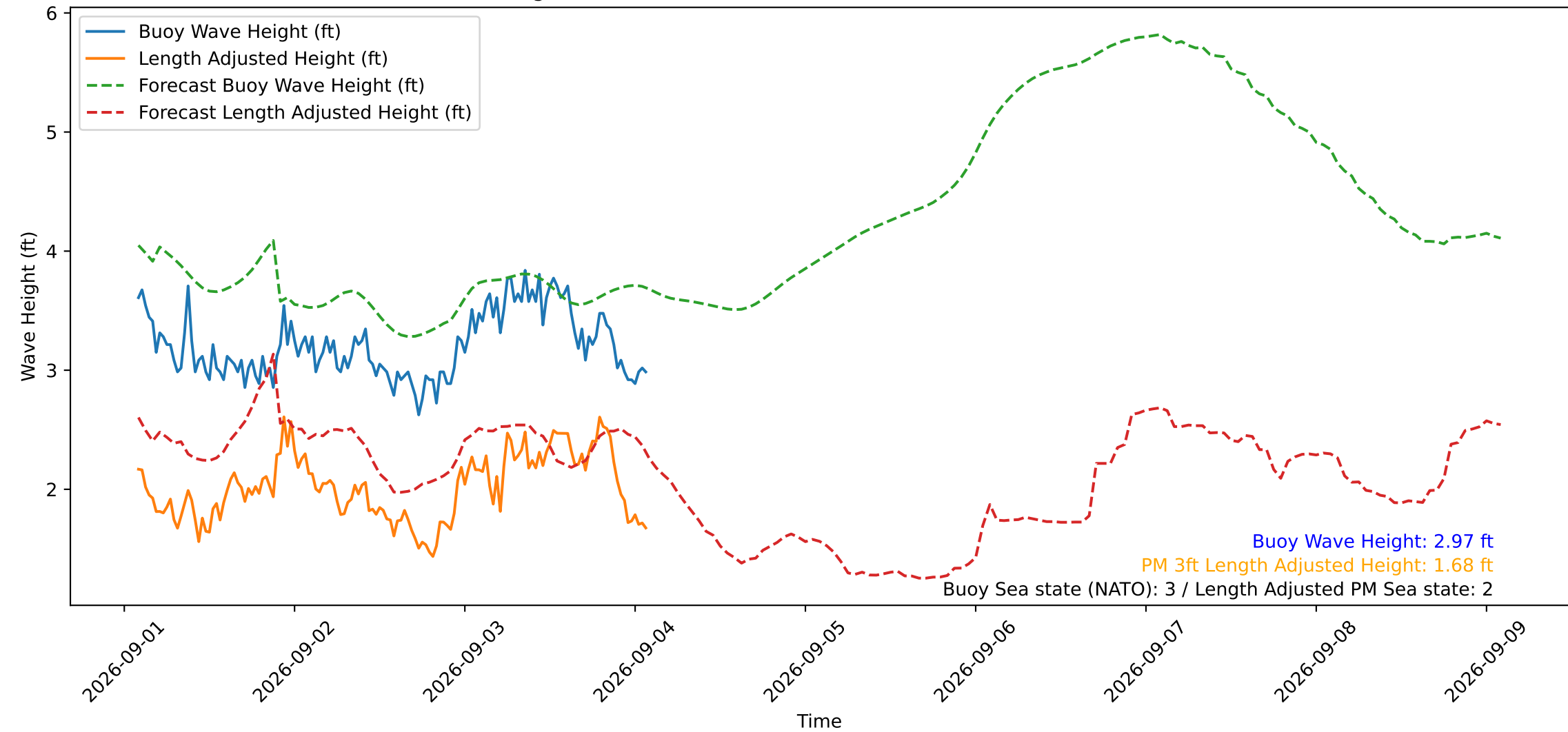
Wave Heights over Time for Oceanside Harbor at 2026-09-04 02:10:30
