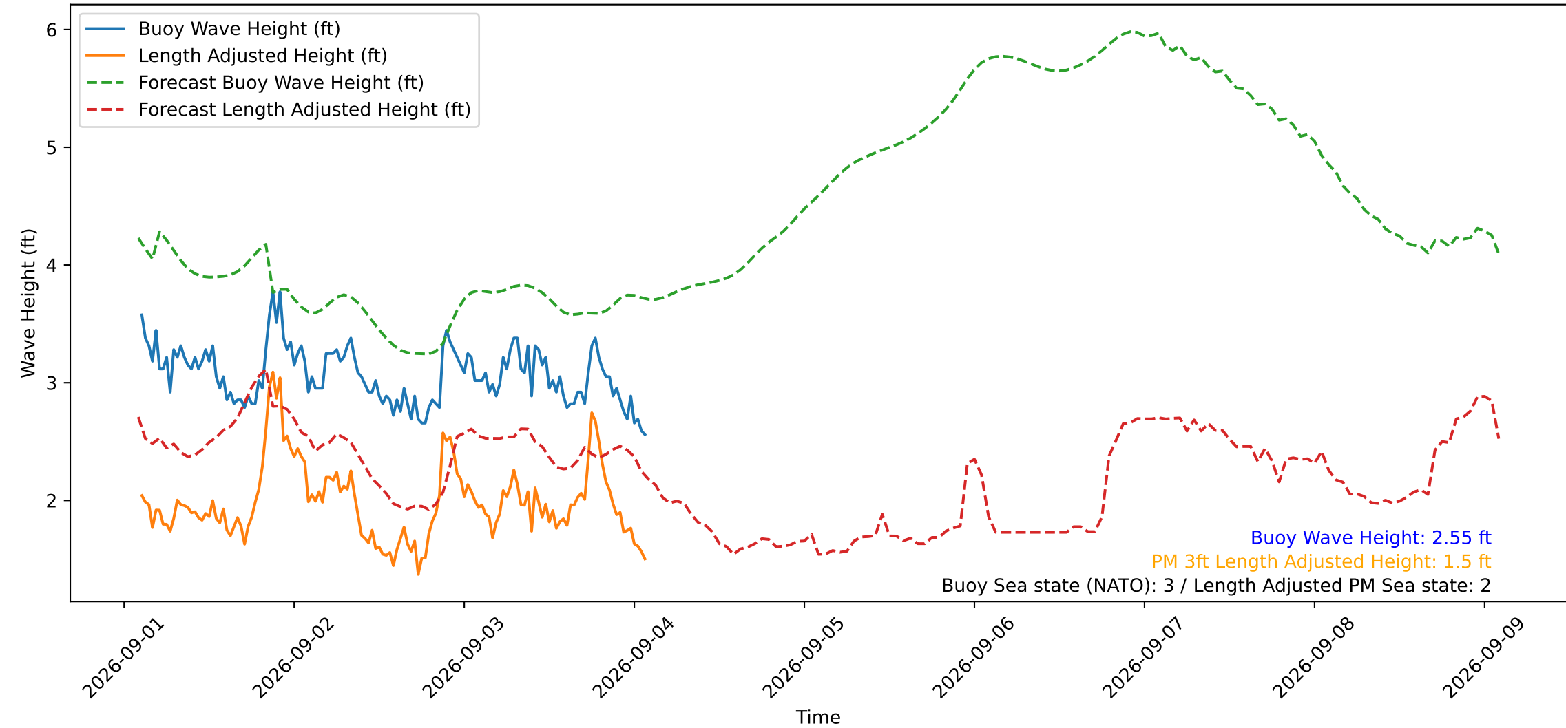
Wave Heights over Time for Green Beach at 2026-09-04 02:11:12
