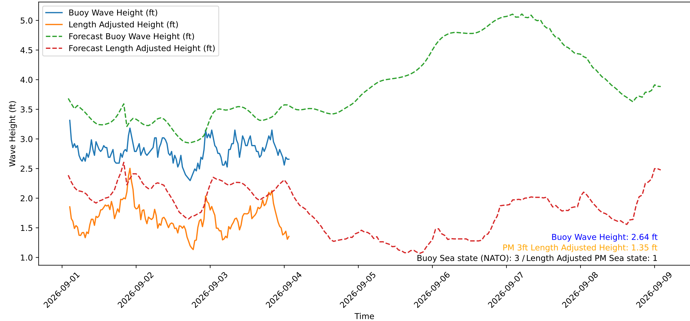
Wave Heights over Time for Red Beach at 2026-09-04 02:10:50
