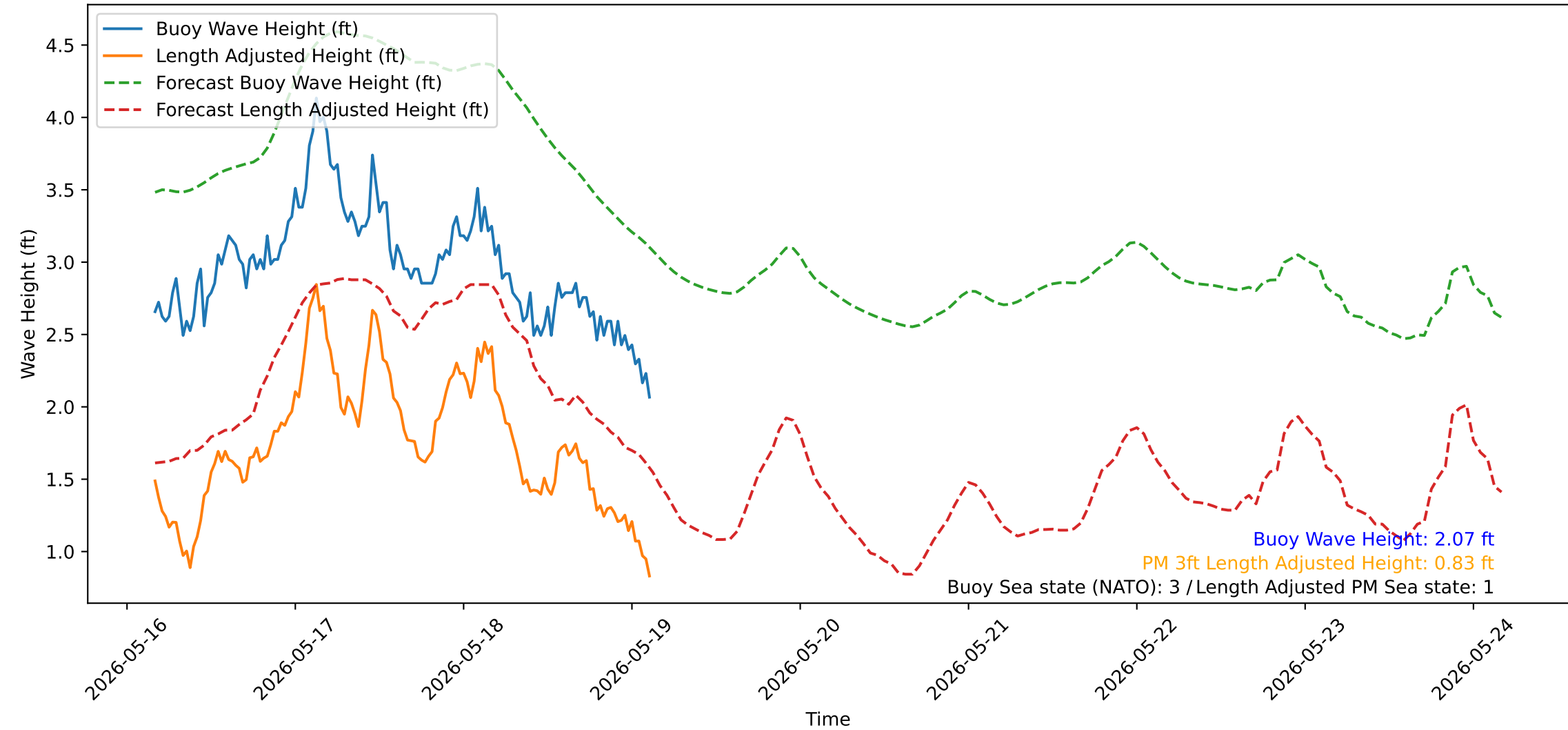
Wave Heights over Time for Red Beach at 2026-05-19 03:30:51
