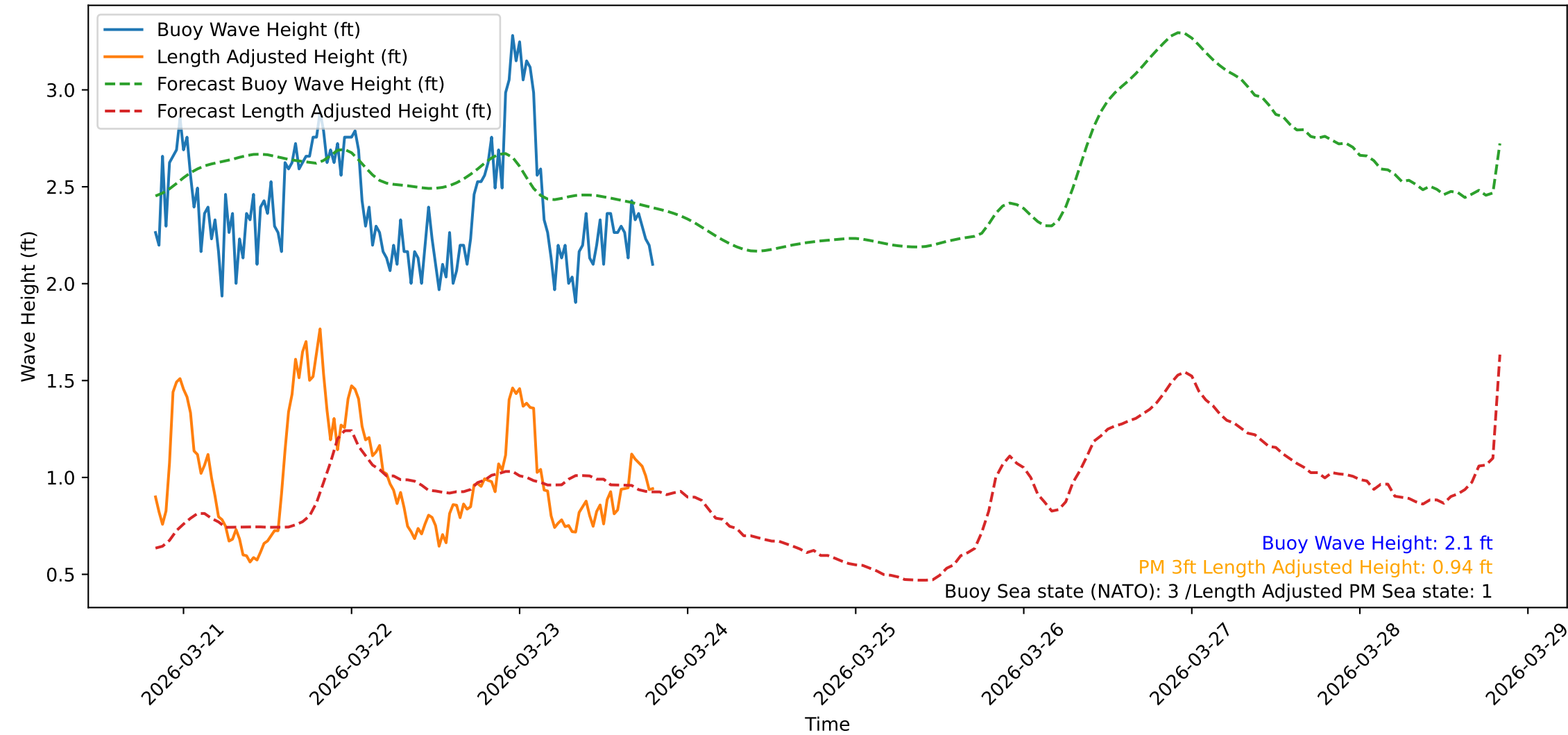
Wave Heights over Time for Green Beach at 2026-03-23 20:01:08
