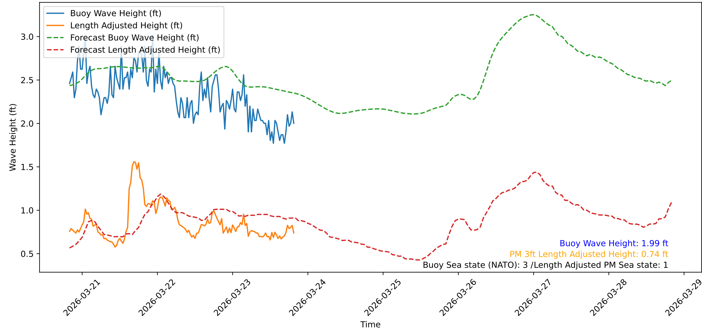
Wave Heights over Time for Oceanside Harbor at 2026-03-23 20:00:31
