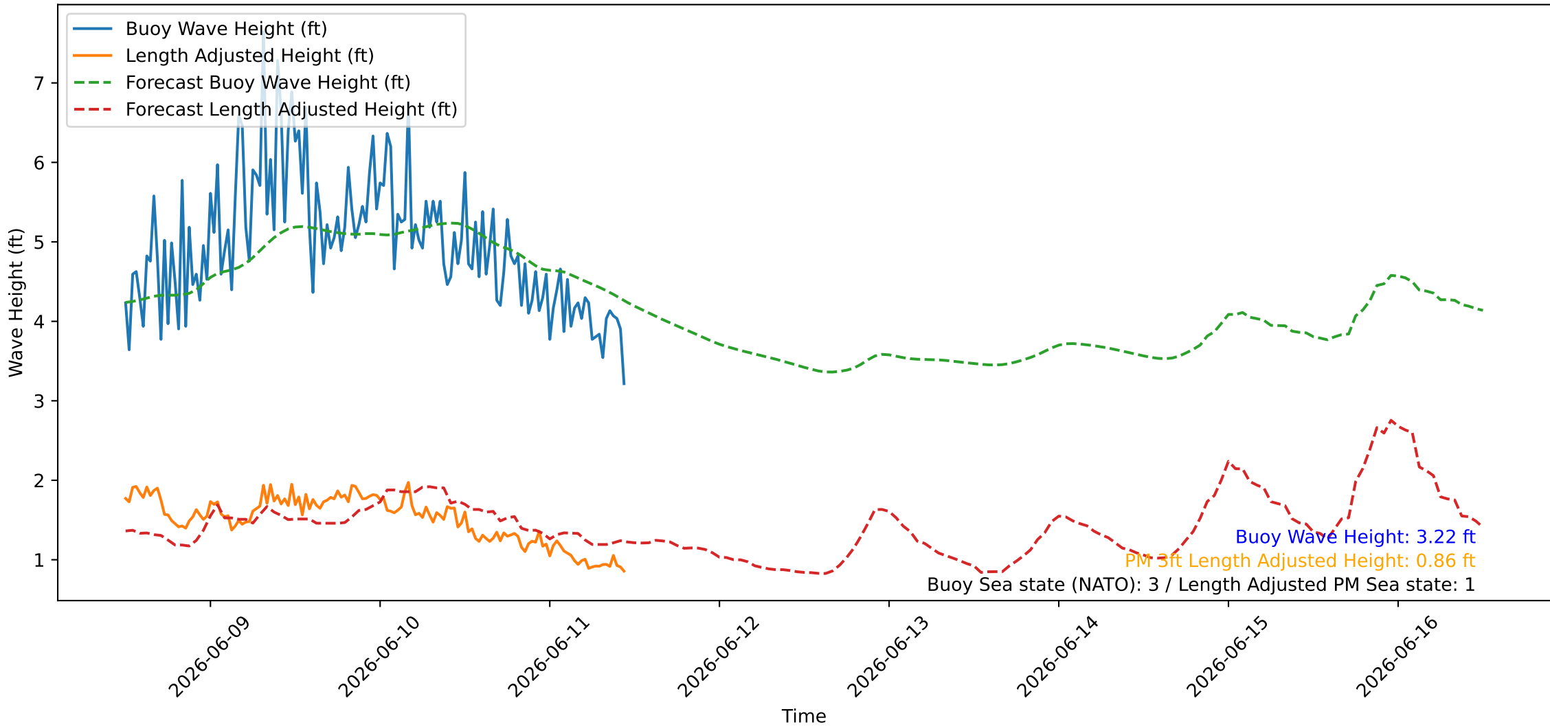
Wave Heights over Time for Red Beach at 2026-06-11 11:30:46
