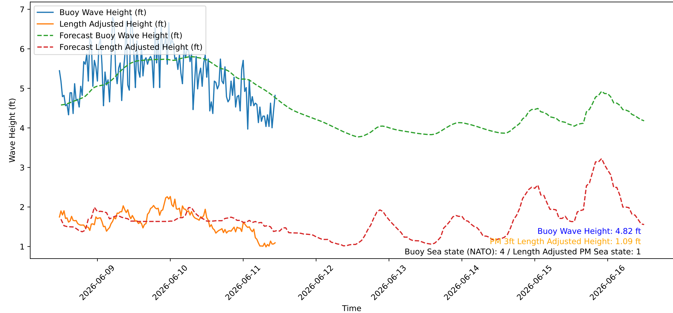
Wave Heights over Time for Green Beach at 2026-06-11 11:31:09
