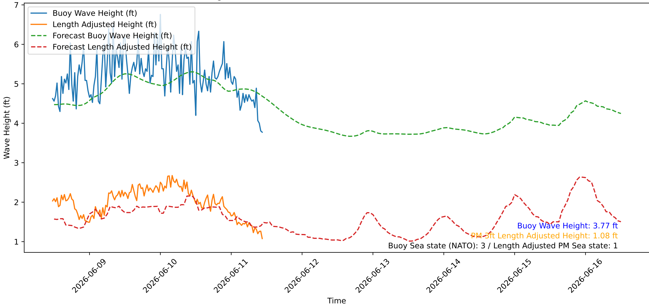
Wave Heights over Time for Oceanside Harbor at 2026-06-11 11:30:26
