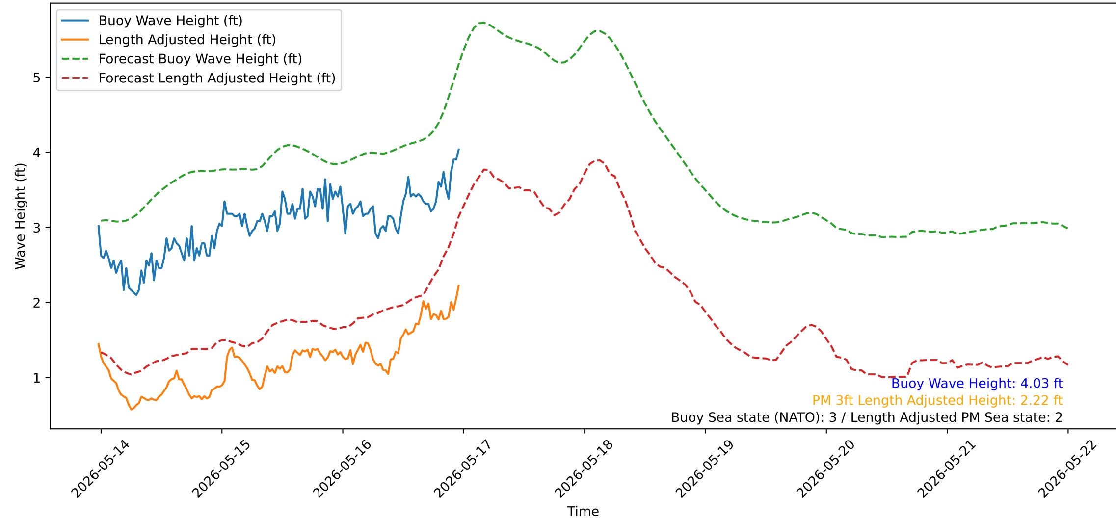
Wave Heights over Time for Green Beach at 2026-05-16 23:41:14
