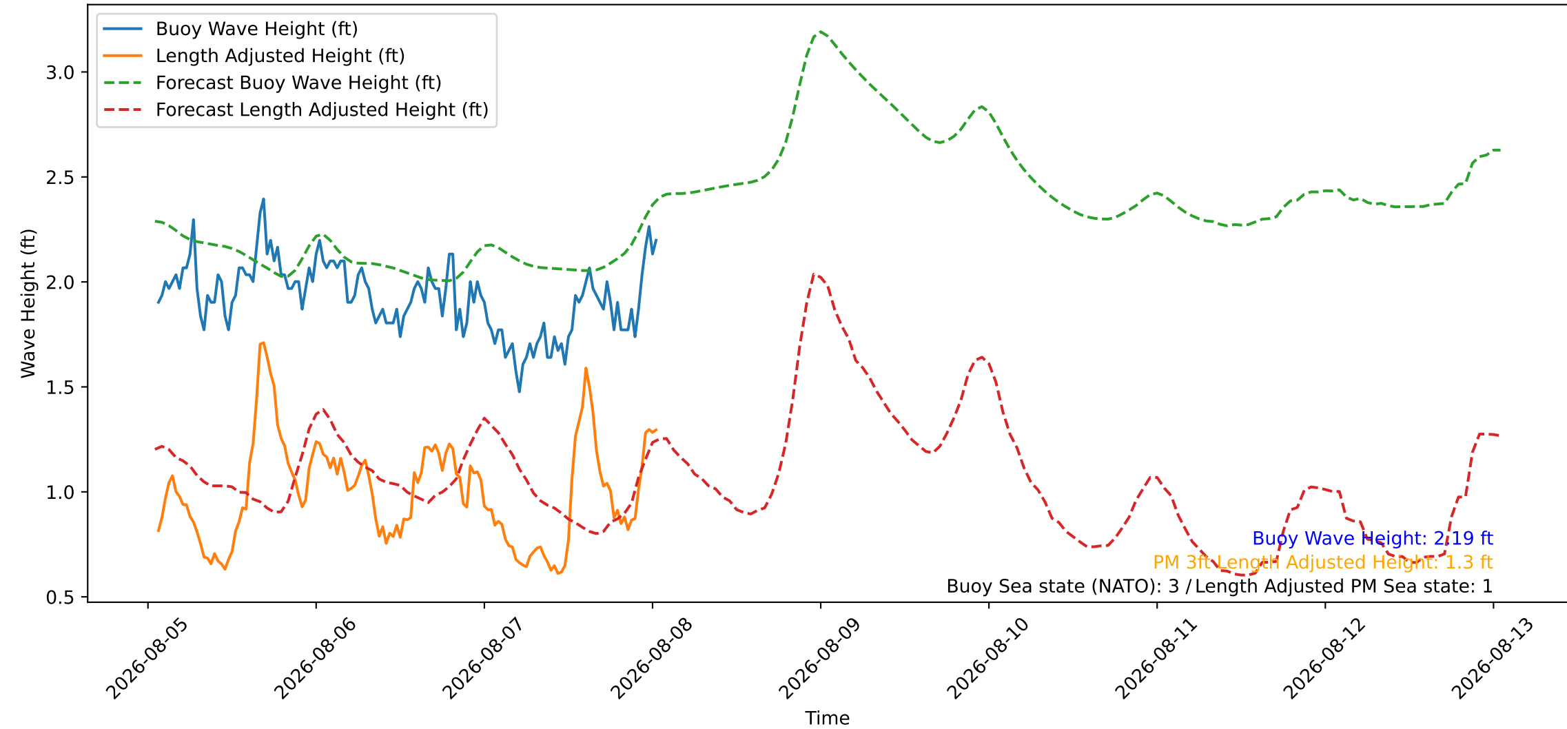
Wave Heights over Time for Red Beach at 2026-08-08 01:20:47
