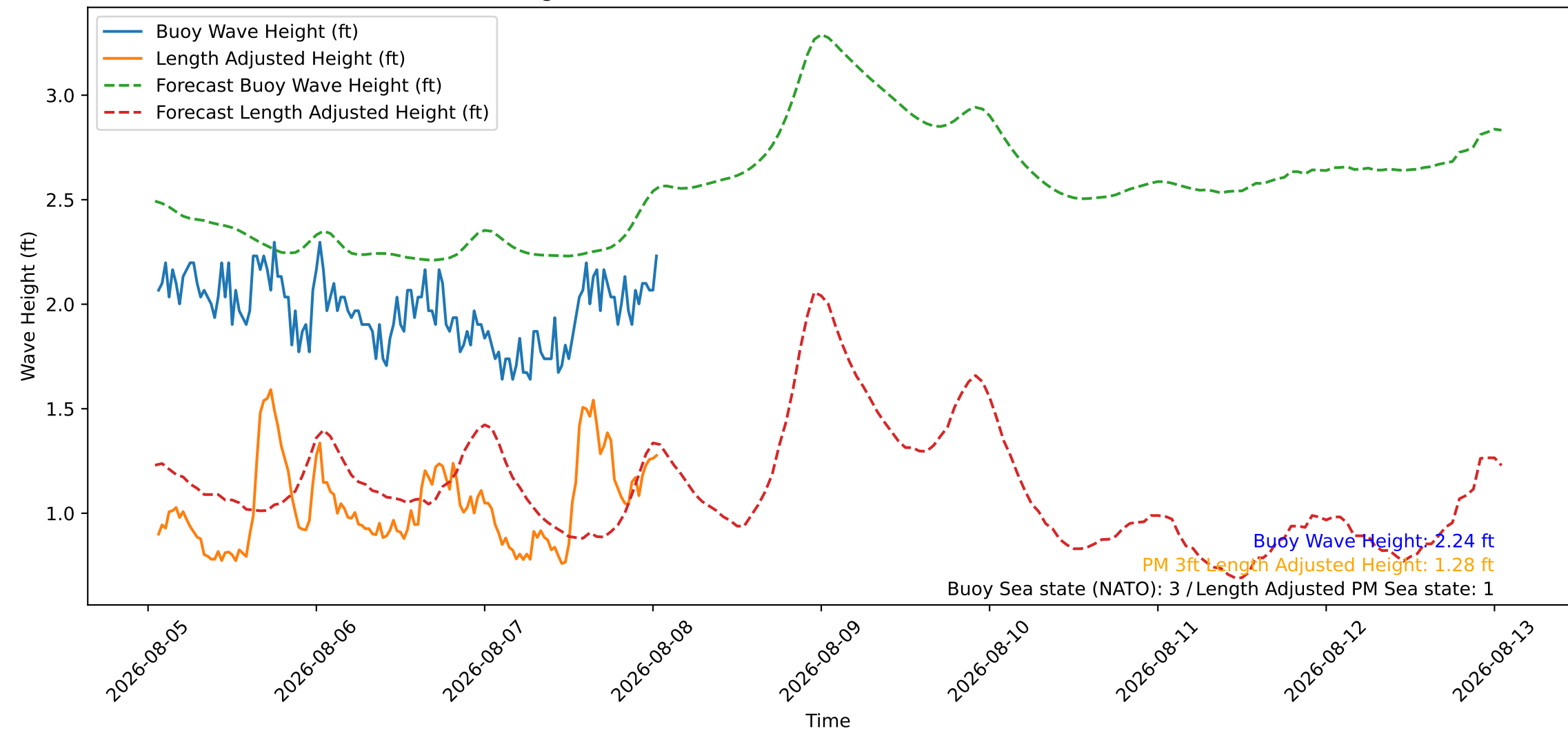
Wave Heights over Time for Oceanside Harbor at 2026-08-08 01:20:26
