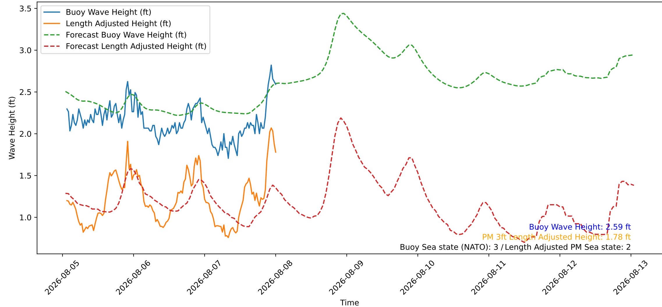
Wave Heights over Time for Green Beach at 2026-08-08 01:21:09
