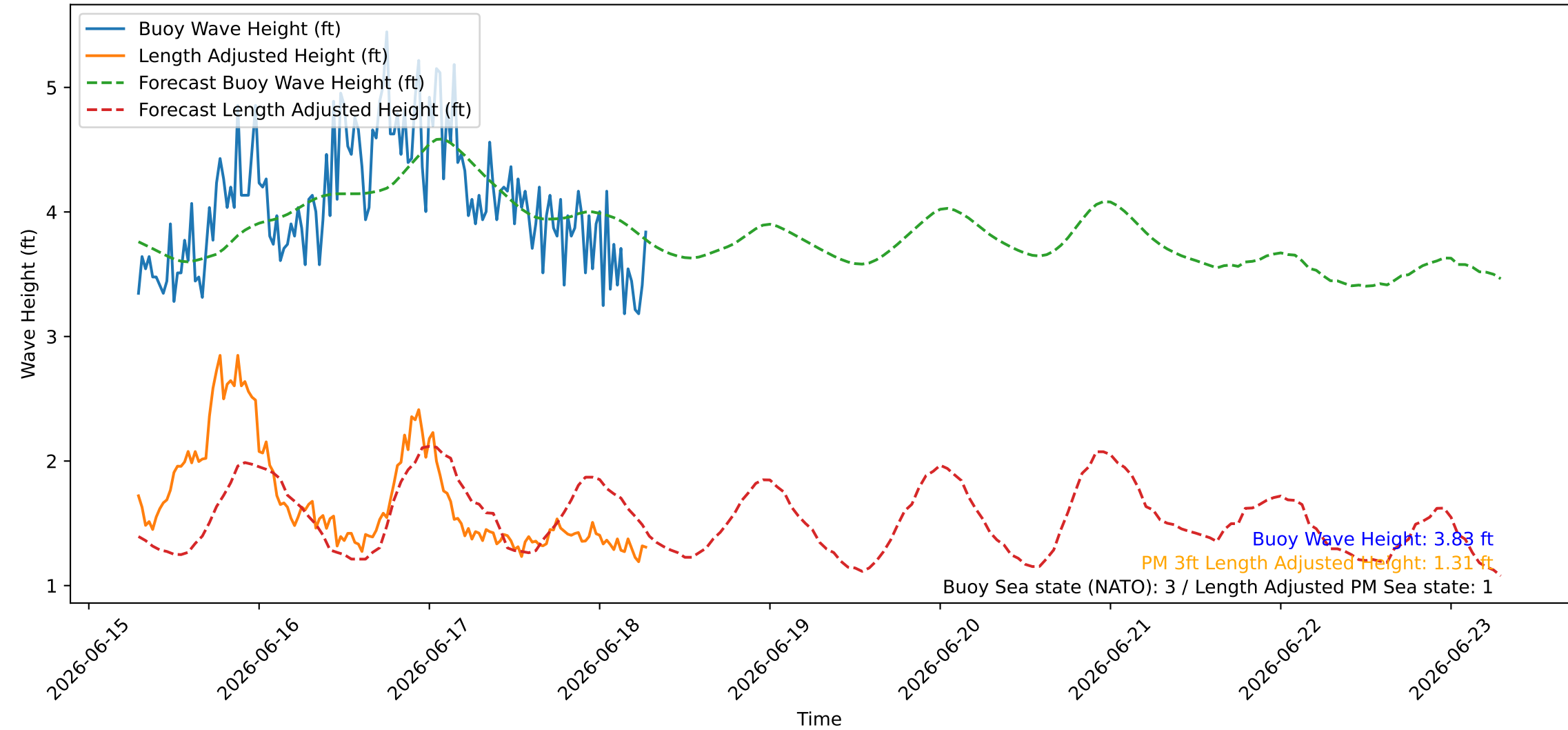
Wave Heights over Time for Oceanside Harbor at 2026-06-18 07:10:26
