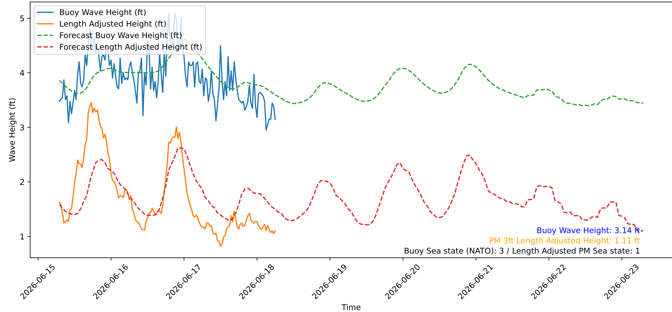
Wave Heights over Time for Green Beach at 2026-06-18 07:11:08
