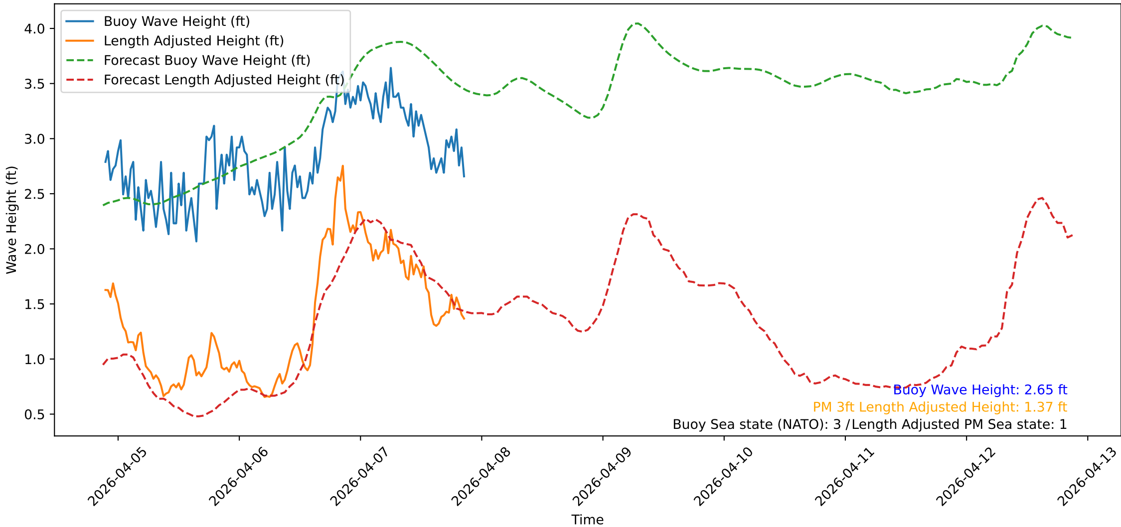
Wave Heights over Time for Oceanside Harbor at 2026-04-07 21:20:31
