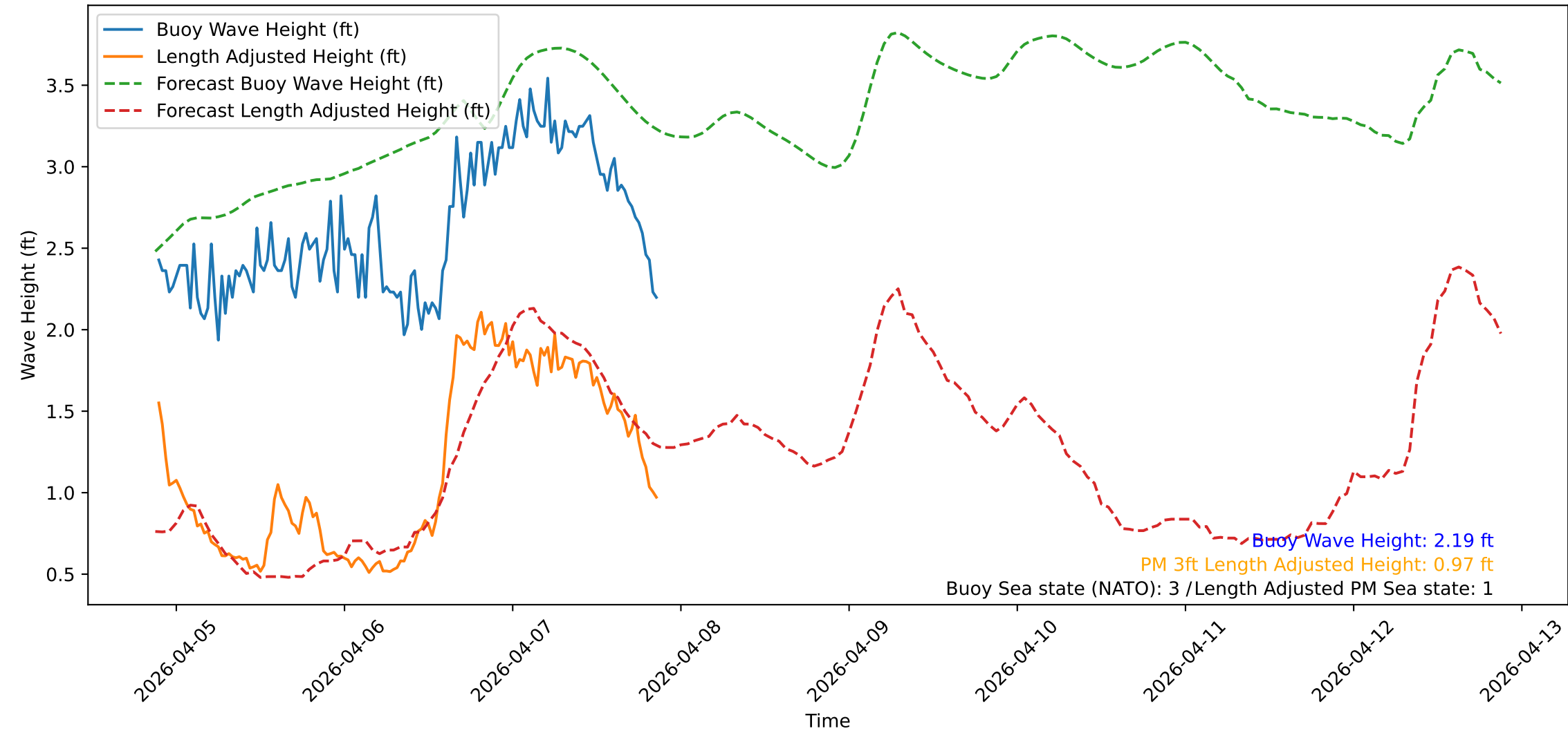
Wave Heights over Time for Red Beach at 2026-04-07 21:20:46
