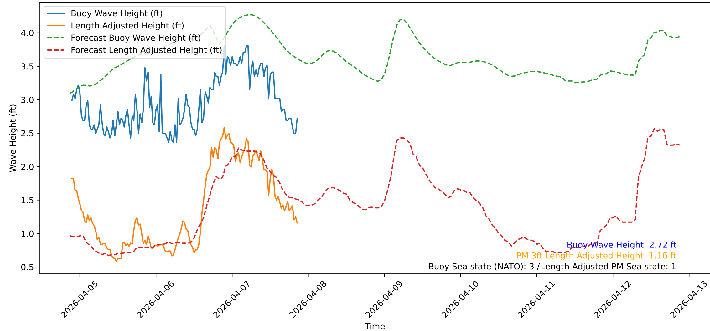
Wave Heights over Time for Green Beach at 2026-04-07 21:21:08
