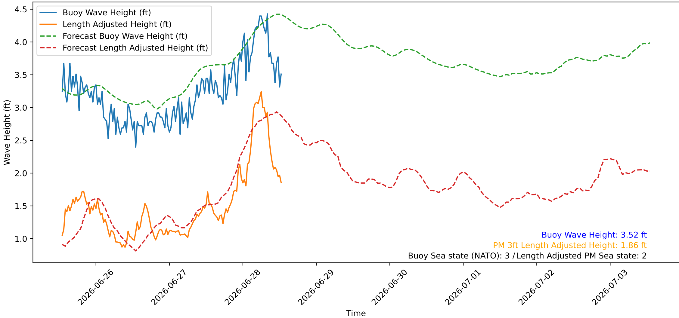
Wave Heights over Time for Oceanside Harbor at 2026-06-28 13:10:26
