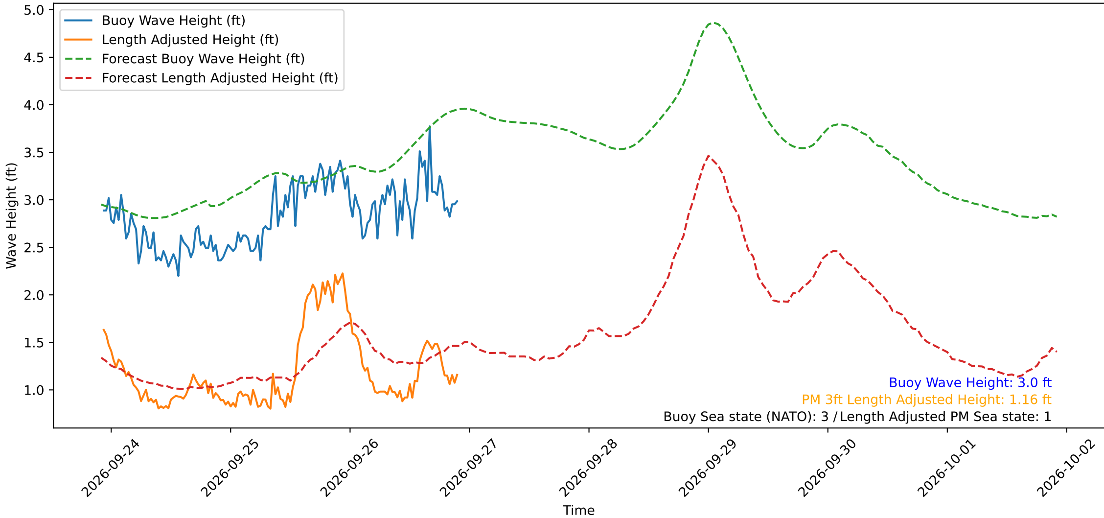
Wave Heights over Time for Oceanside Harbor at 2026-09-26 22:20:30
