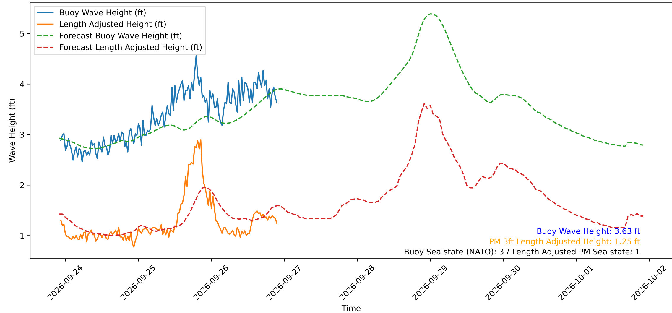
Wave Heights over Time for Green Beach at 2026-09-26 22:21:15
