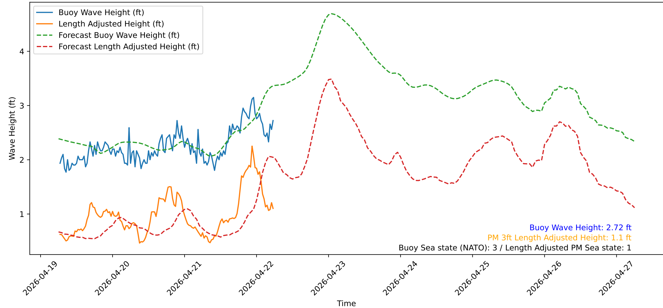
Wave Heights over Time for Red Beach at 2026-04-22 06:20:51
