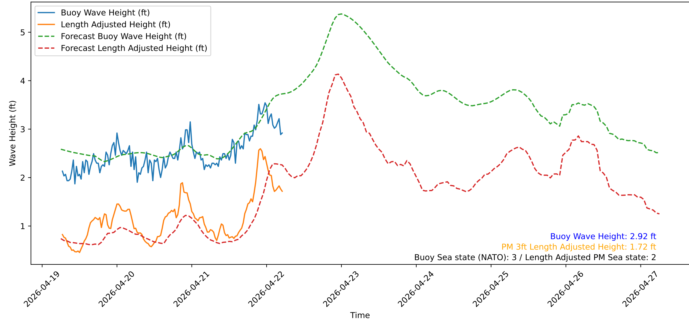
Wave Heights over Time for Green Beach at 2026-04-22 06:21:14
