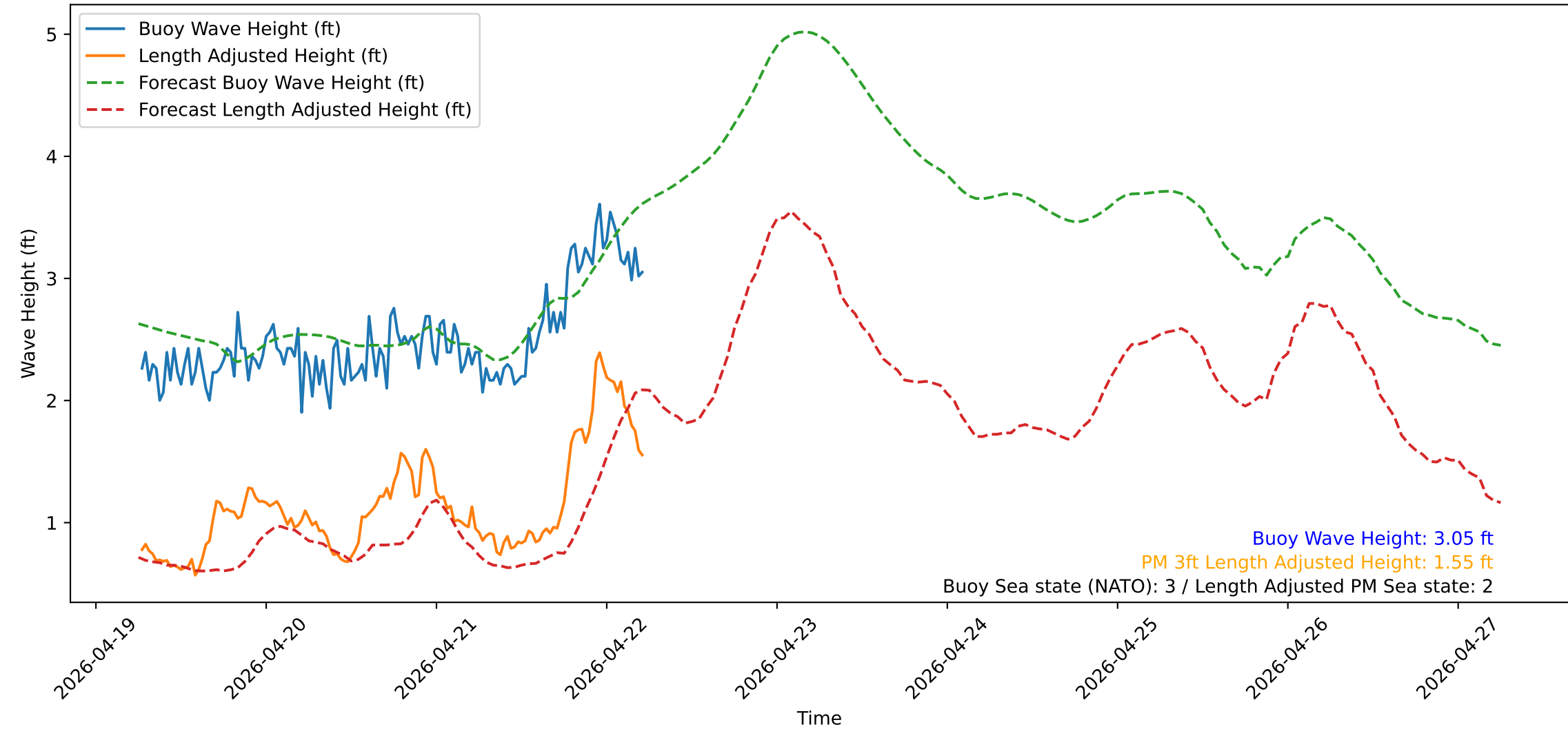
Wave Heights over Time for Oceanside Harbor at 2026-04-22 06:20:31
