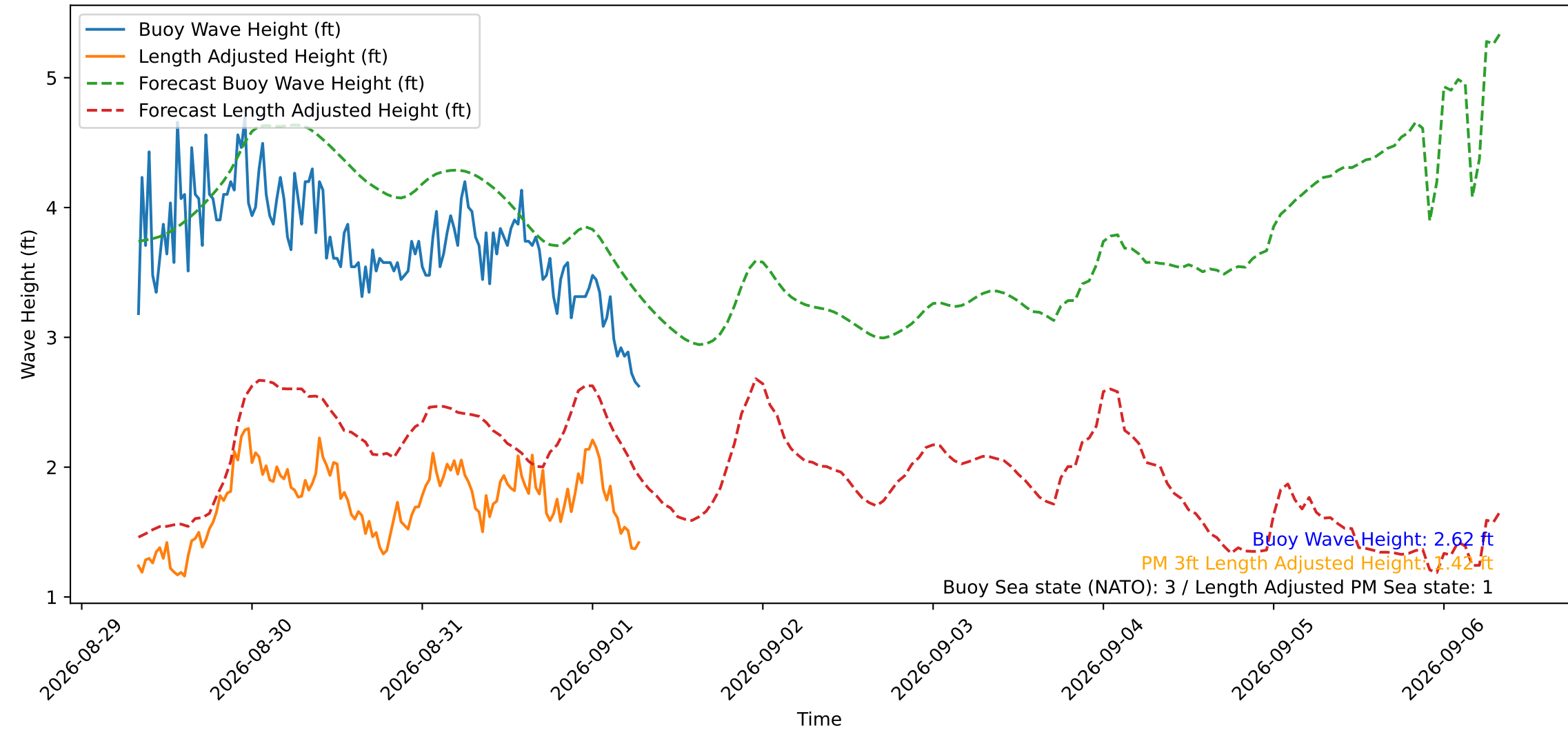
Wave Heights over Time for Red Beach at 2026-09-01 07:30:50
