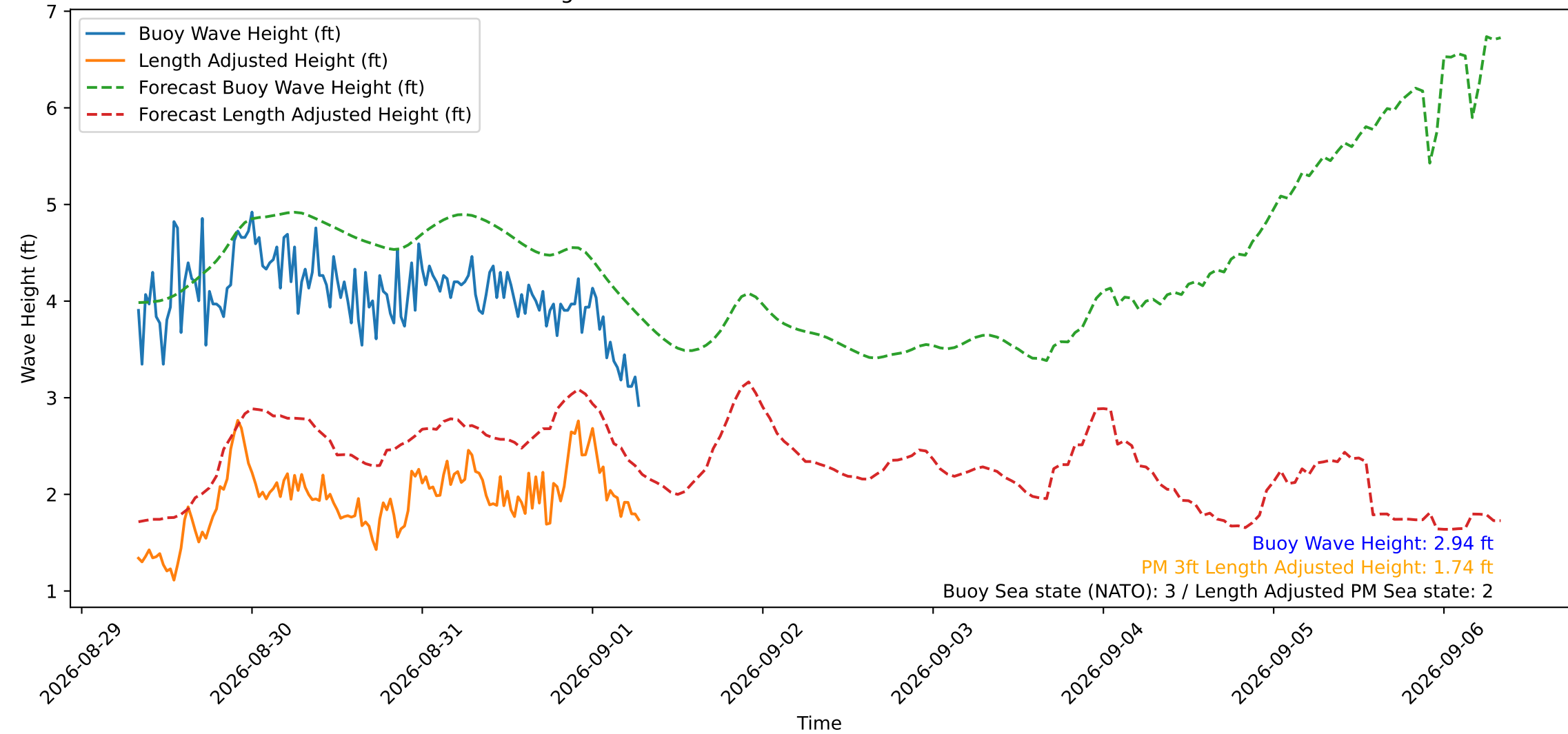
Wave Heights over Time for Green Beach at 2026-09-01 07:31:12
