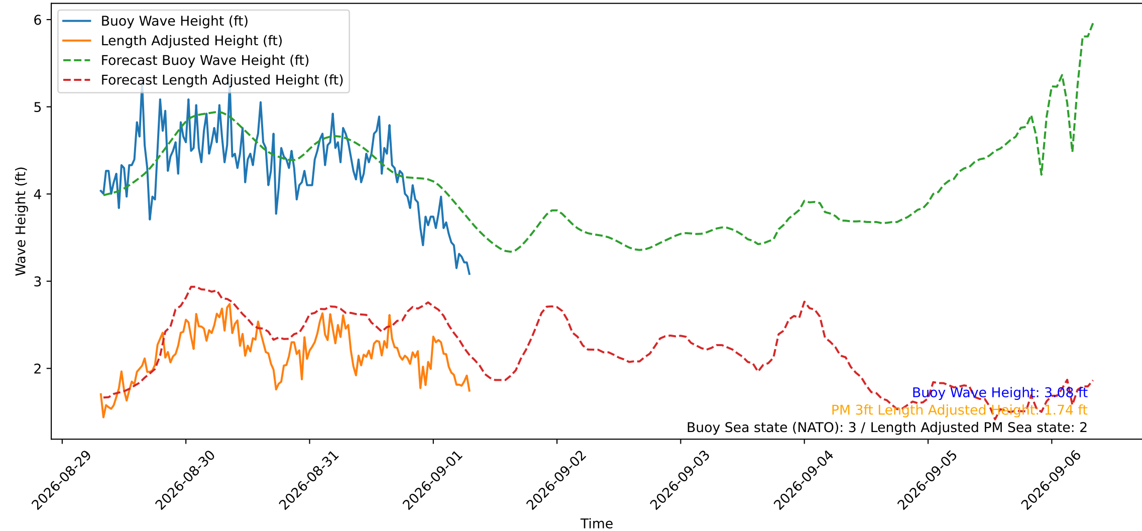
Wave Heights over Time for Oceanside Harbor at 2026-09-01 07:30:30
